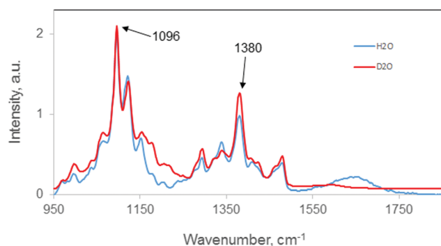
Fig. 11 Raman spectra of CNCs in H 2 O vs. D 2 O (after fully exchanging replaceable OHs with ODs). In the spectrum obtained in D 2 O, the increase in intensity at 1380 cm -1 can be noted.
