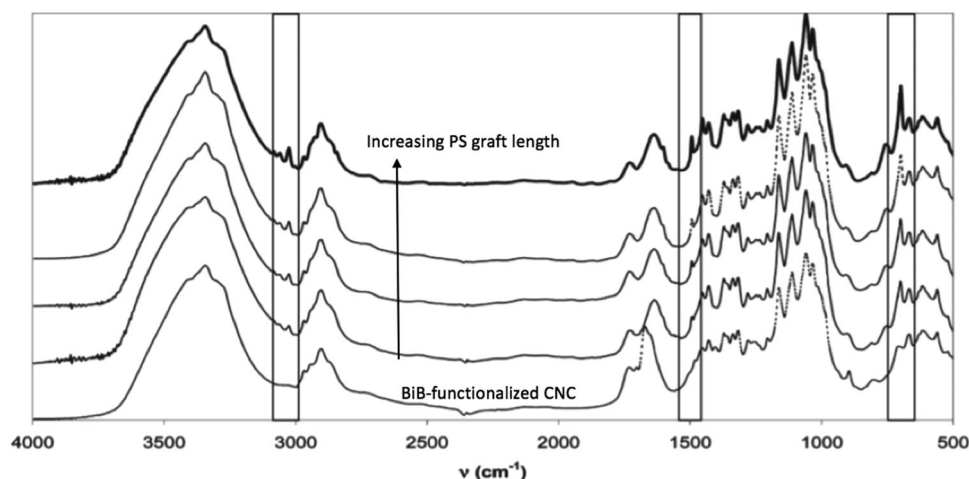
Fig. 13 Full FTIR spectra of BiB-functionalized CNCs and PS-grafted CNCs. Reprinted with permission from reference. Reproduced from ref. 175 with permission from Elsevier, copyright 2015.
