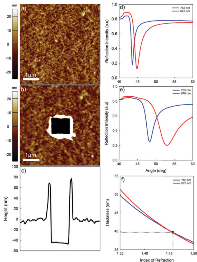
Fig. 31 AFM height image of (a) a dry CNC film, (b) scratched CNC film, and (c) cross section height analysis of scratched image used to determine film thickness. MP-SPR spectrum of (d) bare SiO 2 substrate and (e) dry CNC film. Wavelength crossover (f) displays an index of refraction of 1.4578 and a thickness of 39.7 nm. Reprinted from ref. 56 with permission from the Royal Society of Chemistry.
