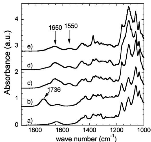
Fig. 14 A snippet of FTIR spectra of sulfated (a), oxidized (b), Jeffamine polyetheramine M1000-grafted (c), Jeffamine polyetheramine M2070-grafted (d), and Jeffamine polyetheramine M2005-grafted (e) CNCs. Reprinted with permission from ref. 256.
