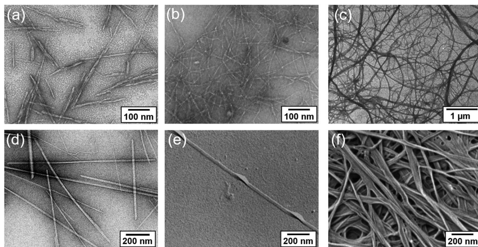
Fig. 1 Electron micrographs of several CNM types, (a) transmission electron microscopy (TEM) image of CNCs, 16 (b) TEM image of CNF with fibrillation pretreatment to impart surface charge, 17 (c) TEM image of CNF without fibrillation pretreatments, 18 (d) TEM image of t-CNCs (image courtesy of Yu Ogawa, CERMAV), (e) TEM of AC, 19 (f) scanning electron microscopy (SEM) image of BC. 20 Reprinted with permission, (a) from ref. 16 TAPPI Press, (b) from ref. 17 TAPPI Press, (c) from ref. 18 © 1997 John Wiley & Sons, (e) from ref. 19 © 1997 Springer Science + Business Media B.V., (f) from ref. 20 © 2007 American Chemical Society.
