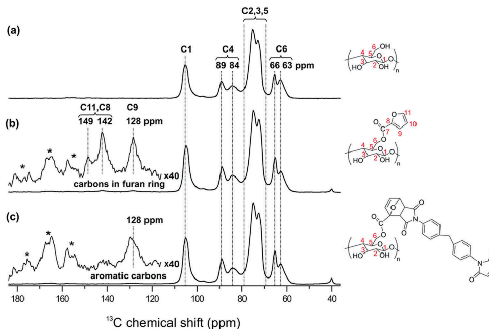
Fig. 17 ssNMR characterization of surface-modified CNFs: CPMAS ^{13}\text{C} NMR spectra of (a) unmodified CNF, (b) furoate CNF and (c) maleimide-modified CNF. The corresponding molecular structures of the CNF and the surface modified CNF are shown in the right panel. The insets in (b) and (c) display zooms over the spectral region 116–184 ppm, with some identified signals from the substituents indicated. Spinning sidebands are marked by asterisks. Reproduced from ref. 266 with permission from ACS Publications, copyright 2015.
