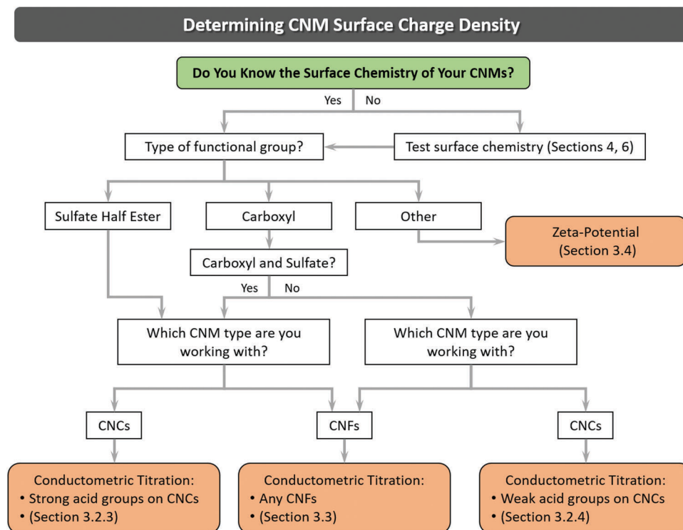
Fig. 5 Decision tree for the determination of surface charge density for different CNMs and functionalizations.
