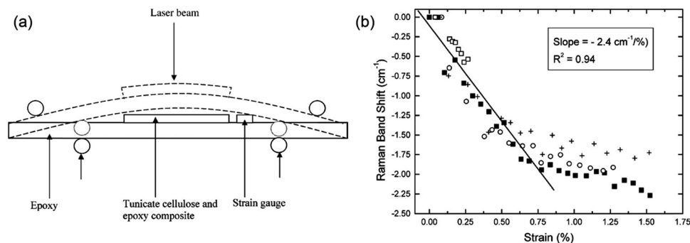
Fig. 39 (a) Schematic of the 4-point bending test used to deform epoxy/tunicate composite samples under a Raman microscope; (b) shifts in the position of the Raman band initially located at \sim 1095\text{ cm}^{-1} from tunicate CNCs embedded in epoxy resin and deformed under 4-point bending in tension. Reprinted from ref. 442. Reproduced with permission from the American Chemical Society.
