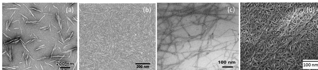
Fig. 18 Images of what to expect from SEM and TEM of CNMs, (a) TEM of negatively stained CNCs (a). Reprinted with permission from ref. 251, copyright 2010 American Chemical Society. (b) SEM of cast CNC film. Unpublished images courtesy of Foster, Roberts and Stinson-Bagby. (c) TEM of negatively stained TEMPO-oxidized CNFs Reprinted with permission from ref. 277, copyright 2007 American Chemical Society and (d) SEM of untreated CNFs. Reprinted from ref. 278, copyright 2015, with permission from Elsevier.
