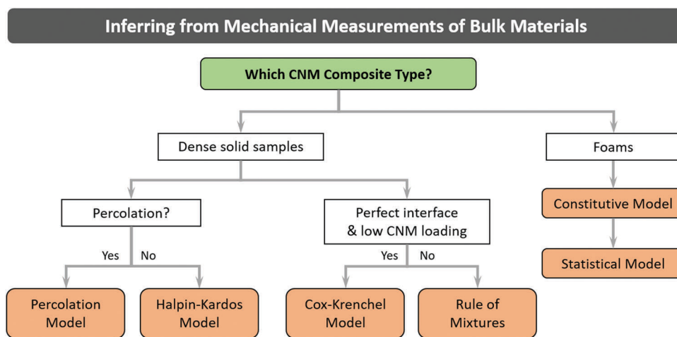
Fig. 38 Decision tree showing the models available for inferring the mechanical measurement of bulk materials.
