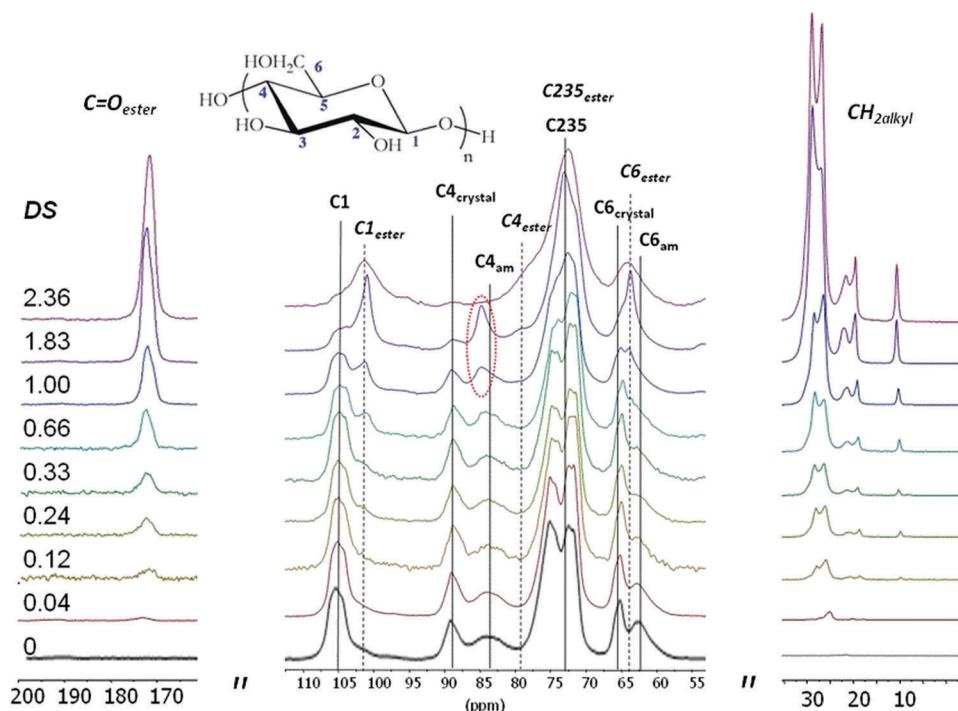
Fig. 16 ssNMR spectra of CNF aerogels modified with palmitoyl acyl chloride vapours, with DS ranging from 0 to 2.36. Reproduced from ref. 259 with permission from ACS Publications, copyright 2013.
