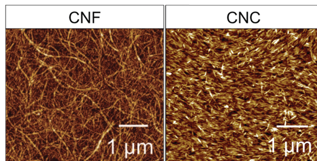
Fig. 30 AFM height images of spin coated CNF (left) and CNC (right) films showing different film topography and porosity. CNF films were prepared from 0.4\ \text{g L}^{-1} suspension on 3-aminopropyl-trimethoxysilane coated \text{SiO}_2 QCM-D sensors. Reproduced from ref. 242 with permission from the American Chemical Society, copyright 2008. CNC films were prepared from 3 wt% suspension spin coated on \text{SiO}_2 coated SPR sensors.
