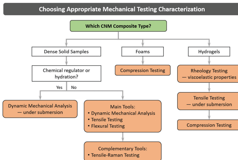
Fig. 35 Decision tree showing the best options for characterization of the mechanical properties of CNM composites.
