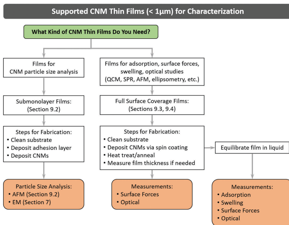
Fig. 28 A decision tree pertaining to supported CNM thin films (<1 µm thick) used for various subsequent characterization techniques.
