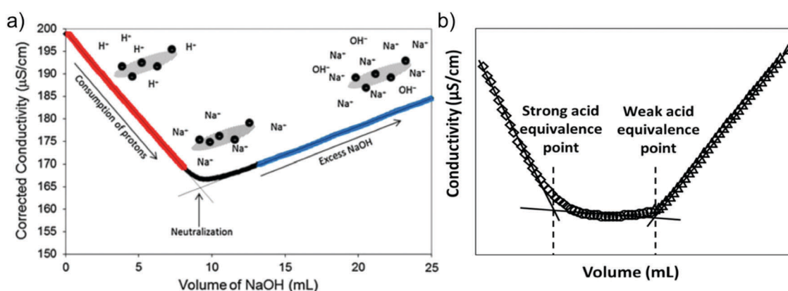
Fig. 6 (a) Conductometric titration curve of S-CNCs from cotton (0.06 g cellulose) titrated against NaOH (1.31 mM) where the intersection of the two slopes (neutralization point) corresponds to the amount of strong acid (sulfate half ester groups) on the CNC surface. Figure reprinted with permission from reference. Reprinted by permission from Springer Nature: Springer Nature Cellulose "Estimation of the surface sulfur content of cellulose nanocrystals prepared by sulfuric acid hydrolysis", Tiffany Abitbol, Elisabeth Kloser, Derek G. Gray, © (2013). (b) \text{COOH} -CNCs in acidic media titrated with NaOH. An initial step associated with the deprotonation of the free acid is followed by the deprotonation of the carboxyl groups and further with an increase of the conductivity associated with the excess NaOH. The linear fit (utilizing the highest coefficient of determination, " R^2 " for all three lines) and two intersection points for determining the strong and weak acid equivalence points are annotated and the total carboxyl content is calculated from the volume difference of NaOH added between the equivalence points. Experimental data kindly provided by Dr S. Camarero-Espinosa.
