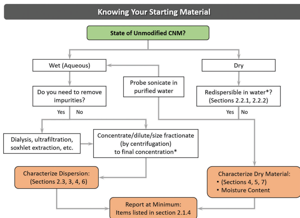
Fig. 3 A decision tree for how to start characterizing your starting CNMs. * Upper limit to suspension concentration dependent upon the type of CNM – ( e.g. , CNC, CNF, charge density, counterions and additives).
