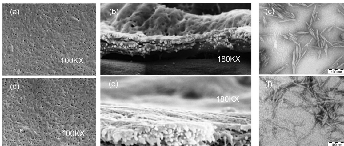
Fig. 25 EM micrographs of the cross-section of CNC containing films where (a–c) (top images) contain sulfuric acid ( \text{H}_2\text{SO}_4 ) treated CNCs, and (d–f) (bottom images) contain APS treated CNCs. Images (a and d) are surface topography SEM images of the two films. Images (b and e) are images showing cross sections of the films. Finally, images (c and f) are TEM images of the CNCs after treatments with \text{H}_2\text{SO}_4 and APS respectively. Reprinted by permission from Springer Nature: Springer Nature, Cellulose “Comparison of cellulose nanocrystals obtained by sulfuric acid hydrolysis and ammonium persulfate, to be used as coating on flexible food-packaging materials”, E. Mascheroni, R. Rampazzo, M. A. Ortenzi et al. , © 2016.
