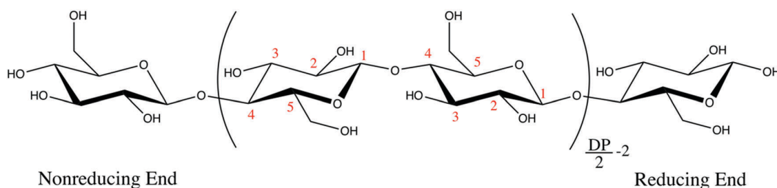
Fig. 10 Chemical structure of cellulose and carbon atom numbering (C1–C5) of the glucose ring.
