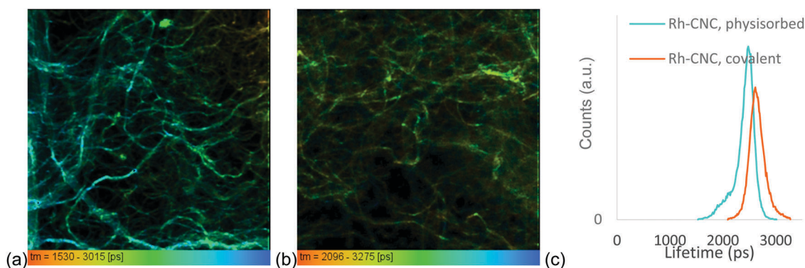
Fig. 34 Fluorescence lifetime image of rhodamine 110 labeled CNCs. (a) Physisorbed and (b) covalently bound with free dye removed using tangential flow filtration. (c) The lifetime distributions narrow to a single peak and shift towards higher lifetimes when the dye is bound. Unpublished data.
