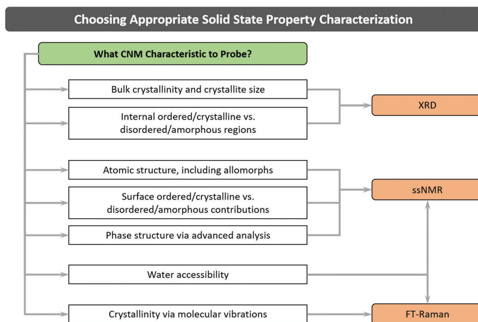
Fig. 8 Decision tree for the three primary techniques used to analyze the solid-state structure of CNMs. These techniques are complementary to each other, and collectively will provide as comprehensive a picture as possible of the CNM solid-state structure. More detailed insights into the topic can be found in Hamad. 193
