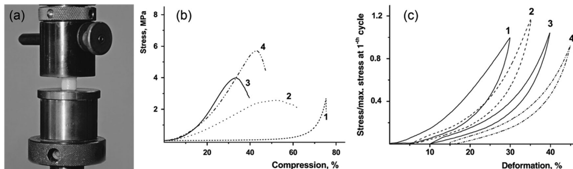
Fig. 36 (a) Photograph of a typical unconfined compression test of BC-PAAm hydrogel (b) stress-strain curves in compression of a series of hydrogels with different BC concentrations: 0 (1), 4.0 (2), 8.0 (3) and 14 (4) wt%, and (c) cyclic compression-unloading curves of BC-PAAm hydrogel samples 1: 1st cycle; 2: 2000th cycle; 3: 4000th cycle; 4: 6000th. Reprinted from ref. 426. Reproduced with permission from Elsevier.
