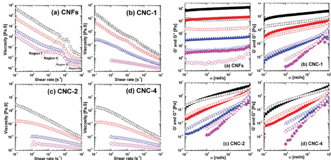
Fig. 27 (left) Steady-state viscosity versus shear rate, (right) SAOS results illustrating shear storage modulus G' (solid symbols) and loss modulus G'' (open symbols) as a function of angular frequency of (a) CNFs, (b) CNC-1, (c) CNC-2, (d) CNC-4 suspensions with concentrations of 1.5 wt% (black squares), 1.0 wt% (red circles), 0.5 wt% (blue triangles), and 0.25 wt% (magenta diamonds) at 25 °C. The number after the CNC represents the hydrolysis time of 1 to 4 h. In a low concentration and a low shear rate region, the viscosity could not be measured precisely because of the sensitivity of the rheometer. Reproduced from ref. 285 with permission from the American Chemical Society, copyright 2015.
