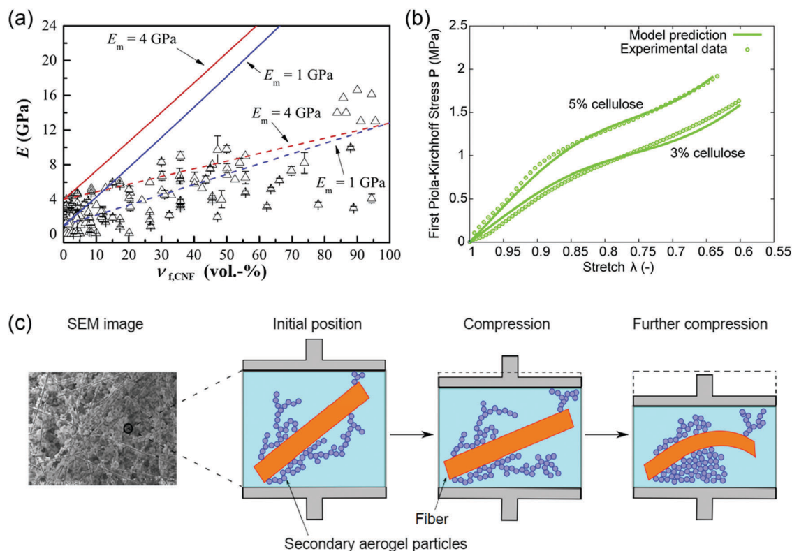
Fig. 37 (a) Theoretical and experimental tensile moduli values of CNF reinforced composites. The hollow icons represent the experimental data and the solid line and dashed line denote the theoretical values obtained using the Cox–Krenchel model and theoretical values obtained using rule-of-mixtures, respectively. This figure is obtained from Lee et al. 435 reproduced under the terms of Creative Commons Attribution License; (b) model predictions of the constitutive response of cellulose aerogels compared with experimental data 439 (reproduced from ref. 439 with permission from The Royal Society of Chemistry). (c) An illustration of the damage behavior in the fiber-aerogel composite foam 438 (reproduced from ref. 438 with permission from John Wiley and Sons).
