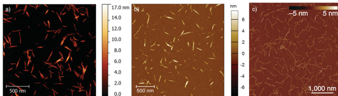
Fig. 29 AFM images for particle size analysis of CNMs. (a) Sulfuric acid hydrolyzed CNCs from bleached softwood kraft pulp deposited by solvent casting on poly-L-lysine coated mica. Reproduced from ref. 95 with permission from L. Johnston and the American Chemical Society, copyright 2016. (b) CNCs produced by CelluForce deposited via spin coating on a poly(allylamine hydrochloride) coated silicon wafer. (c) TEMPO-oxidized CNFs solvent cast onto (3-aminopropyl)triethoxysilane coated mica, adapted from reference. Reproduced from ref. 323 with permission from Nature Communications, copyright 2015.
