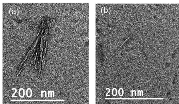
Fig. 21 TEM images of CNCs prepared with (a) negative staining and (b) unstained (both images taken around 100k magnification). Unpublished images courtesy of Foster, Roberts and Stinson-Bagby.
