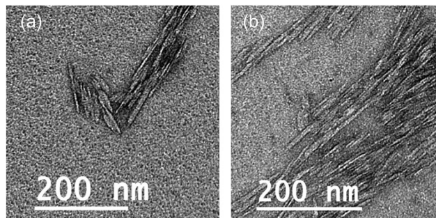
Fig. 20 TEM images of unstained CNCs comparing (a) never-dried CNCs and (b) freeze dried and redispersed CNC. Unpublished images courtesy of Foster, Roberts and Stinson-Bagby.
