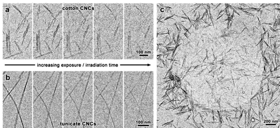
Fig. 22 Damage of the CNMs under TEM as a result of radiation damage on unstained (a) cotton and (b) tunicate. In (c), the CNMs were damaged and shifted as the result of a condensed beam on one spot. Reprinted from ref. 295, under CC BY 3.0 license. Available from: DOI: 10.5772/60985.
