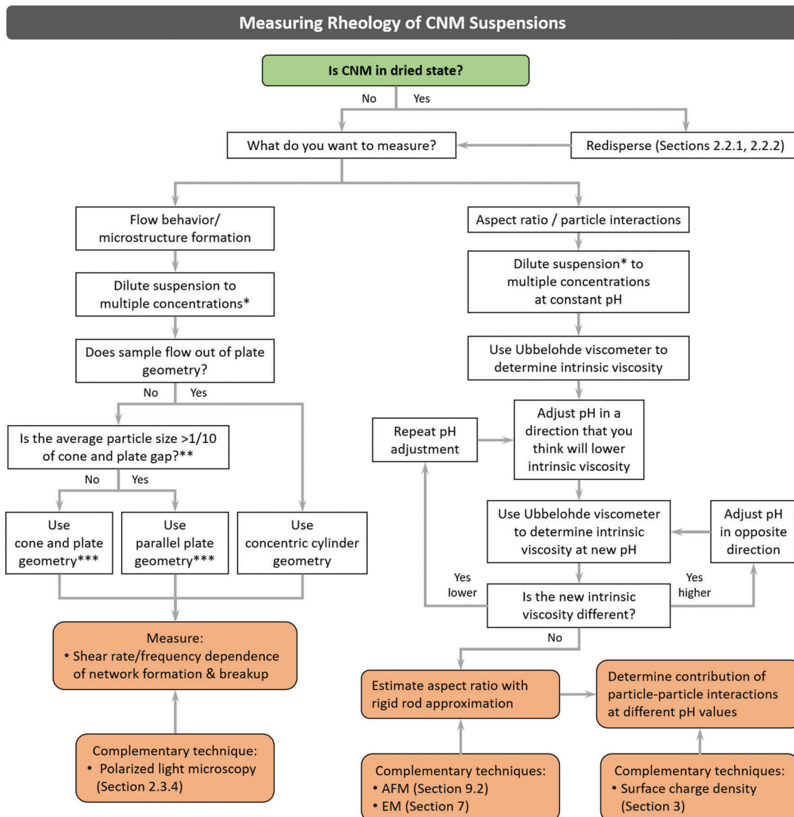
Fig. 26 Decision tree to analyze rheology of CNM suspensions. * Suggested dispersion verification technique in Fig. 3. ** Use solvent trap to prevent sample evaporation. *** Use strain range within LVE region for measurement.
