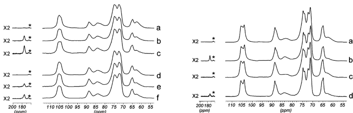
Fig. 15 Left: CP-MAS carbon-13 NMR spectra of microfibrillated sugar beet pulp (SBP): (a) original sample; (b) oxidized SBP (0.75 mol NaClO per mol glycosyl unit); (c) oxidized SBP (2 mol NaClO per mol glycosyl unit); (d) HCl-hydrolyzed; (e) HCl-hydrolyzed and oxidized (0.75 mol NaClO per mol glycosyl unit); (f) HCl-hydrolyzed and oxidized (2 mol NaClO per mol glycosyl unit). The spectral region corresponding to the C=O signals (175–200 ppm) has been multiplied by a factor 2. Asterisks (*) indicate residual spinning sidebands from the C1 signal. Right CP-MAS Carbon-13 NMR spectra of cotton linters: (a) original sample; (b) oxidized (2 mol NaClO per mol glycosyl unit); (c) HCl-hydrolyzed; and (d) HCl-hydrolyzed and oxidized (2 mol NaClO per mol glycosyl unit). The spectral region corresponding to the C=O signals (175–200 ppm) has been multiplied by a factor 2. Asterisks (*) indicate residual spinning sidebands from the C1 signal. Reproduced from ref. 219 with permission from ACS Publications, copyright 2013.
