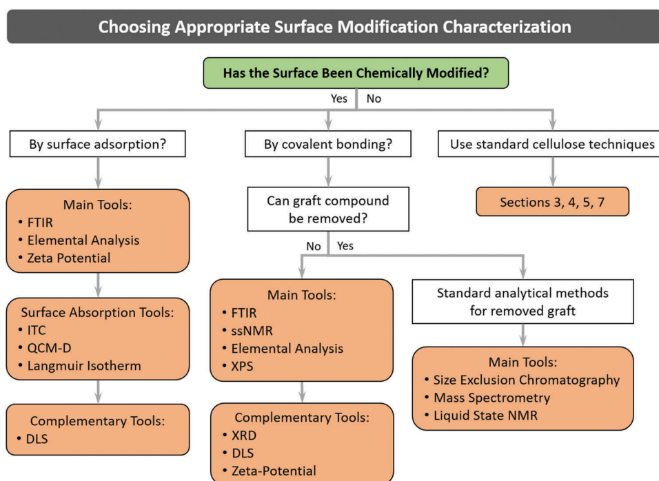
Fig. 12 Decision tree showing a proposed approach for the characterization of chemical modification to CNM surfaces.
