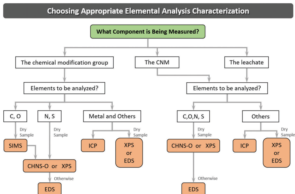
Fig. 7 A decision tree for elemental analysis characterization of the chemical modification group, the CNM or the leachate.
