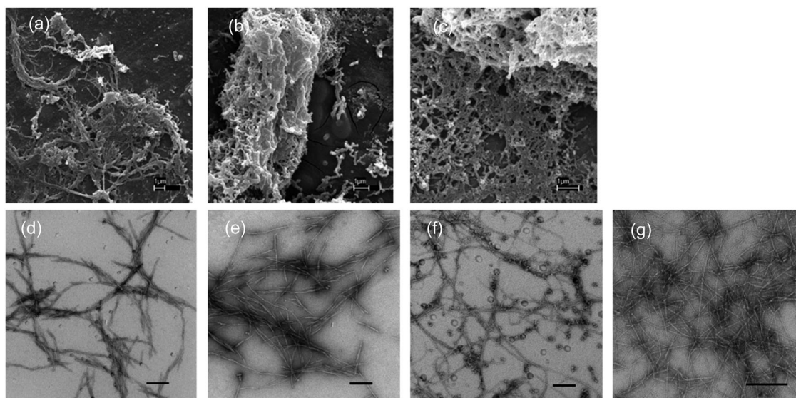
Fig. 24 EM images of eucalyptus CNFs refined with different enzymatic and mechanical treatments; SEM images (a–c) have scale bars of 1 micron; TEM images (d–g) have scale bars of 200 nm; (a and d) enzyme pretreated, refined with a SuperMassCollider; (b and e) enzyme pretreated, refined with a microfluidizer; (c and f) no pretreatment, refined with a microfluidizer; (g) pretreated with TEMPO oxidation, no refinement. Reprinted from ref. 228, copyright 2013, with permission from Elsevier.
