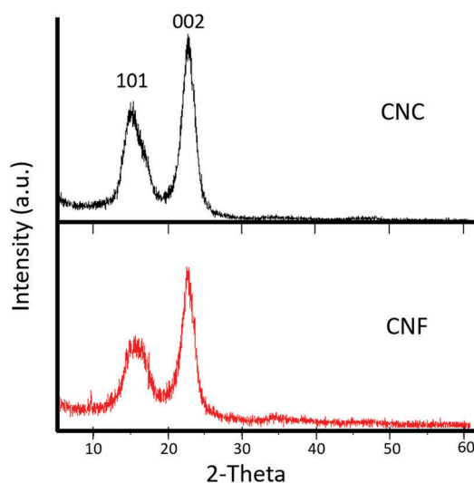
Fig. 9 Diffraction pattern for freeze dried CNCs (hydrolyzed using 64 wt% \text{H}_2\text{SO}_4 , 45^\circ\text{C} , 25 min) and CNFs (supplied by University of Maine) resolved into crystalline peaks and amorphous background (following the Ruland–Rietveld analytical approach). It is worthy of note that both CNC and CNF samples have the same crystallite size of 5.9 nm but different crystallinities, X_{c\text{-CNC}} = 86.2\% and X_{c\text{-CNF}} = 68.6\% .
