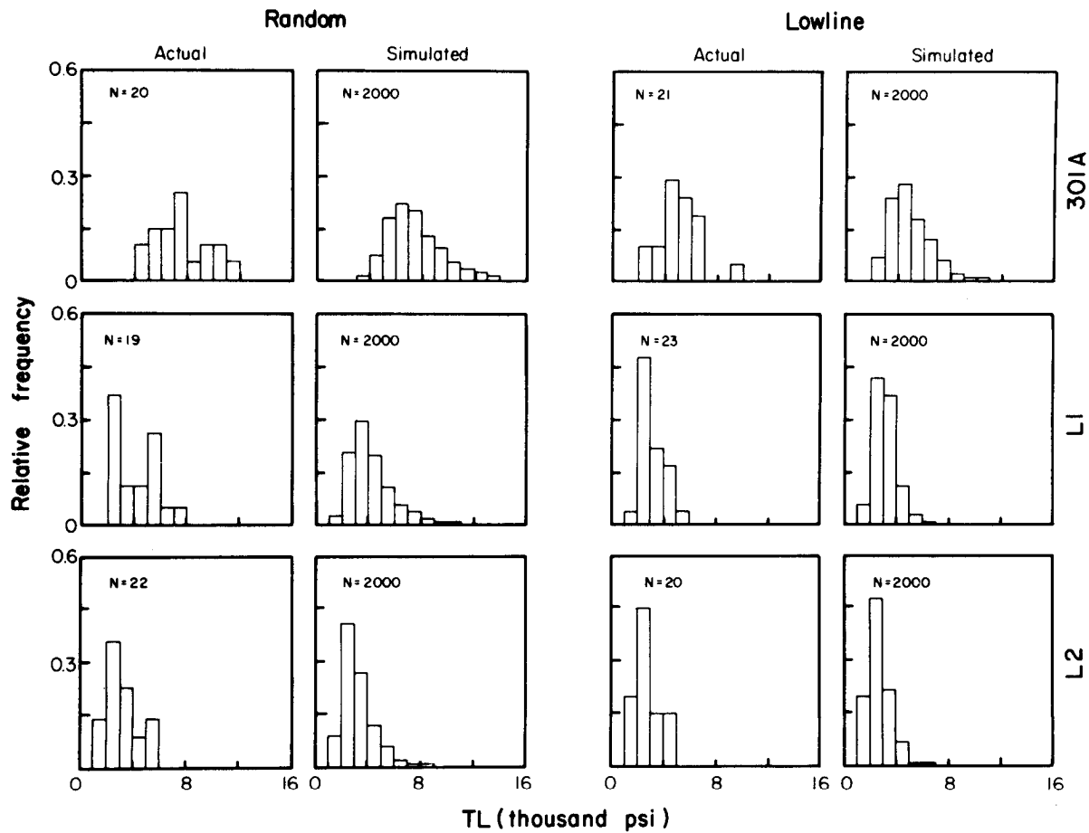
Figure 6.—Histograms for the actual and simulated tensile strength (TL) data for 2- by 6-inch Douglas-fir special laminating grade 301A and laminating grades L1 and L2 (random and lowline). Based on visual inspection, the simulated data for lowline closely mimic the data, whereas the simulated data for random only somewhat mimic the actual data. (ML85 5228)
