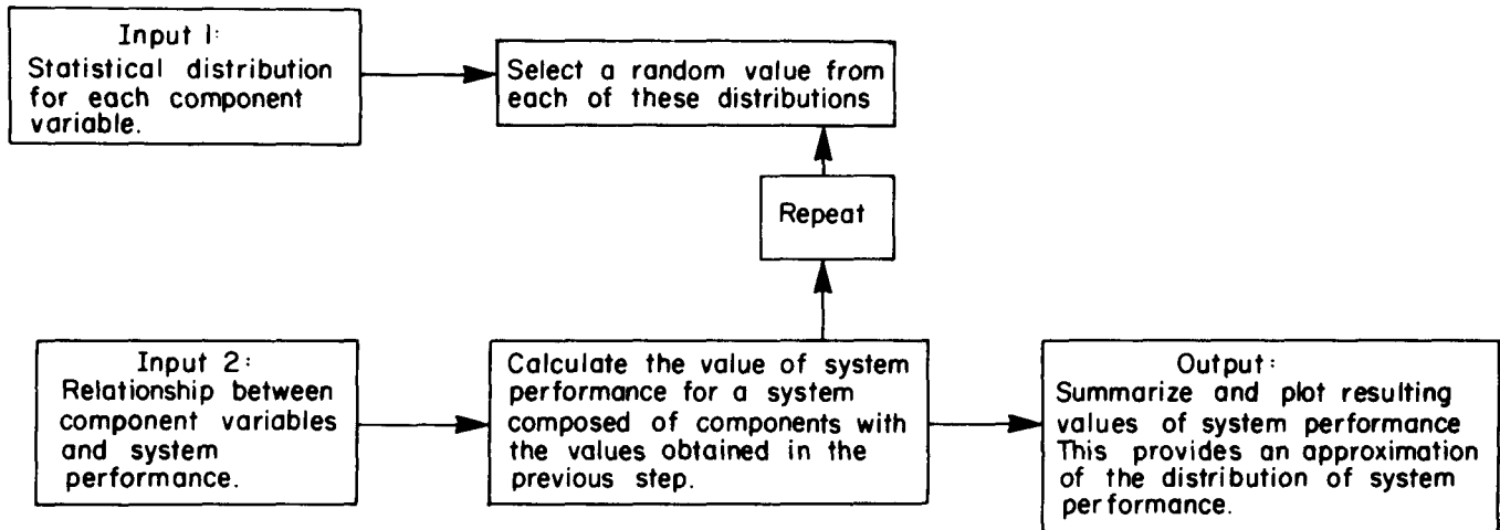
Figure 3.—Flow chart of the Monte Carlo simulation method (25). (ML85 5222)
