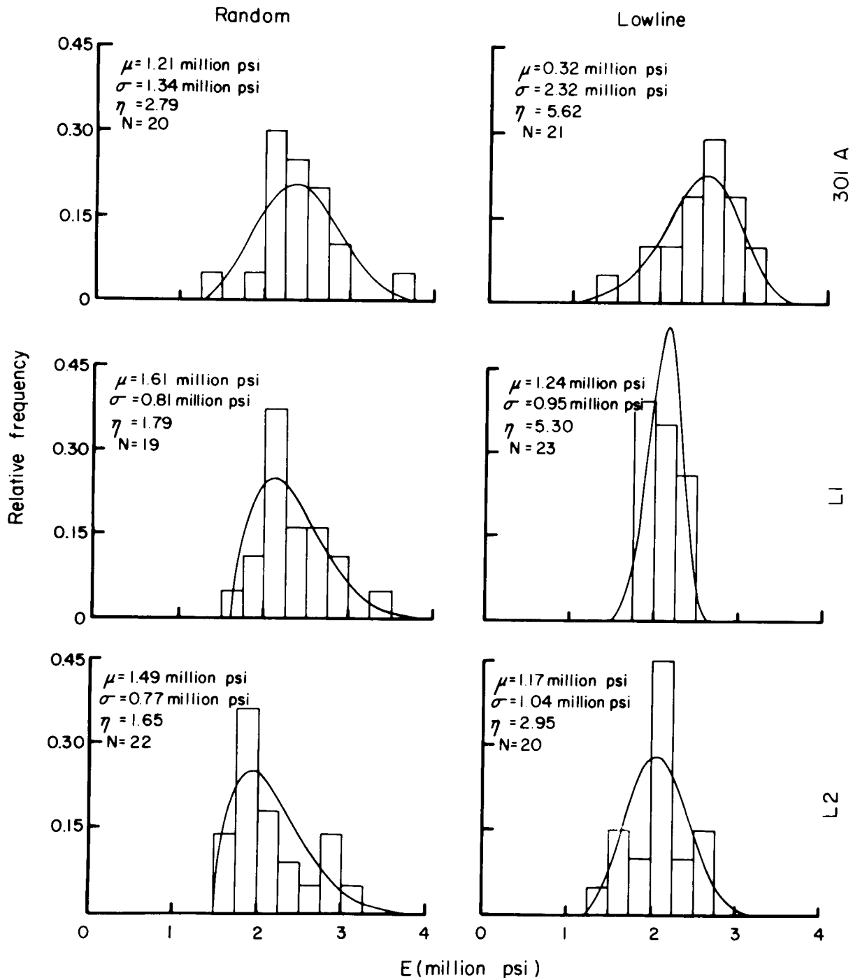
Figure 4.—Histograms of actual long span modulus of elasticity ( E ) data for 2- by 6-inch Douglas-fir special laminating grade 301A and laminating grades L1 and L2 (random and lowline). The three-parameter Weibull density function was fitted to the data, and the resulting curves coincide with the histograms. The lowline specimens were chosen to contain a near-maximum allowable strength-reducing characteristic for the grade (ML85 5226)
