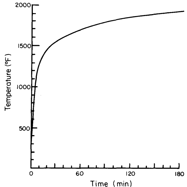
Figure 1.—The ASTM E 119 time-temperature curve (9). (ML85 5220)
