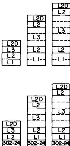
Figure 7.—Layups of the six beam groups used in the calibration of the beam strength model. Half of the beams had specially graded 302-24 lowline tension laminations and the other half had L1 lowline tension laminations. All other laminations were chosen to be a random sampling of the grade. The lamination grades are listed in order of increasing severity of defects as follows: 302-24, L1, L2D, L2, L3. (ML85 5225)
