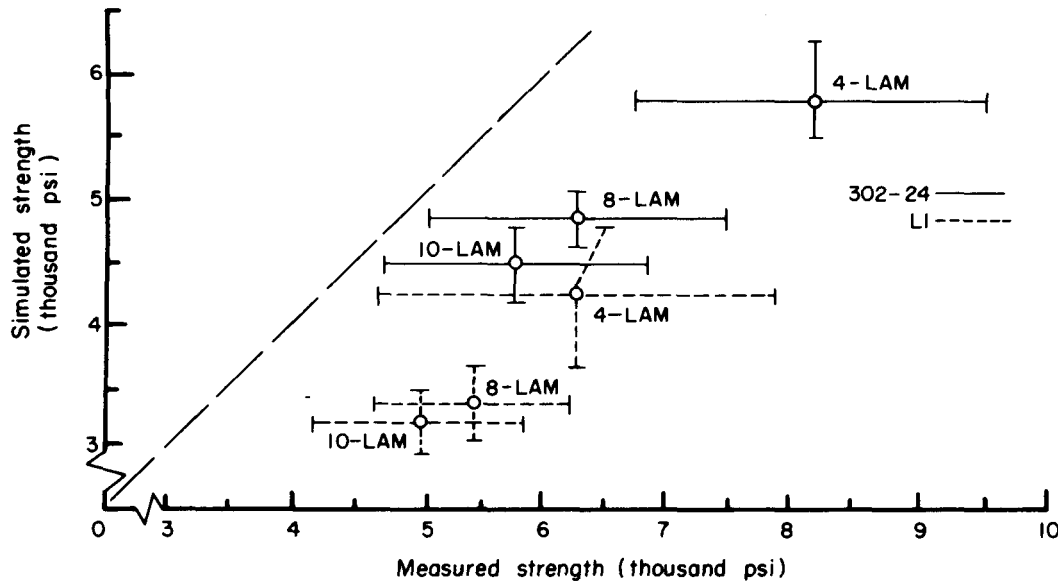
Figure 8.—Predicted beam strength means and variation (COV) (using the unrefined simulation model) vs. measured values. Tension laminations in the 4-, 8-, and 10-lamination beams are either L-1 or 302-24. (Data from table 4.) (ML85 5223)
