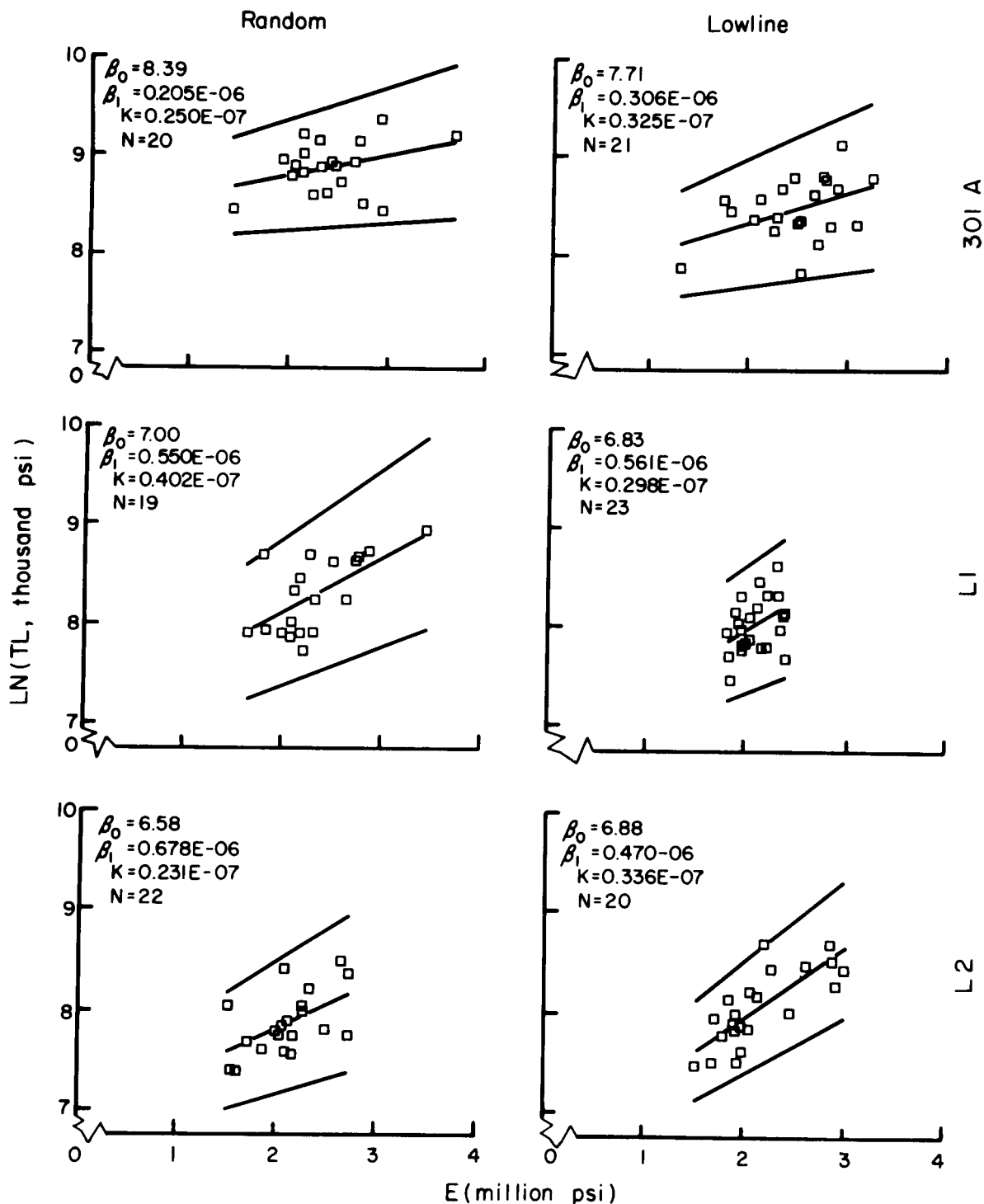
Figure 5.—Scattergram of the actual modulus of elasticity (E)-tensile strength (TL) pairs for 2- by 6-inch Douglas-fir special laminating grade 301A and laminating grades L1 and L2 (random and lowline). Overlays of the weighted least squares regression line and curves which bound 99 percent of the residuals are included. A logarithmic transformation was performed on the dependent variable, TL. The regression model appears to fit the data well. (ML85 5227)
