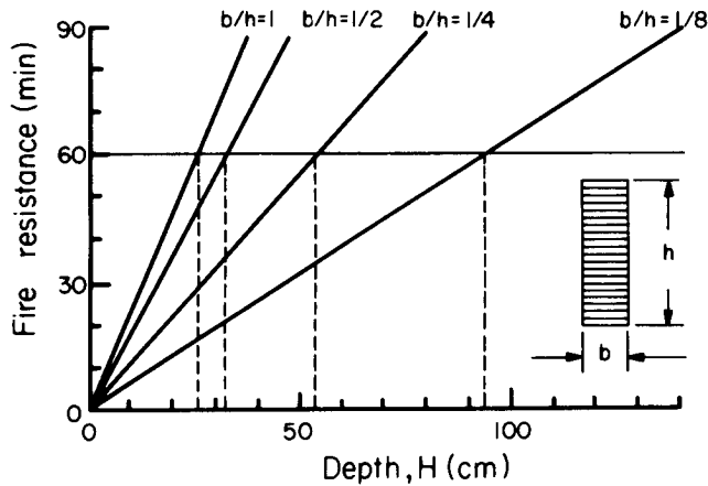
Figure 2.—Anticipated fire endurance for beams loaded to 100 percent of the design load. The temperature reduction factor is equal to unity, and the beams are exposed to fire on all four sides (28). (ML85 5221)
