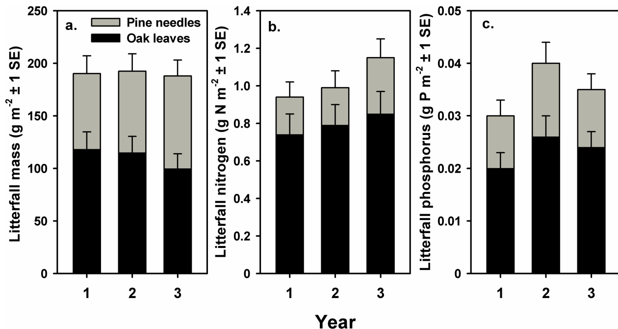
Fig 2. Annual fine litterfall flux derived from canopy foliage in longleaf pine forest at the Ordway-Swisher biological station. Values are mean \text{g m}^{-2} \text{yr}^{-1} \pm 1 \text{ SE} from 27 litterfall traps; a) mass, b) nitrogen, and c) phosphorus.
