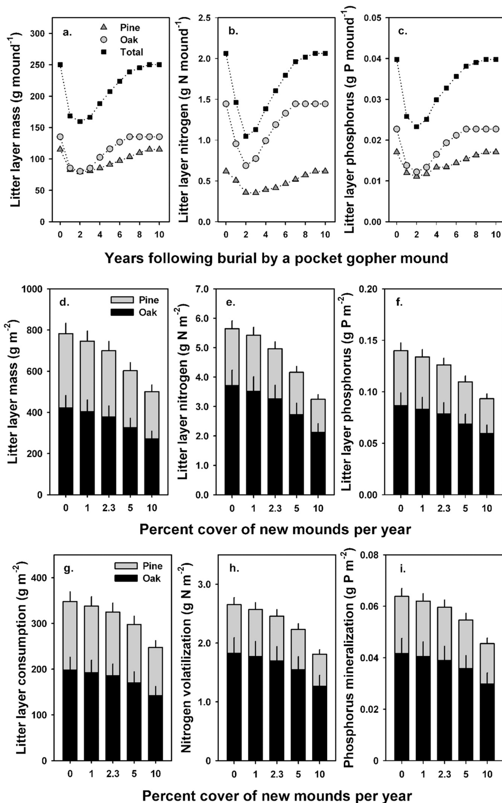
Fig 6. Model simulations of litter mass, nitrogen, and phosphorus content on the forest floor of a longleaf pine forest. (a-c) Litter layer dynamics of an individual pocket gopher mound over a 10-year period predicted by the single
