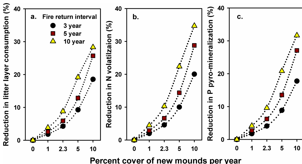
Fig 7. Simulated mass consumption, nitrogen volatilization, and phosphorus pyro-mineralization of the litter layer at three fire return intervals and five rates of pocket gopher mound formation. Simulated fire return intervals are 3, 5 and 10 years, and rates of new mound formation are 0%, 1%, 2.3%, 5% and 10% of the forest floor covered per year. Values are percent reduction of (a) mass consumption, (b) N volatilization, and (c) P pyro-mineralization predicted by the mound density and fire simulations compared to prescribed fire only simulations.
