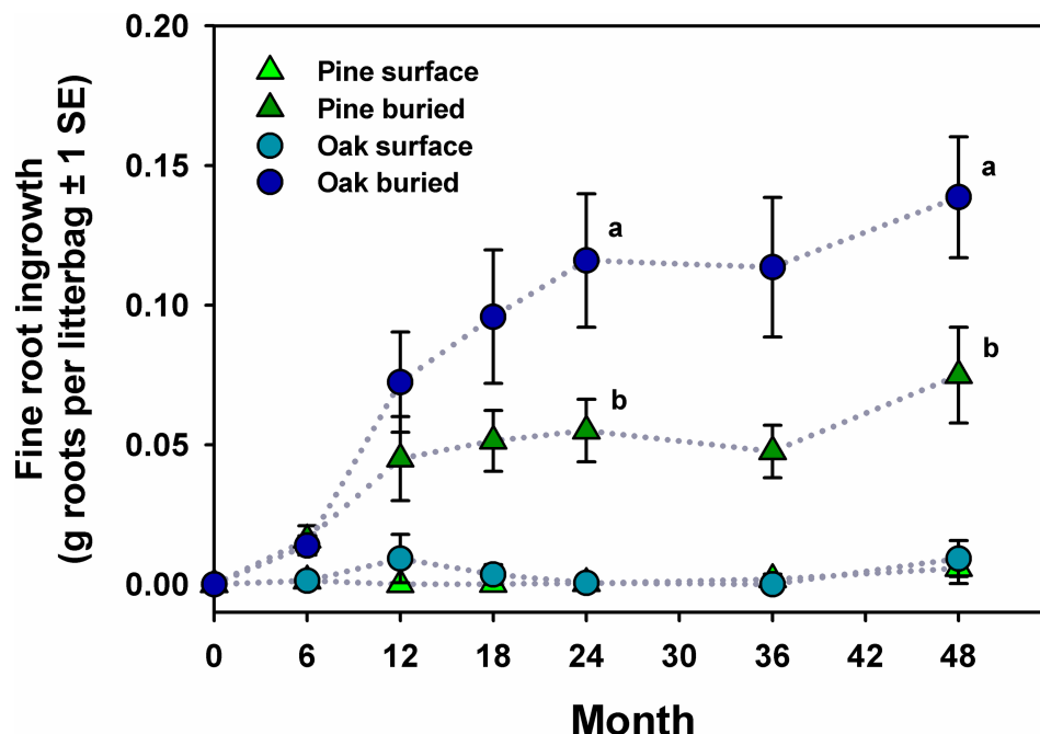
Fig 5. Fine root ingrowth into longleaf pine and turkey oak litter in litterbags on the surface of the forest floor and buried beneath pocket gopher mounds over a four year period. Values are mean g fine roots / litterbag \pm 1 SE.
