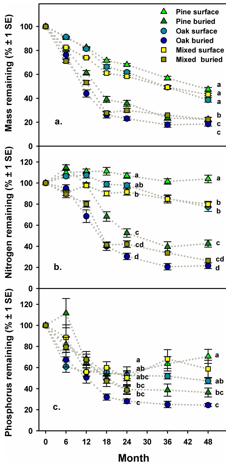
Fig 3. Decomposition and nitrogen and phosphorous dynamics of longleaf pine needle litter, turkey oak leaf litter, and mixed pine and oak litter in litterbags on the surface of the forest floor and buried beneath pocket gopher mounds over a four year period; a) percent of the initial mass remaining, b) percent of the initial nitrogen content remaining, and c) percent of the initial phosphorous content remaining. Values are means \pm 1 SE. Litter types and location that are significantly different ( p < 0.05 ) have different letters. Significance levels for percent mass remaining were calculated based on models for decomposition coefficients, k , calculated for sets of litterbags in each 0.5 ha plot. Complete statistics are in Table 2.
