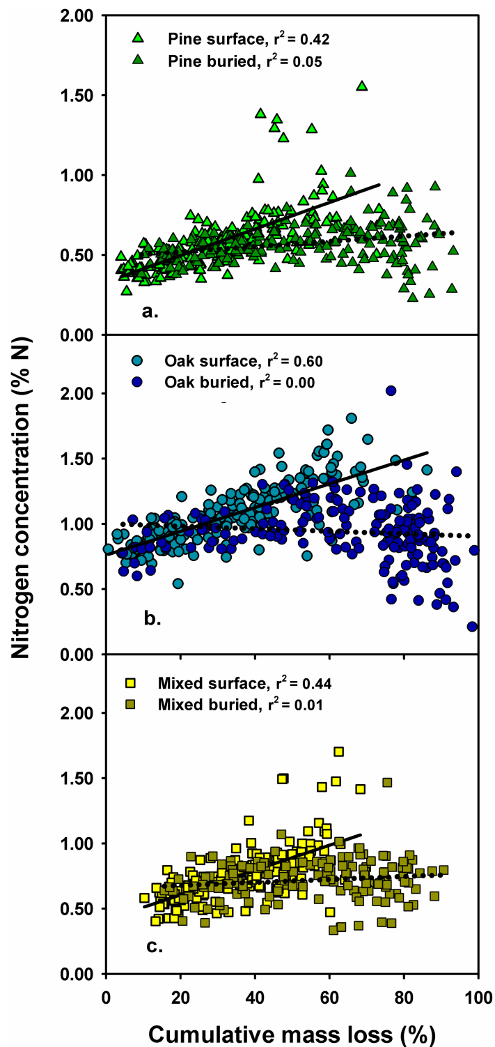
Fig 4. The relationship between cumulative mass loss and nitrogen concentration in litter in litterbags on the surface of the forest floor and buried beneath pocket gopher mounds over a four year period; a) longleaf pine litter, b) turkey oak litter, c) mixed pine and oak litter. Complete statistics for the regression lines for surface (solid lines) and buried (dotted lines) litterbags are in S3 Table.
