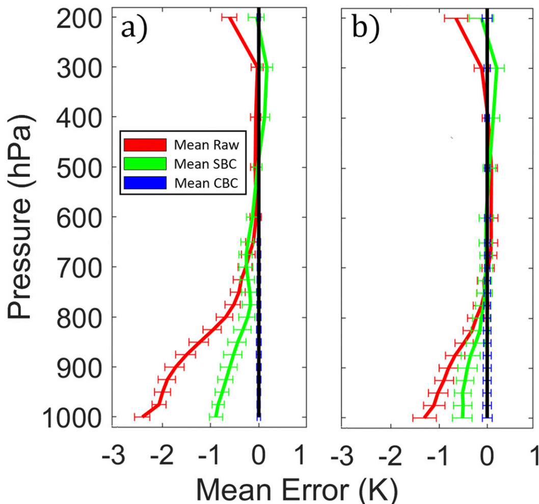
FIG. 9. ME-derived SREF ensemble mean temperature profiles of raw (red), SBC (green), and CBC (blue) for (a) SREF1 and (b) SREF2. Error bars represent the 25th and 975th permille of the 1000 resampled datasets.
