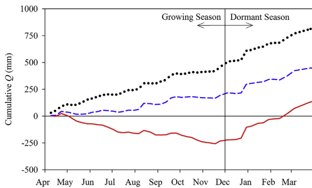
Fig. 8. Mean cumulative Q for SG (solid red line), LP (dashed blue line), and BA (dotted black line) based on weekly computed water balance. (For interpretation of the references to colour in this figure legend, the reader is referred to the Web version of this article.)
