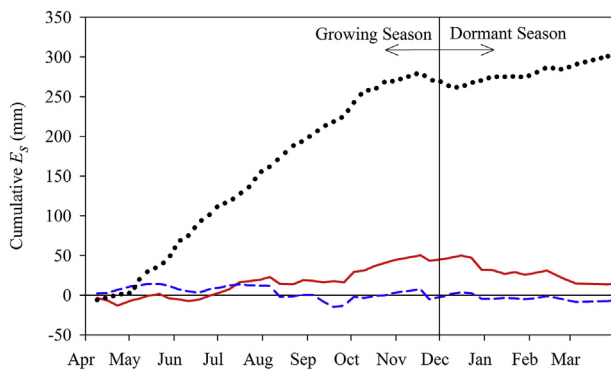
Fig. 4. Cumulative E_s for SG (solid red line), LP (dashed blue line), and BA (dotted black line) based on lysimeter measurements on approximately weekly intervals. (For interpretation of the references to colour in this figure legend, the reader is referred to the Web version of this article.)
