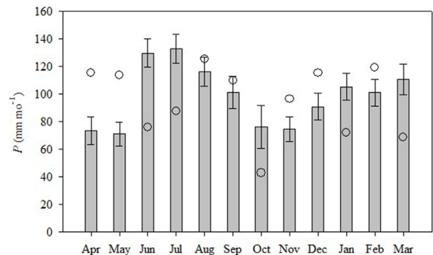
Fig. 2. Monthly P during the 2014–2015 water year measured at the study site (circles) and 1981–2010 long-term monthly mean P (bars ± SE).
