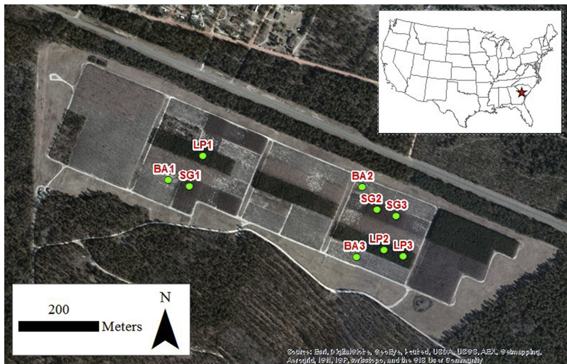
Fig. 1. Savannah River Site location in South Carolina, USA (inset) and vegetative plot locations. The first two characters of plot names identify the vegetation type (BA = bare, SG = sweetgum, LP = loblolly pine); the last character identifies the replicate plot number for that vegetation type.
