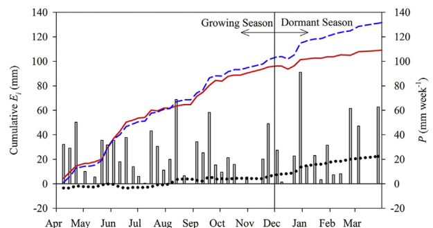
Fig. 3. Mean cumulative E i for SG (solid red line), LP (dashed blue line), and Mean cumulative E i LP − E i SG (dotted black line) calculated from throughfall measurements recorded on approximately weekly intervals. Also shown is the total P (grey bars) for each week. (For interpretation of the references to colour in this figure legend, the reader is referred to the Web version of this article.)
