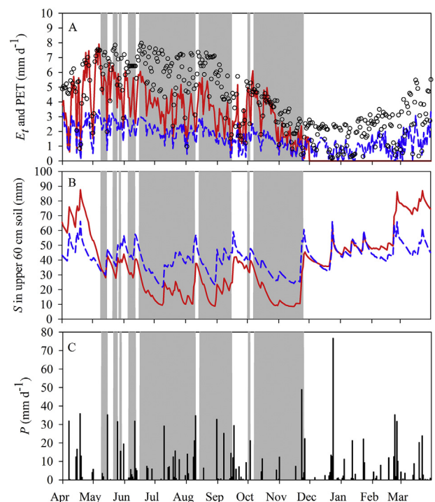
Fig. 7. Mean daily E_t for SG (solid red line), LP (dashed blue line), and PET (circles) (A), mean daily soil moisture storage ( S ) in the upper 60 cm of soil for SG (solid red line) and LP (dashed blue line) (B), and mean daily P (C). Areas shaded in grey indicate periods when the soil water content at the 35 cm depth in SG was less than the plant wilting point (greater than 15 bar tension). (For interpretation of the references to colour in this figure legend, the reader is referred to the Web version of this article.)
