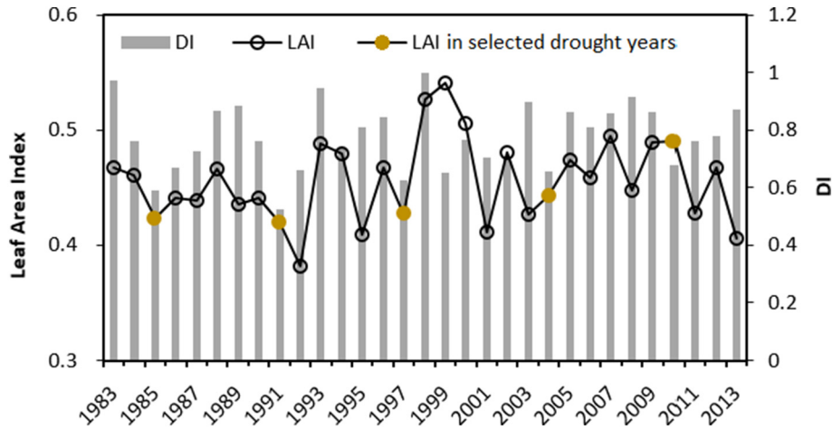
Fig. 2. Leaf area index (LAI) and growing season DI (P/PET) from June to September during 1983–2013 (the brown spots are selected drought years). (For interpretation of the references to colour in this figure legend, the reader is referred to the web version of this article.)
