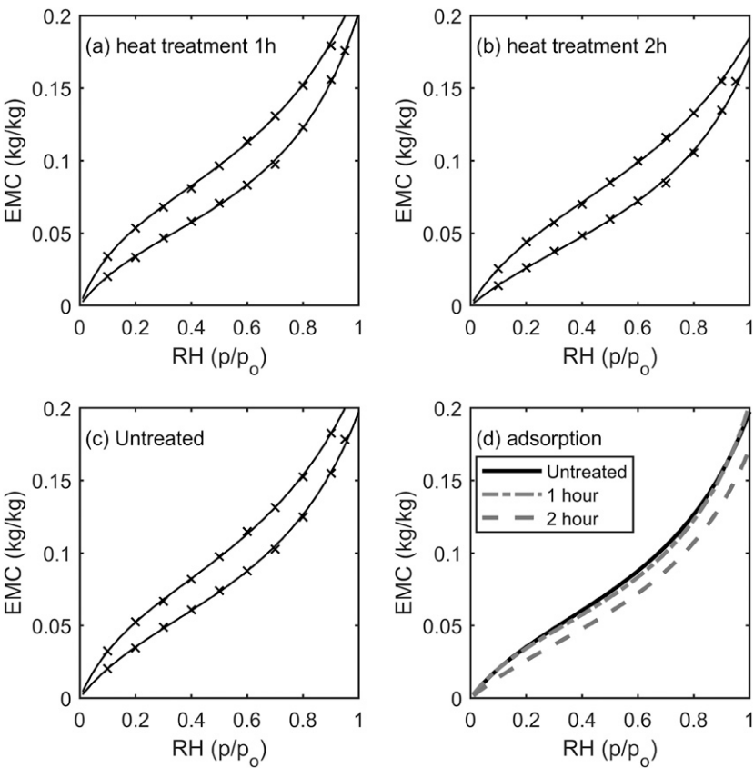
Figure 4. (a-c) Water vapor sorption isotherms for the heat-treated and untreated specimens. (d) Absorption isotherms from (a-c) overlaid.
