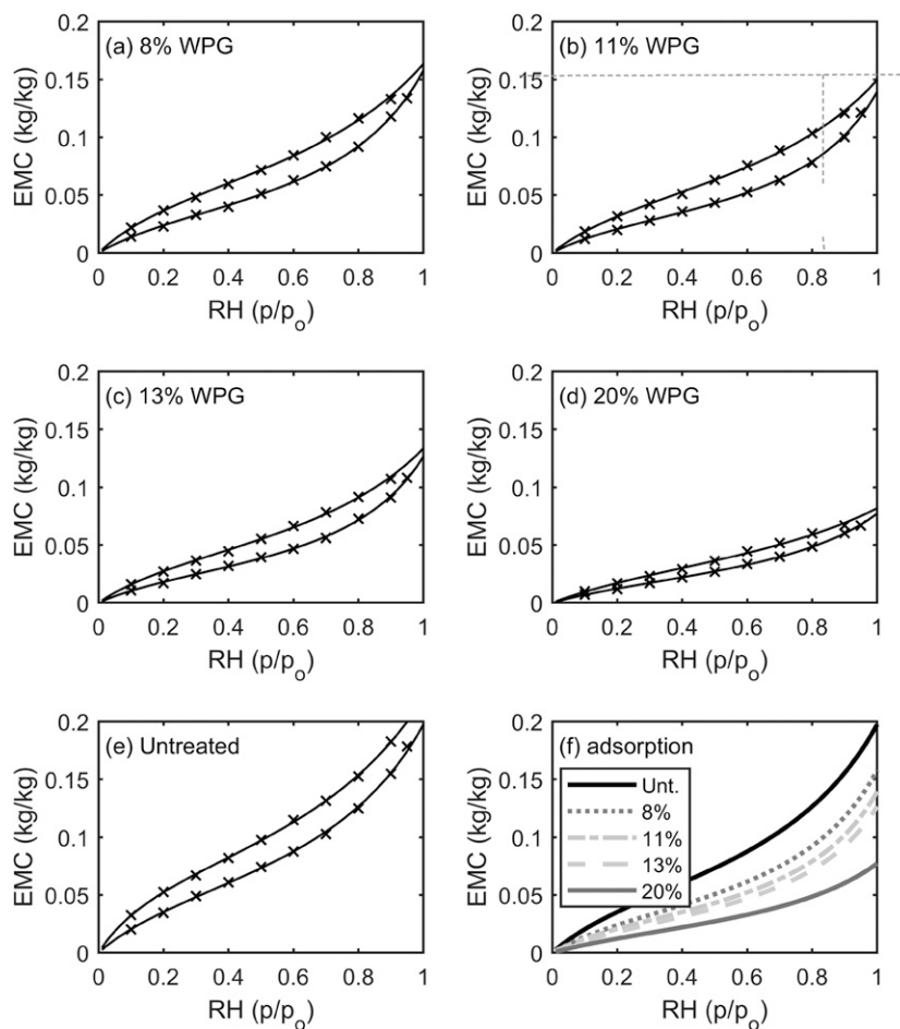
Figure 3. (a-e) Sorption isotherms for the acetylated and untreated samples. (f) Comparison of the absorption isotherms.
