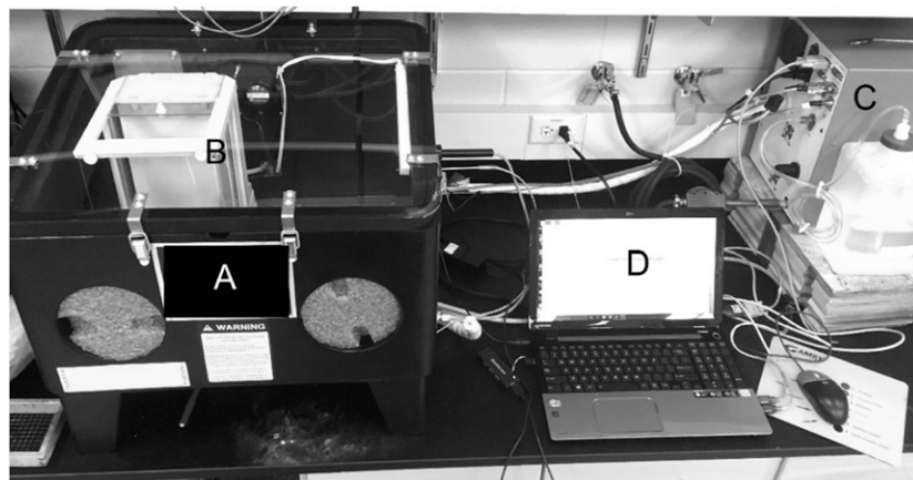
Figure 1. Photograph of the experimental setup including the enclosure (a), balance (b), humidity generator (c), and computer (d) for control and data acquisition.
