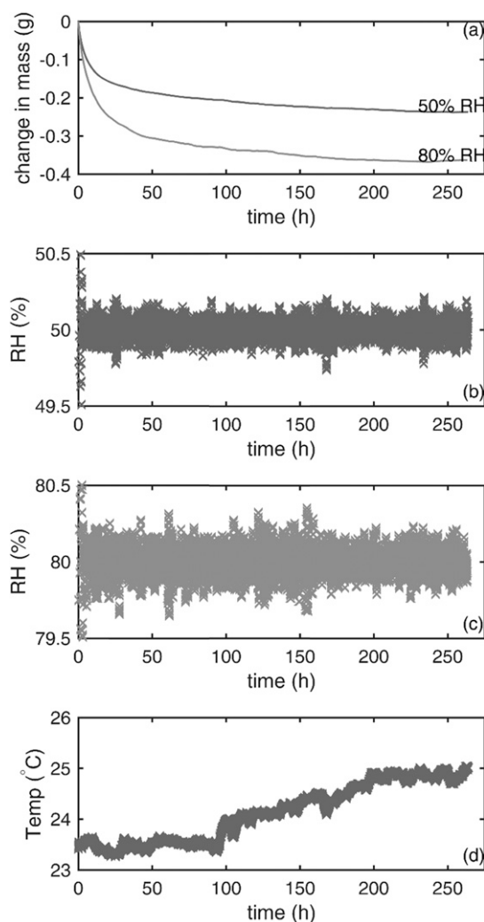
Figure 2. Example of representative change in mass as a function of time for the 60-50% RH and 90-80% RH steps. (b and c) Measured RH within the chamber during the desorption steps and (d) measured temperature within the chamber during the 50% RH desorption step.
