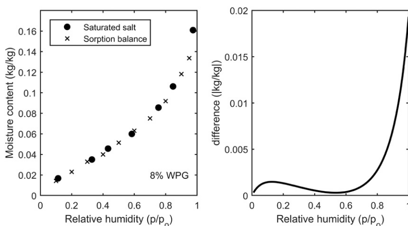
Figure 5. Comparison of the water vapor sorption isotherm of the 8% WPG sample collected with the saturated salt solution method (●) and with the parallel DVS apparatus presented in this article (×).
