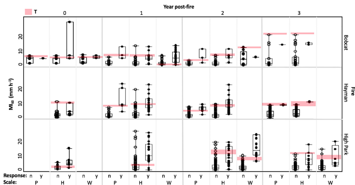
Fig. 3. MI 60 rainfall and thresholds ( T ) for unmulched sites (n; open circles) or presence (y; filled circles). Spatial scale abbreviations are plots (P), hillslopes (H) and watersheds (W). Box plots include: median (horizontal line), 25% and 75% quantiles (box), and observations (circles). Shaded areas are the range of MI 60 thresholds ( T ) that maximized the prediction accuracy ( F ) for each dataset.
