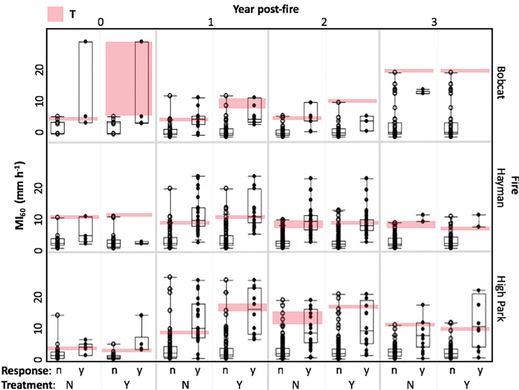
Fig. 4. MI 60 rainfall and thresholds (T) for hillslopes by mulch treatment (N/Y), year post-fire, fire, and response absence (n; open circles) or presence (y; filled circles). Box plots include the median (horizontal line), 25% and 75% quantiles (box), and observations (circles). Shaded areas are the range of MI 60 thresholds (T) that maximized the prediction accuracy (F) for each dataset.
