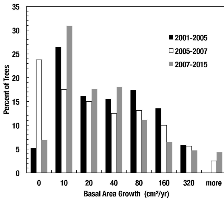
FIGURE 6. Histogram of basal area growth of trees measured at three time periods.
