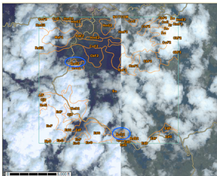
FIGURE 2. Map of our field sites circled, with major roads and soil types shown. So = serpentinite outcrops. NcD2 = Nipe Clay; RsE2 = Rosario Clay (USDA Web Soil Survey).
