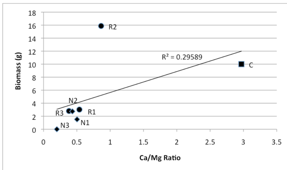
FIGURE 5. Plant-available Ca/Mg ratio vs. total biomass production.
