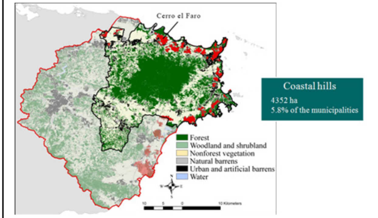
FIGURE 1. Coastal Hills (in red) of Northeastern Puerto Rico and the location of Cerro El Faro. This map was created by the GIS Remote Sensing Laboratory of the International Institute of Tropical Forestry and was made available through William Gould and Maya Quiñones.
