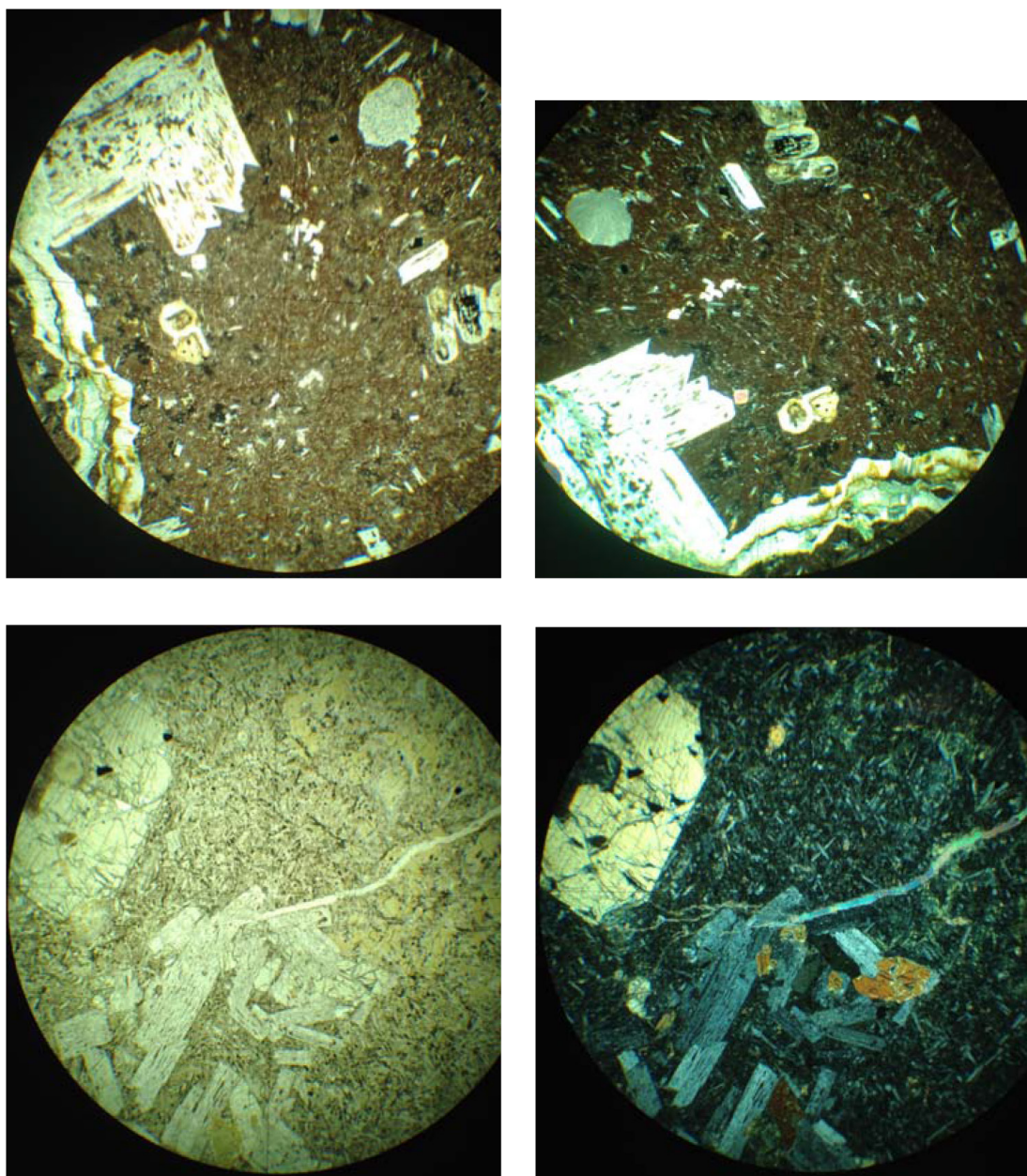
FIGURE 7. Thin section micrographs of (clockwise from top left) P2 rim PPL pillow, P2 rim CPL pillow, P2 core PPL pillow, and P2 core CPL pillow. Rims have cryptocrystalline/glassy groundmass with significant secondary alteration, especially of ferromagnesian minerals and glass. Sieve texture of K-feldspar phenocrysts suggests disequilibrium crystallization. Fractures are significantly chloritized, indicating relatively high-T remineralization post-emplacement. Pillow cores are relatively unaltered, with intact K-feldspar phenocrysts and glomerporphyritic plagioclase and augite. Plagioclase microphenocrysts are significantly larger in groundmass; optically resolvable augite microcrysts are present in groundmass, which is significantly less glassy than pillow rims.
