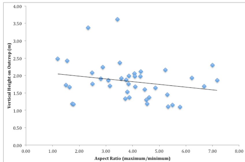
FIGURE 6. Inverse relationship between aspect ratio and increasing vertical position of the pillow. Higher aspect ratios correspond to position further down in the section.
