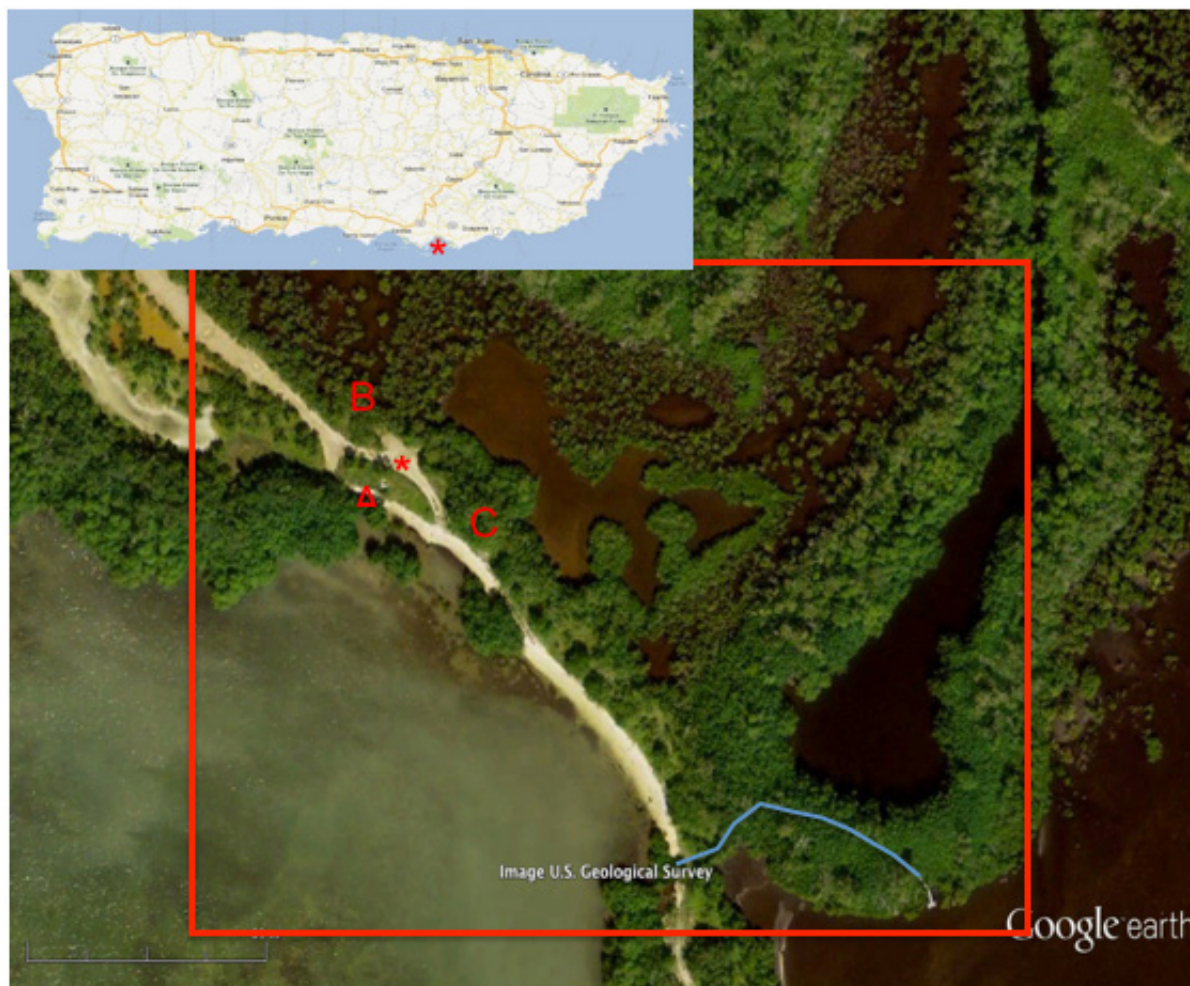
FIGURE 1. Study site: Camino de los Indios, Jobos Bay, Guayama, PR. The blue line indicates the location of the wooden path within the fringe mangrove. Imagery date: 11/1/2006. Lat 17.935437° long -66.253300° elev 0 m eye alt 298 m *Main camp; A Fringe site ( R. mangle + L. racemosa ; B Basin site ( A. germinans ); C Bank site ( Thespesia populnea )
