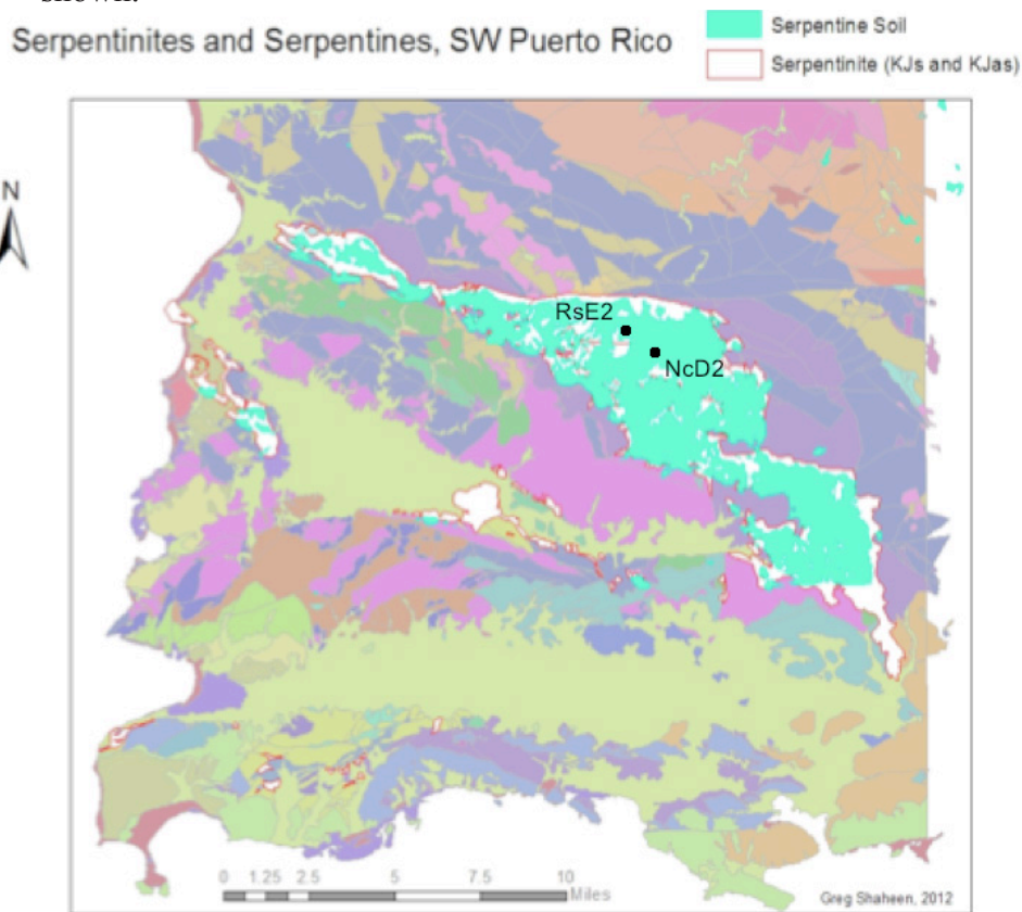
FIGURE 1. Extent of serpentinite rock outcrops and serpentine soils in southwest Puerto Rico (Leonard et al. 2013). Geographical context of our field sites, NcD2 and RsE2, is shown.
