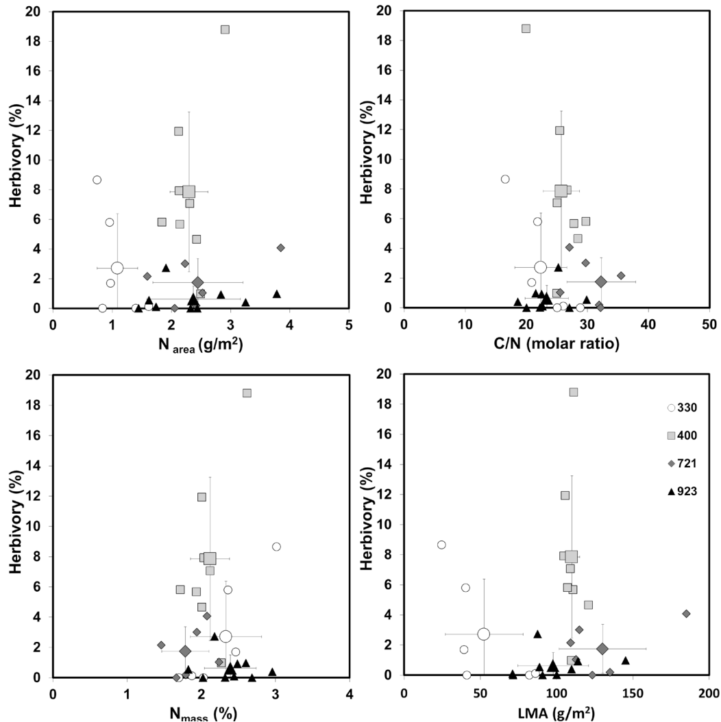
FIGURE 3. Comparison of herbivory versus N_{area} (top left), C/N (top right), N_{mass} (bottom left) and LMA (bottom right). Individual leaves are shown by the smaller points and grouped by elevation (meters asl). The larger points represent the means for each elevation, with the error bar representing one standard deviation.
