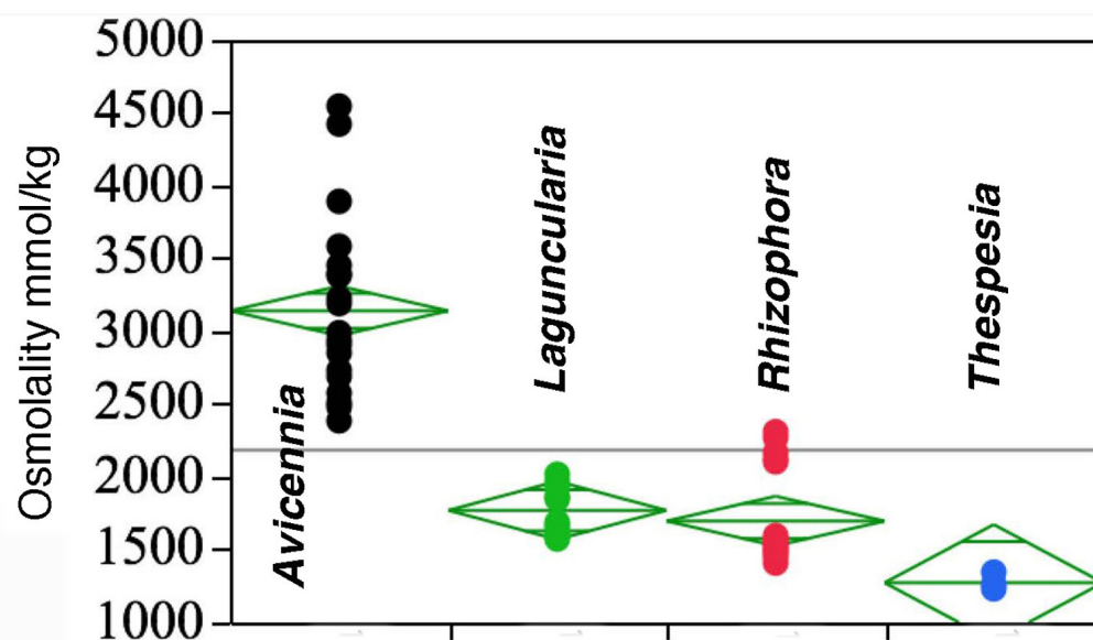
FIGURE 5. Osmometry of leaf sap obtained from adult leaves. The green diamonds correspond to the visual representation of the one-way analysis of variance performed by JMP. Black dots: Avicennia ; Green dots: Laguncularia ; Red dots: Rhizophora . Y: young leaves; A: adult leaves; O: old leaves. Significance of the green diamonds as in Fig 3.
