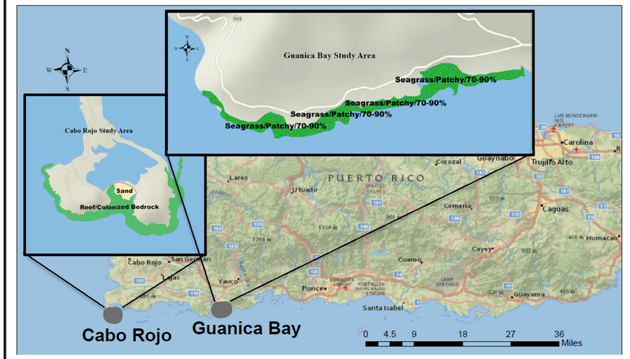
FIGURE 2. Map of Puerto Rico with locations of non-pristine (Guánica Bay; right inset) and pristine (Cabo Rojo; left inset) sites. Seagrass is shown in green (Whitall et al. 2014).
