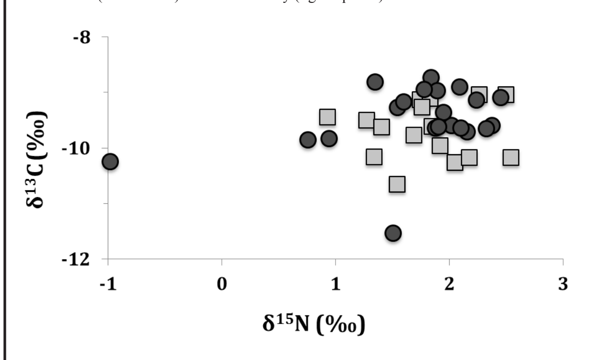
FIGURE 3. \delta^{13}\text{C} and \delta^{15}\text{N} results for Thalassia from both seagrass bed sites. Each data point represents the \delta^{13}\text{C}:\delta^{15}\text{N} ratio for individual leaf tissue samples from Cabo Rojo (dark circles) and Guánica Bay (light squares).
