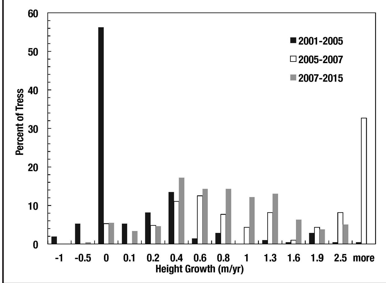
FIGURE 7. Histogram of height growth the trees measured at three time periods.
