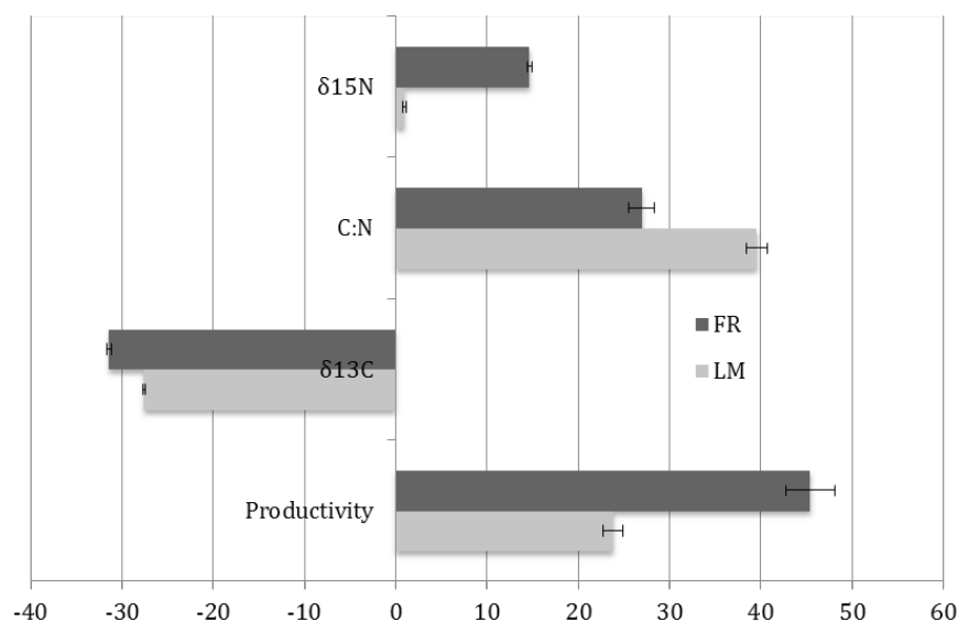
FIGURE 2. Mean carbon and nitrogen isotopic values (‰), C:N mass ratio, and calculated productivity ( \delta^{13}\text{C} \times \text{weight percent nitrogen} ) measured at each site. Bars are standard errors of the mean. FR = Fajardo River site (more polluted); LM = Los Machos site (less polluted).
