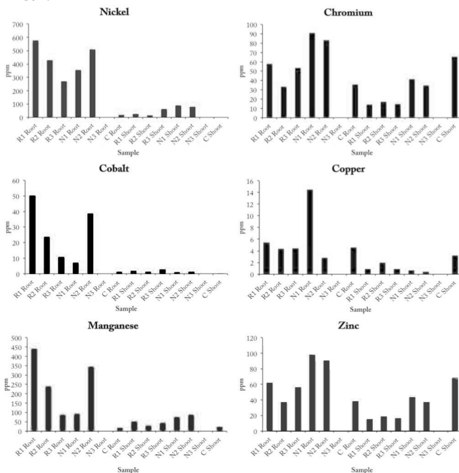
FIGURE 4. Concentrations of heavy metals in roots and shoots of Brassica juncea . The y-axis scaling differs by metal. Since there was no biomass production in soil N3, there was no biomass to analyze. N = Nipe Clay; R = Rosario Clay; C = Control potting soil.
