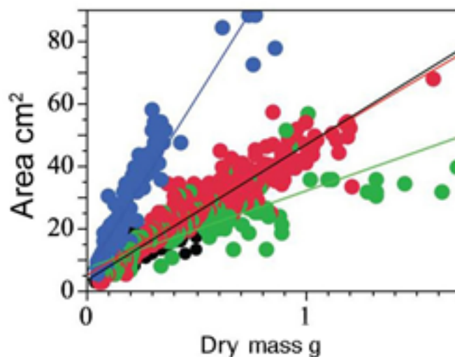
FIGURE 3. Area/mass relationship of different species from tree species at Jobos Bay. The regression equations are: Area ( A \text{ cm}^2 ) and mass ( W \text{ g} ) Thespesia (blue) A = 5.615 + 111.890 W ; R^2 \text{ adj} = 0.87 ; F = 927 , P > F < 0.0001 ; n = 146 Avicennia (black) A = 3.235 + 43.358 W ; R^2 \text{ adj} = 0.75 ; F = 893 , P > F < 0.0001 ; n = 299 Rhizophora (red) A = 4.857 + 41.599 W ; R^2 \text{ adj} = 0.89 ; F = 2436 , P > F < 0.0001 ; n = 297 Laguncularia (green) A = 7.146 + 24.772 W ; R^2 \text{ adj} = 0.68 ; F = 321 , P > F < 0.0001 ; n = 149
