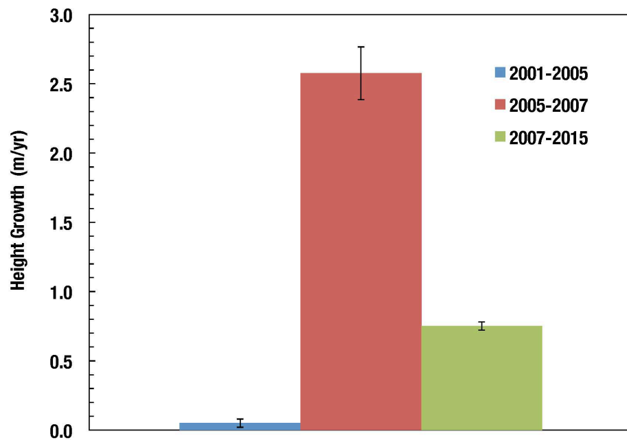
FIGURE 8. Histogram of average tree height growth rates during the three time periods. The vertical lines represent the standard error of the mean ( n = 238 ).
