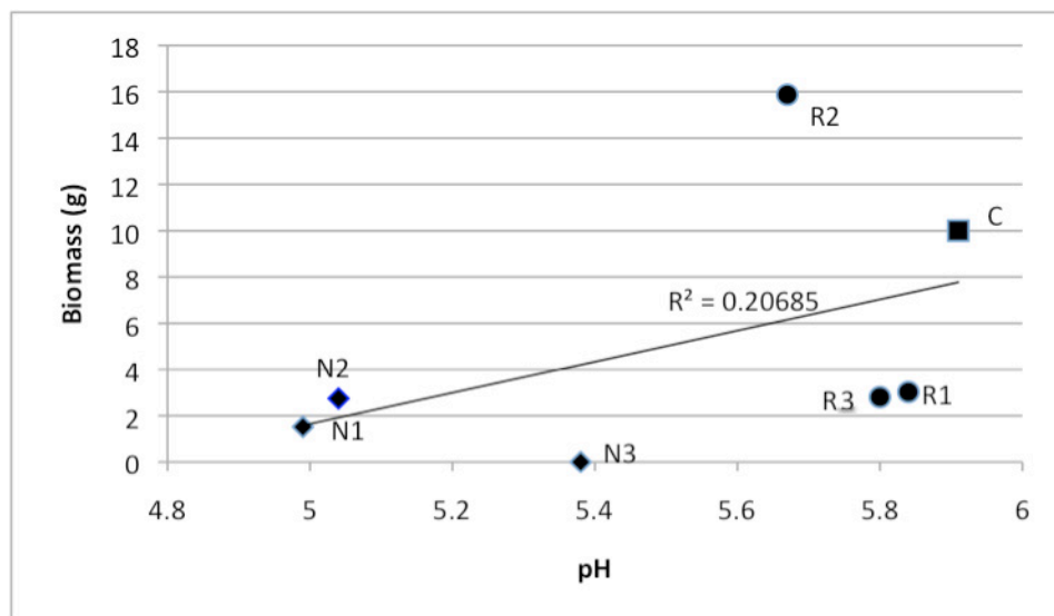
FIGURE 6. Soil pH vs. total biomass production.
