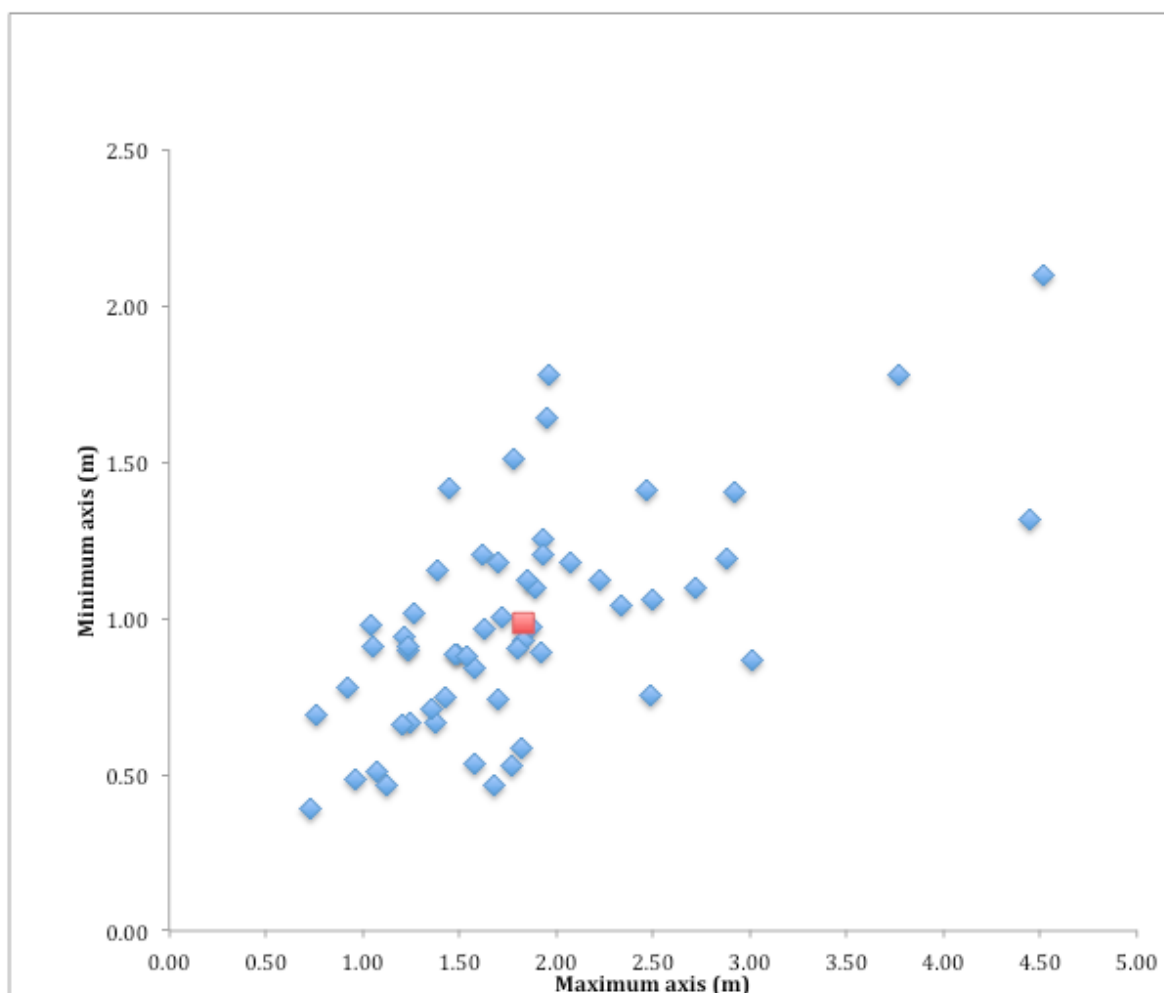
FIGURE 4. Maximum and minimum pillow dimensions for 56 pillows (blue diamonds), and average maximum and minimum axes (red square).
