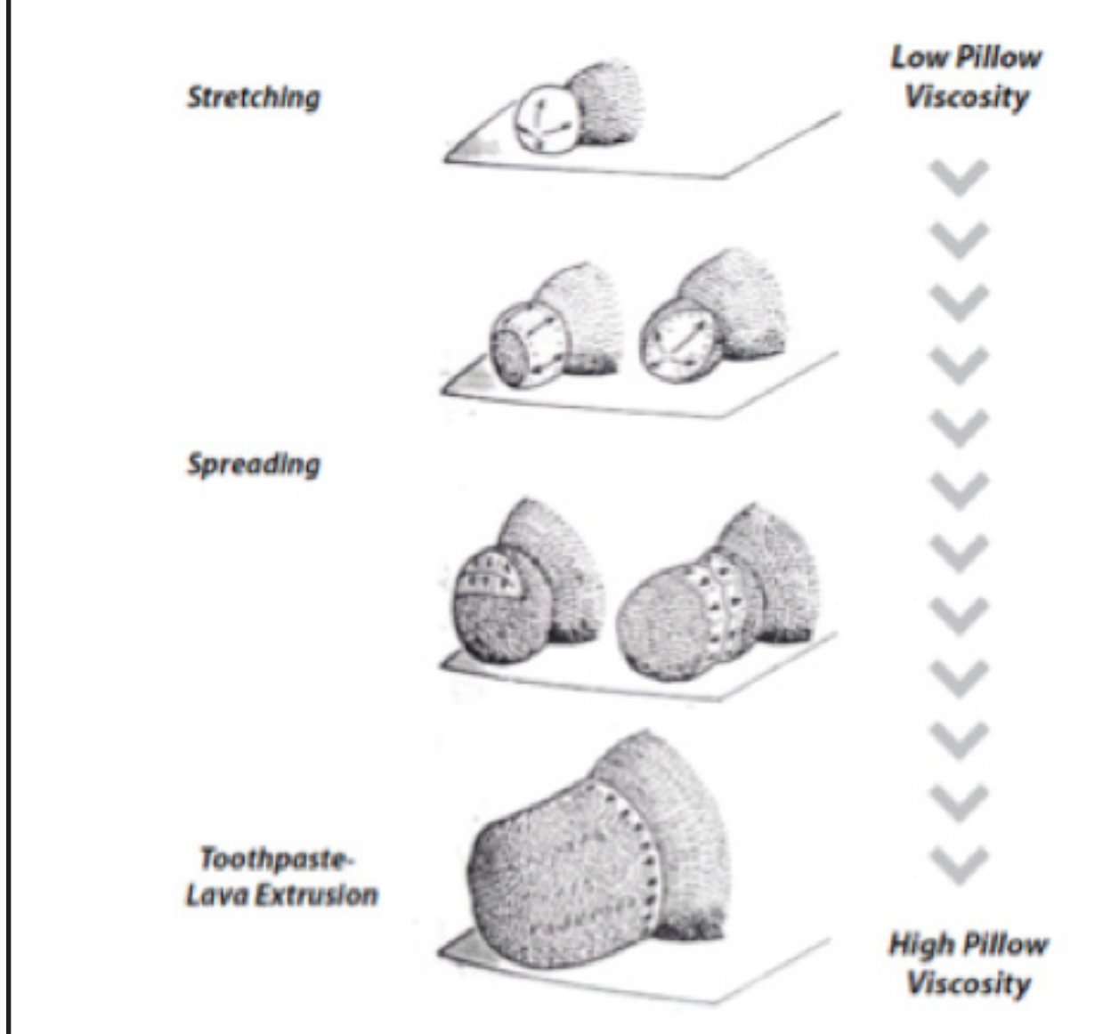
FIGURE 8. Walker's classification of pillow growth related to increasing lava viscosity. The first mechanism is characterized by uniform localized stretching of the chilled, relatively smooth skin. Pillows of the highest viscosity grow by toothpaste-like extrusion where lava is pushed from the solidified pillow; these pillows are usually rough surfaced. (Schnur 2007).
