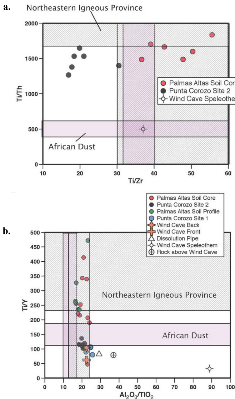
FIGURE 2. a) Bivariate plot of Ti/Th vs. Ti/Zr; b) Bivariate plot of Ti/Y vs. Al_2O_3/TiO_2 . The pink area delineates the range of African dust; the shaded grey area delineates the northeastern igneous rocks (data from Schellekens 1998). The overlapping area of pink (or shaded) rectangles in each plot denotes the area that African dust (or igneous rock source) is most likely to be present.
