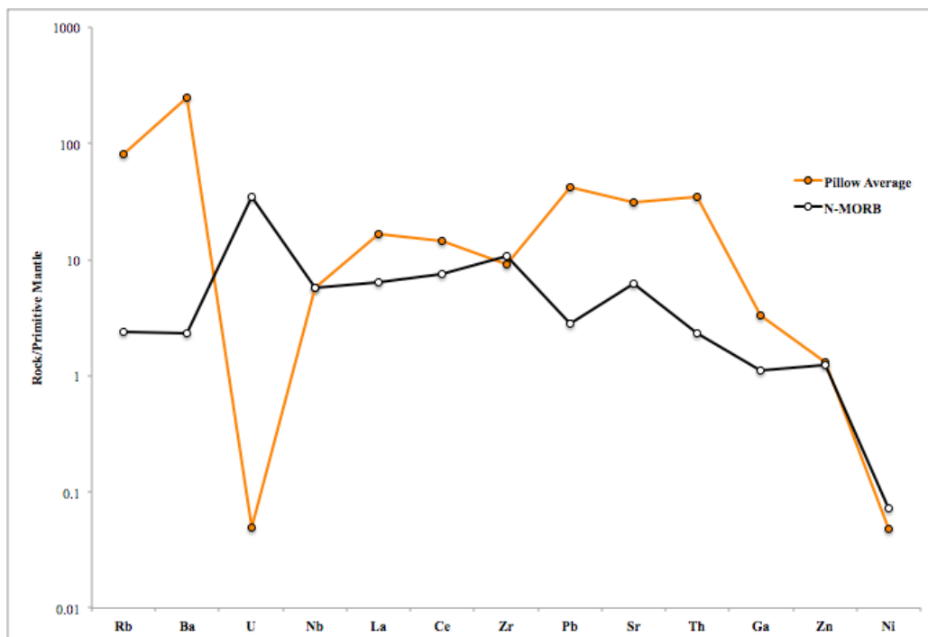
FIGURE 10. Trace elements in the 2014 Lapa Lava pillows and N-MORB, normalized to primitive mantle. N-MORB and primitive mantle compositions from Halliday et al. 1995; Hofmann 1988; Sun 1982. U was not detected in the analyses but is assumed to be present in very low concentration. Despite apparent U depletion, the pillow lava is enriched overall in HFSE and LILE relative to N-MORB.
