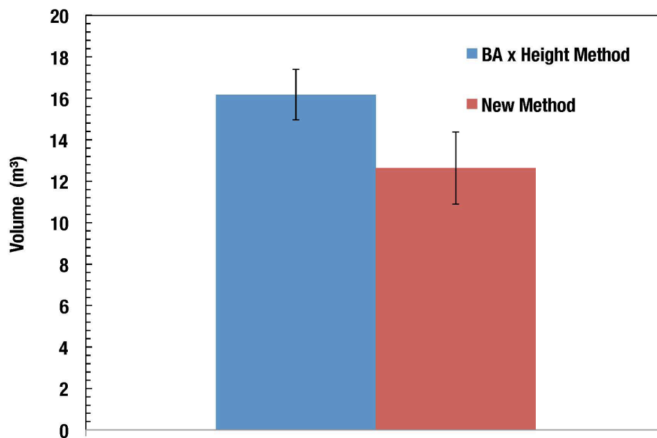
FIGURE 10. Histogram of the volume of four trees measured using our new method vs. the volume of those same trees using the traditional method for trees in natural forests (product between tree basal area and height). The lines represent standard error of the mean ( n = 4 ).
