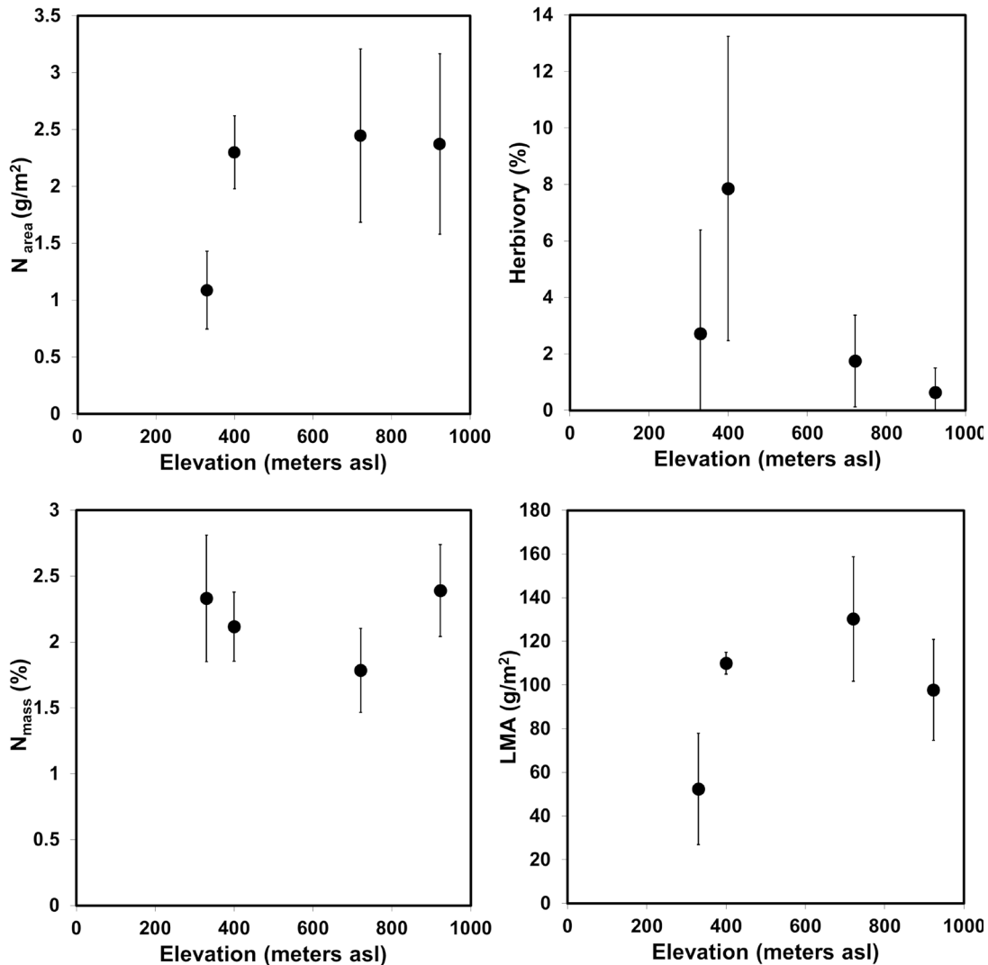
FIGURE 2. N_{area} (top left), herbivory (top right), N_{mass} (bottom left) and LMA (bottom right) versus elevation. Points represent sample means of individual leaves (at 330 m n = 6 for LMA, herbivory, and N_{area} ; n = 8 for N_{mass} ; at 400 m n = 8 for LMA, herbivory, and N_{area} ; n = 9 for N_{mass} ; at 721 m n = 6 for LMA, herbivory, and N_{area} ; n = 9 for N_{mass} ; at 923 m n = 9 for LMA, herbivory, N_{area} , and N_{mass} ). Error bars show one standard deviation.
