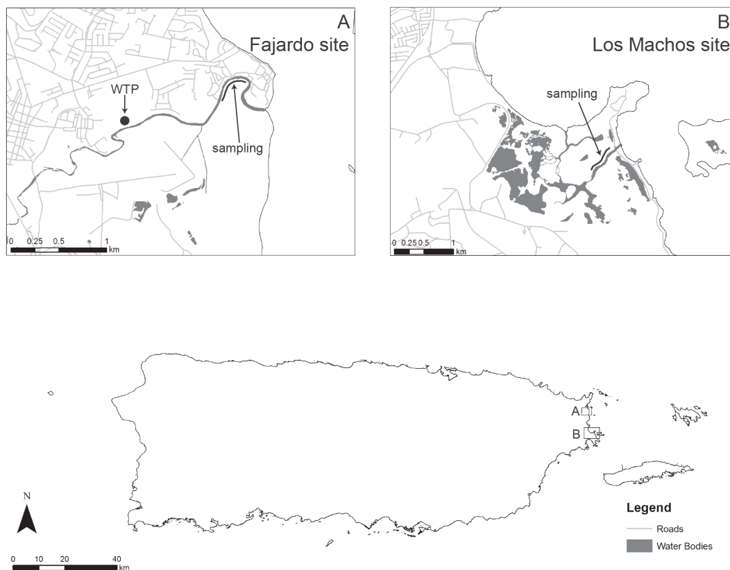
FIGURE 1. Map of sampling areas. Black labeled lines demarcate the boundaries of our sampling (leaves were sampled from both sides of each water channel). An old wastewater treatment plant is marked (“WTP”). The active Fajardo Regional Wastewater Treatment Plant is ~5 km upriver from our sampling at the Fajardo site. Map made in ARC GIS using data from http://gis.pr.gov .
