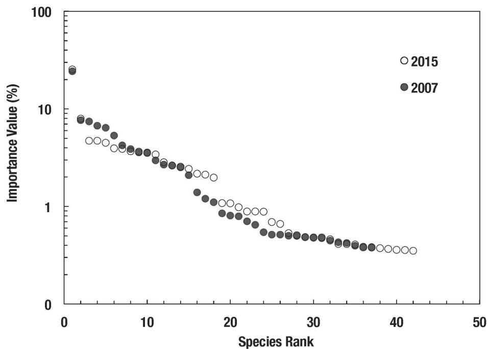
FIGURE 2. Species Importance Value Curve demonstrating species dominance over two different periods and showing species increase in 2015.
