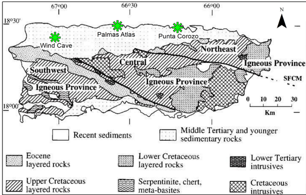
FIGURE 1. Geologic map of Puerto Rico with sampling locations (after Schellekens 1998). The white stippled area denotes carbonates. Coordinates for the sampling locations are Punta Corozo (Core 1: 18.4685, -66.199227; Core 2: 18.468141, -66.199017), Palmas Altas (Profile: 18.48393, -66.5756; Core: 18.484099, -66.574943), and the Cave of the Wind (18.417744, -66.967594). More detailed maps of the sampling locations are available from the authors.
