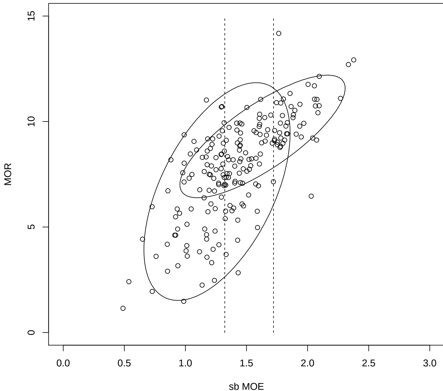
Figure 18: Scatter plot of MOR versus sb MOE, and 0.90 probability content contours for the two bivariate normal components of the fitted mixed bivariate normal model. The vertical lines are at the 0.40 and 0.80 sb MOE quantiles estimated from the marginal sb MOE distribution calculated from the fitted mixed bivariate normal model.
