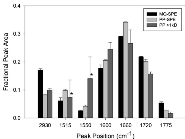
Fig. 4. Relative peak areas for peaks identified in the 1500–1800 \text{cm}^{-1} range from peak fitting. Peak areas for C–H stretching peaks at 2850–2950 \text{cm}^{-1} are also shown. * Note that the peak positions for the PP > 1kD fraction shifted to ~1500 and 1540 \text{cm}^{-1} .
