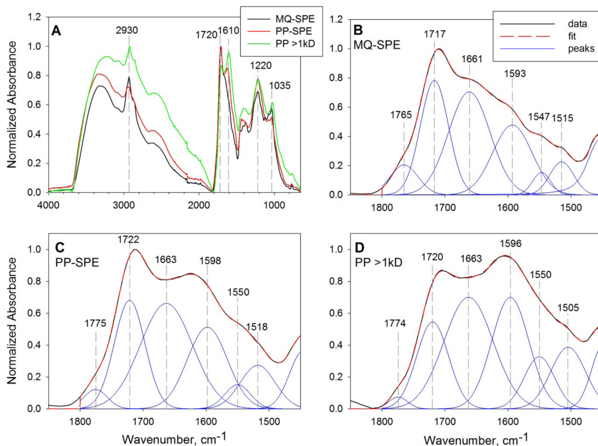
Fig. 3. Normalized ATR-FTIR spectra for isolated NOM fractions from LRC sediment. (A) Comparison of extracts over entire spectral range, and close up of 1500–1800 \text{cm}^{-1} with peak fits for (B) MQ-SPE, (C) PP-SPE, and (D) PP > 1kD fractions.
