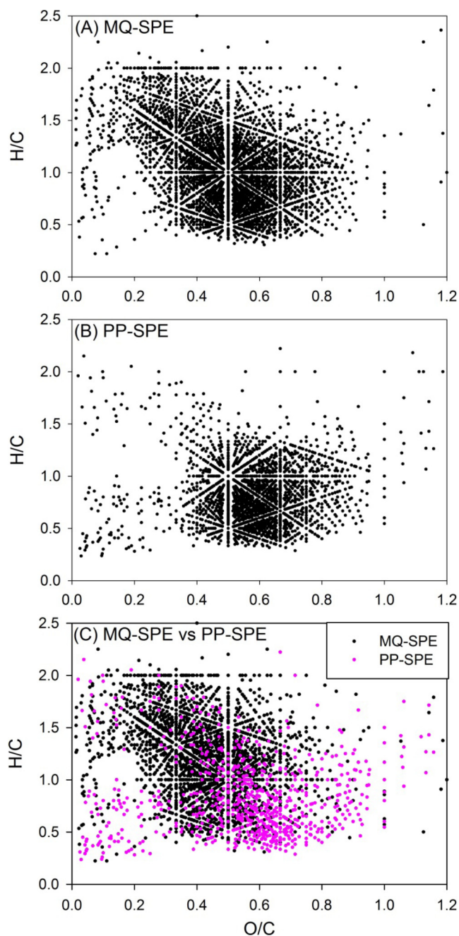
Fig. 5. Example ESI-FTICR-MS van Krevelen diagrams showing all peaks for (A) MQ-SPE and (B) PP-SPE fractions of NOM isolated from LRC sediment, and (C) comparison of unique peaks for MQ-SPE (black) and PP-SPE (pink). (For interpretation of the references to colour in this figure legend, the reader is referred to the web version of this article.)
