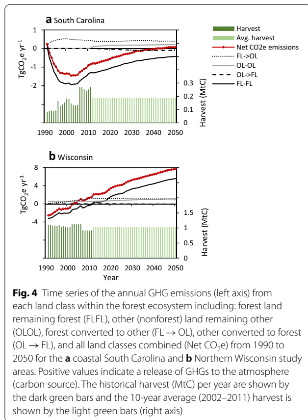
Fig. 4 Time series of the annual GHG emissions (left axis) from each land class within the forest ecosystem including: forest land remaining forest (FLFL), other (nonforest) land remaining other (OLOL), forest converted to other (FL → OL), other converted to forest (OL → FL), and all land classes combined (Net \text{CO}_2\text{e} ) from 1990 to 2050 for the a coastal South Carolina and b Northern Wisconsin study areas. Positive values indicate a release of GHGs to the atmosphere (carbon source). The historical harvest ( \text{MtC} ) per year are shown by the dark green bars and the 10-year average (2002–2011) harvest is shown by the light green bars (right axis)
