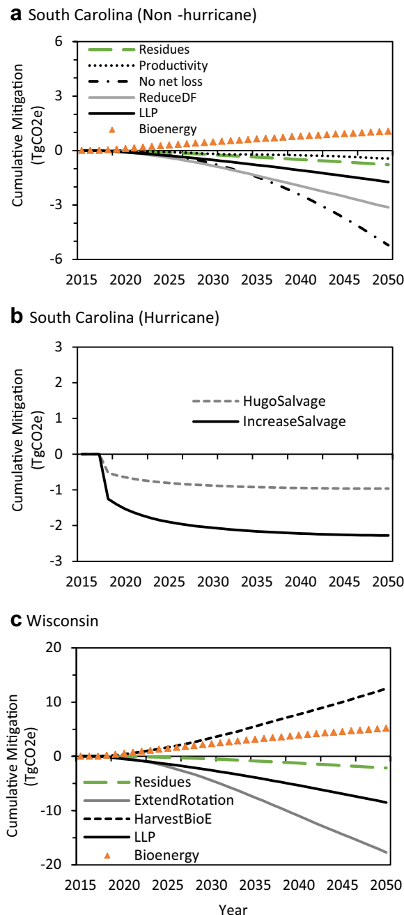
Fig. 6 Time series of the total cumulative mitigation relative to the baseline for each scenario for a coastal South Carolina (non-hurricane scenarios), b coastal South Carolina (hurricane scenarios), and c Northern Wisconsin study areas. Negative values denote a reduction in GHG emissions
