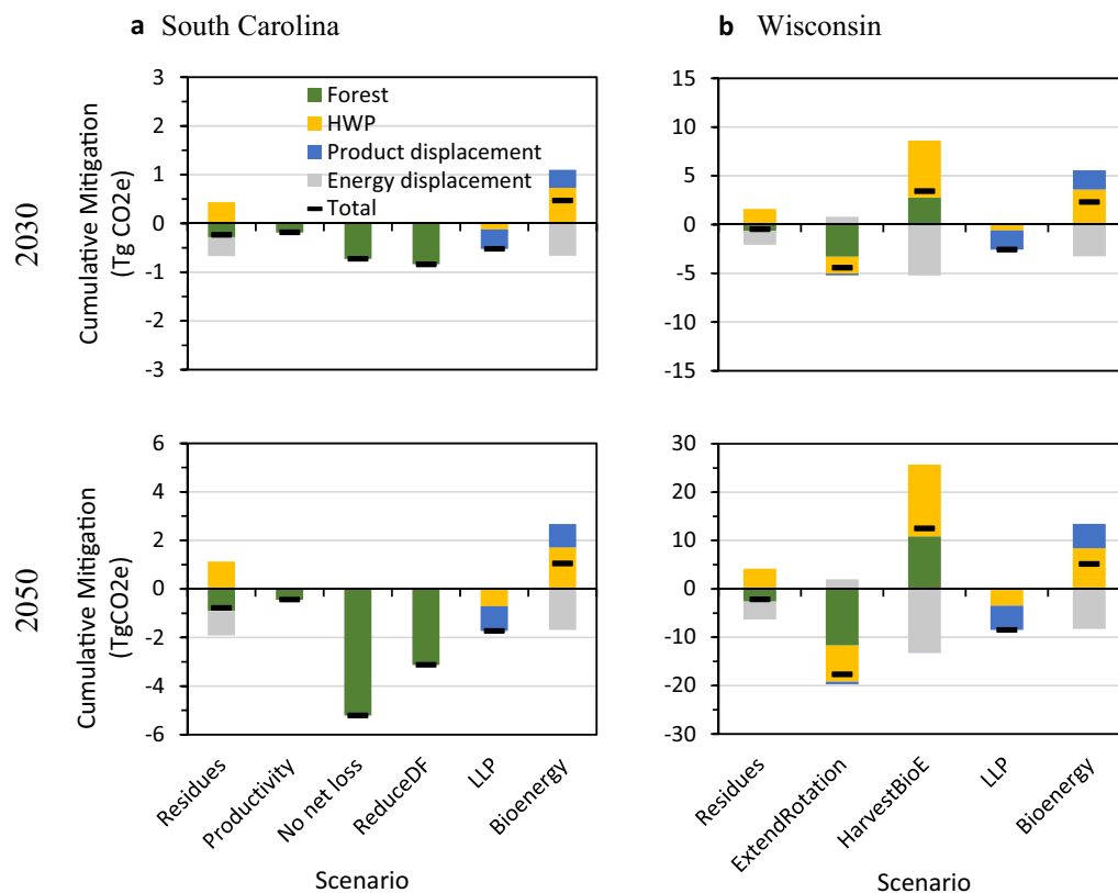
Fig. 7 Cumulative mitigation by component in 2030 and 2050 for the a coastal South Carolina and b Northern Wisconsin study areas. Negative values denote a reduction in GHG emissions
