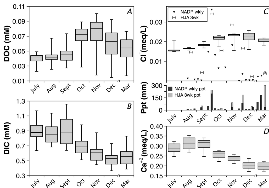
Figure 3. (a) Boxplots of DOC, (b) DIC, (c) \text{Cl}^- , and (d) \text{Ca}^{+2} concentrations in all sampled wells. Whiskers extend to extreme data points and indicate the range. Chloride concentrations in precipitation, and precipitation amounts are also shown in Figure 3c. Precipitation chemistry is from weekly National Atmospheric Deposition Program (NADP) samples and from 3 week bulked samples collected at the PRIME meteorological station at H.J. Andrews Experimental Forest. Symbols were located using the end date for each weekly (NADP) or 3 week (HJA) sampling period.
