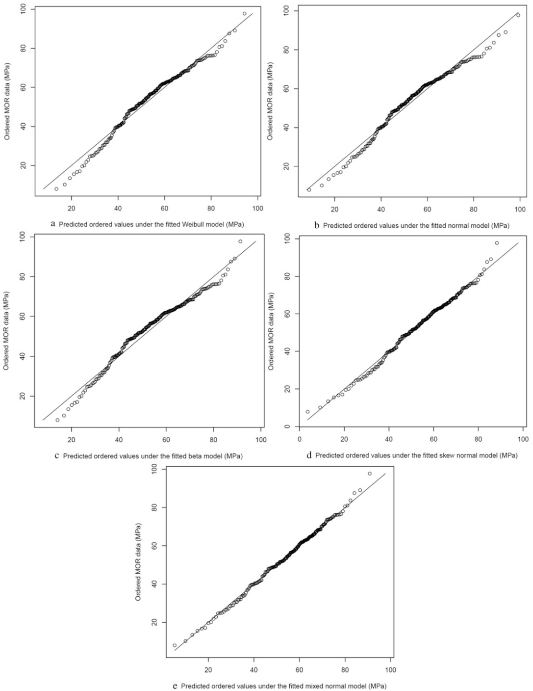
Figure 6. Probability plots of MOR data fitted with two-parameter Weibull, three-parameter Weibull, normal, three-parameter beta, skew normal, and mixed normal distributions. (The best-fit two-parameter Weibull and best-fit three-parameter Weibull are equivalent and represented by the same plot (a) above.) Ordered observed data ( Y axis) plotted against expected scores ( X axis). The reference line y = x indicates perfect fit.
