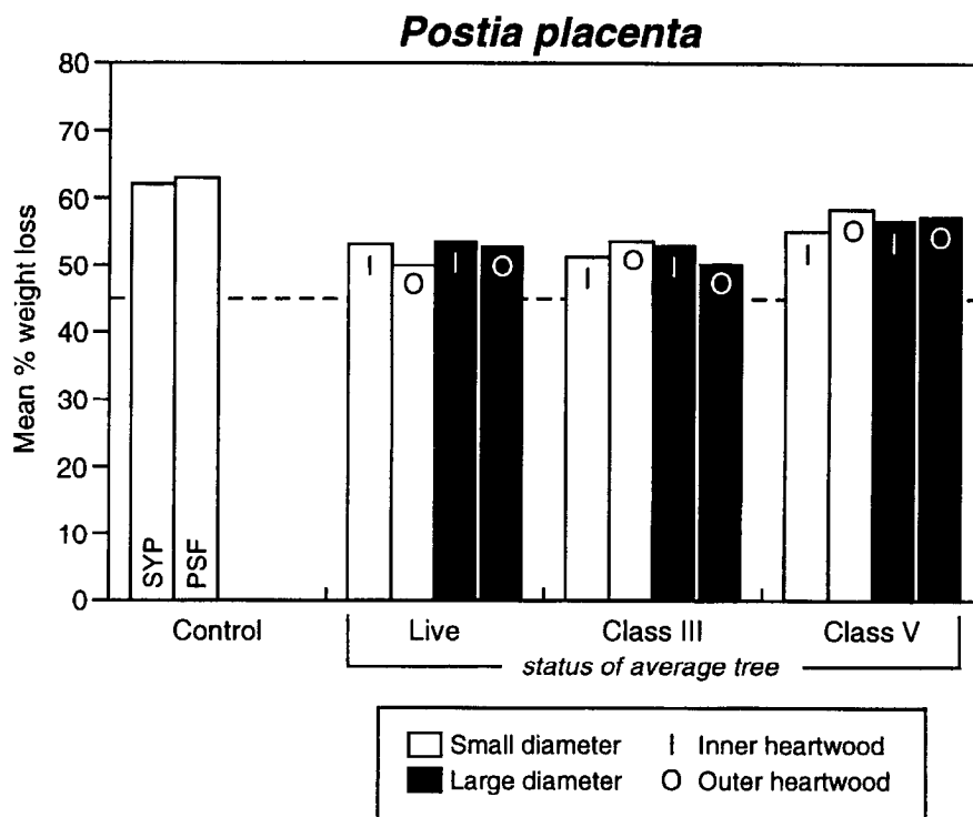
Figure 3. – Mean percentage weight loss caused by P. placenta in heartwood from live and dead trees of yellow-cedar.
