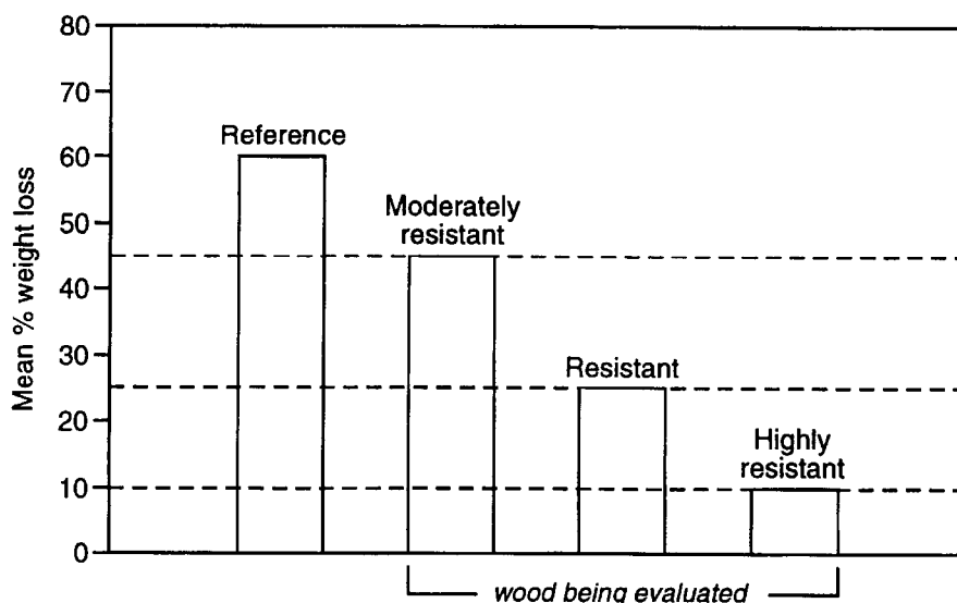
Figure 1. – Classification of natural decay resistance in subject wood when mean weight loss in reference wood has achieved 60 percent (1).
