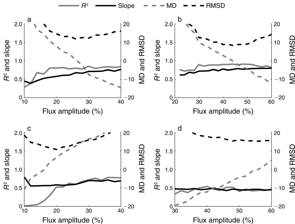
FIG. 6. Four metrics comparing estimates of DOY of (a) start of spring, (b) middle of spring, (c) end of fall, and (d) middle of fall using dates extracted from GCC curve fitting and percentage of maximum GPP. Plots represent 8 GRS site-years. On the left axes, R^2 and slope for geometric mean regression. On right axes, mean deviation (MD) and root mean square deviation (RMSD) of estimates; units are days. DOY 1 is 1 January.
