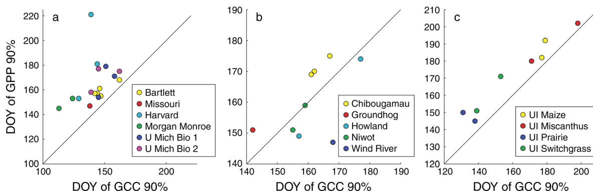
FIG. 5. Comparisons of derived dates (DOY) of maximum greenness and fluxes ( GCC_{90\%} and GPP_{90\%} , respectively) for (a) deciduous broadleaf forest, (b) evergreen needleleaf forest, and (c) grassland/crops sites. DOY 1 is 1 January.
