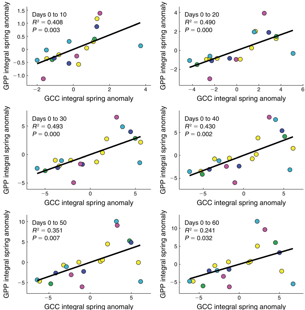
FIG. 8. Regression of GPP integrated sums (dimensionless) vs. GCC integrated sums (dimensionless) during the first 60 days following green-up (shown in 10-day increments) for deciduous broadleaf sites. Legend colors are equivalent to Fig. 5a.
