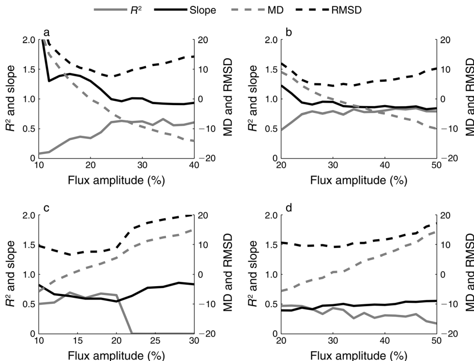
FIG. 4. Four metrics comparing estimates of day of year (see Methods ) for (a) start of spring, (b) middle of spring, and (d) middle of fall using dates extracted from GCC curve fitting and percentage of maximum GPP. The plots represent 19 DBF site-years. (c) End of fall camera dates are derived from date of maximum RCC. On left axes, R^2 (0.0–1.0) and slope for geometric mean regression. On right axes, mean deviation (MD) and root mean square deviation (RMSD) of estimates; units are days.
