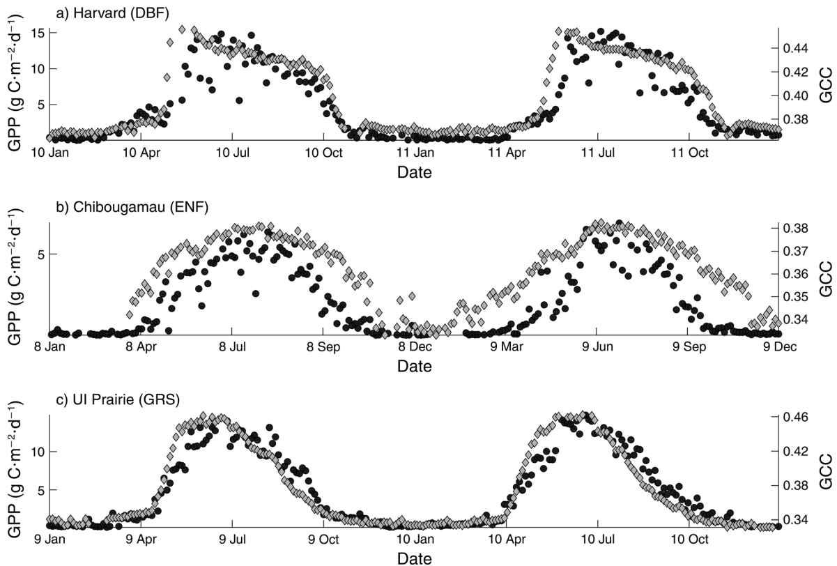
FIG. 2. Time series of daily GPP (black circles, \text{g C}\cdot\text{m}^{-2}\cdot\text{d}^{-1} ) and GCC (green chromatic coordinate, gray diamonds) for (a) deciduous broadleaf forest (DBF); (b) evergreen needleleaf forest (ENF); and (c) grassland/crops (GRS). Two characteristic years of data are featured in each subplot. See Methods for acronyms.
