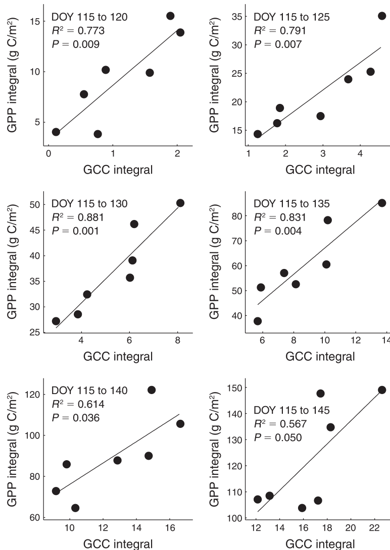
FIG. 7. Regression of GPP integrated sums vs. GCC integrated sums (dimensionless) during the first 30 days following green-up (in 5-day increments) for 2006–2012 at Bartlett.
