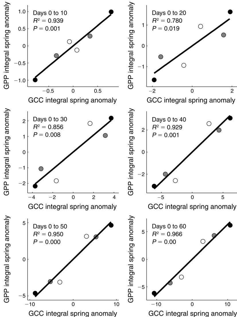
FIG. 9. Regression of normalized GPP integrated sums (dimensionless) vs. GCC integrated sums (dimensionless) during the first 60 days following green-up (in 10-day increments) for the GRS sites, UI Miscanthus (black circles), UI Prairie (white circles) and UI Switchgrass (gray circles).
