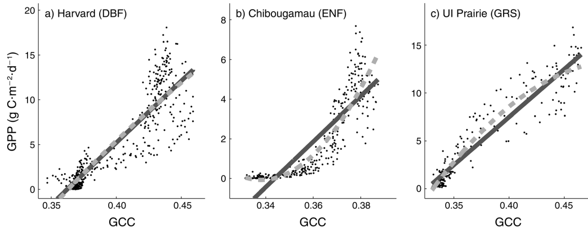
FIG. 3. Scatterplots of daily GPP ( \text{g C}\cdot\text{m}^{-2}\cdot\text{d}^{-1} ) vs. GCC for (a) deciduous broadleaf forest (DBF); (b) evergreen needleleaf forest (ENF); and (c) grassland (GRS). Linear (dark gray) and quadratic regression lines (dashed light gray) are superimposed (see Table 2 for coefficients of determination). All years of data are featured in each subplot.
