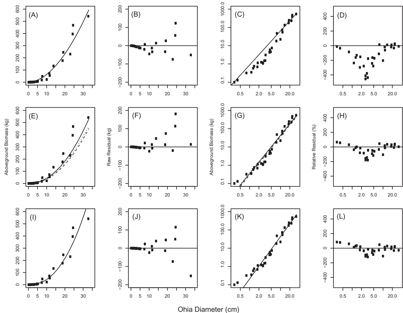
Figure 1. Three fitting techniques for the power-law model architecture of Metrosideros polymorpha . A–D, nonlinear fitting to the untransformed data with the assumption of homoscedastic errors ('method 1' in Table 1), which Packard (2013) argued 'followed the path of the observations'. E–H, linear fitting to the log-transformed diameter and biomass data, followed by back-transformation ('method 2' or the traditional method). The relative residual reflects the fraction (percentage) of the residual compared with the observed value. The dashed line represents the equation Packard (2013) plotted for this fitting technique, for which he excluded the requisite correction factor (i.e. Baskerville, 1972), which is necessary to properly back-transform the error structure with this fitting method. The dotted line represents a generalized linear modelling result offered by Packard as a substitute for the correction factor technique that we originally used. I–L, nonlinear fitting to the untransformed data with the assumption of heteroscedastic errors ('method 3'). Mascaro et al. (2011) considered all three fitting techniques and concluded that methods 2 and 3 (second and third rows) were preferred within the confines of power-law architecture.
