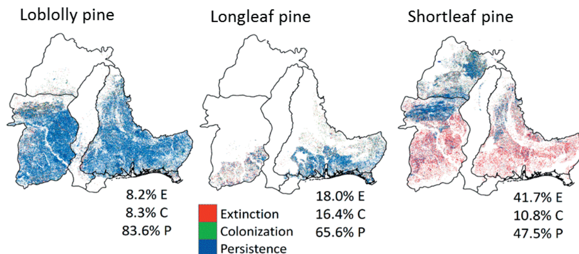
Fig. 2. Predicted changes in (A) tree habitat suitability and (B) tree species occupancy in 2100 without tree harvest, and (C) tree species occupancy in 2100 with tree harvest under climate change in the Gulf Coast Plains and Ozarks region of the southern United States. Changes in habitat suitability are based on early growth and survival of trees simulated by LINKAGES 3.0. Predicted tree species occupancy are based on forest landscape change simulations with LANDIS PRO and include current levels of fire and tree harvest or no tree harvest. Results presented are for the CanESM2 RCP 8.5 scenario, which represented an intermediate level of climate change compared with the other 2 scenarios considered (He and Thompson 2016).
