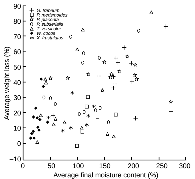
Figure 3—Relationship, by fungus, between average final percentage wood moisture content and average percentage weight loss in blocks. Each entry represents a separate wood species challenged by fungi (identified by a symbol).
