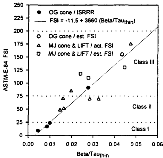
Figure 8. Data of E84-FSI plotted with \beta / \tau_{\text{thin}}
