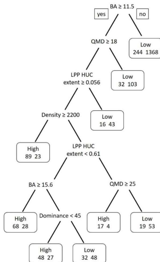
Figure A2. Parsimonious classification tree; misclassification rate 18%. In each box, the left value is the number of incorrectly classified subwatersheds and the right value is the number of correctly classified subwatersheds. Classification tree 1 in Table A1. See Table 1 for variable descriptions.
