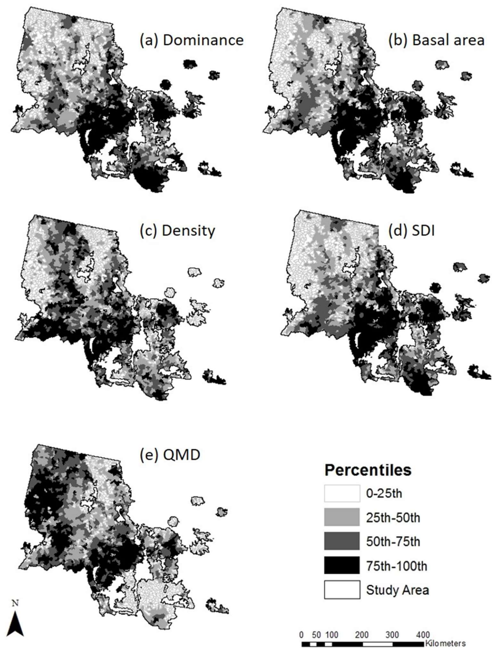
Figure 3. Spatial distribution of subwatershed mean LPP forest parameters by percentile for lodgepole (a) dominance, (b) basal area, (c) density, (d) stand density index and (e) quadratic mean diameter. See Table 1 for variable description.
