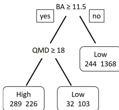
Figure 5. Simplest classification tree; misclassification rate 22%. In each box, the left value is the number of incorrectly classified subwatersheds and the right value is the number of correctly classified subwatersheds. Classification tree 5 in Table A1. See Table 1 for variable descriptions.
