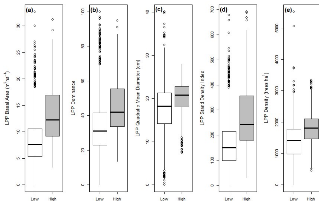
Figure 2. Distribution mean of host characteristics by subwatershed by low and high MPB-attack severity for lodgepole (a) basal area, (b) dominance, (c) quadratic mean diameter, (d) stand density index, and (e) density. See Table 1 for variable descriptions.
