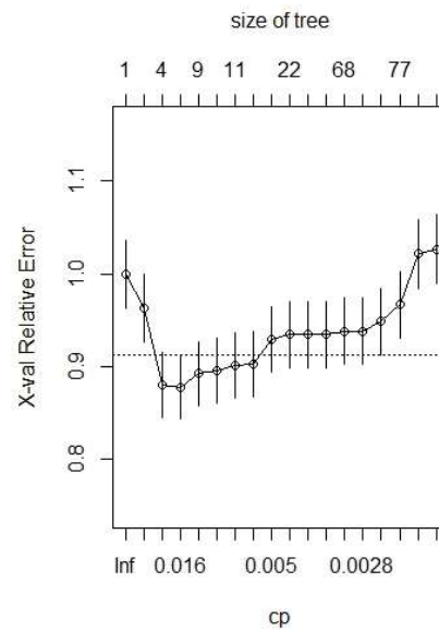
Figure A1. Plot of the cross-validation relative error rate for trees of increasing size (top X-axis) and the corresponding cost-complexity values (bottom X-axis).
