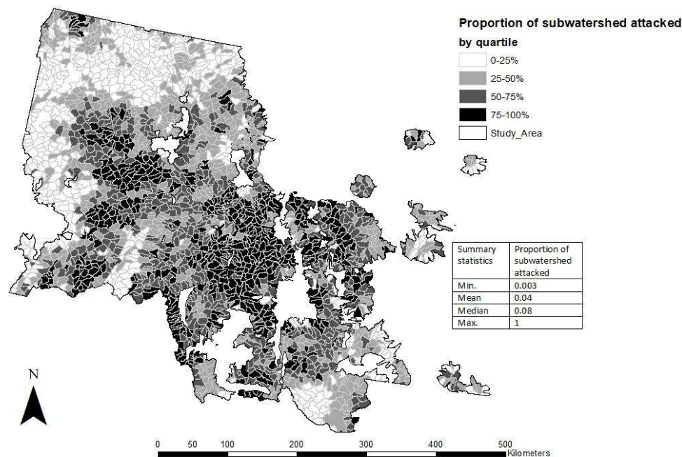
Figure 4. Subwatershed MPB attack severity by quartile, with summary statistics of proportion of area attacked in a subwatershed at high severity.
