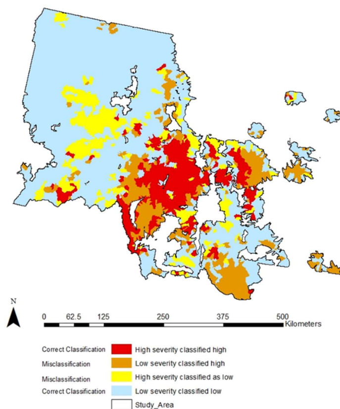
Figure 6. Results of the simplest model for the study area, indicating where subwatershed MPB attack severity was correctly classified and misclassified.
