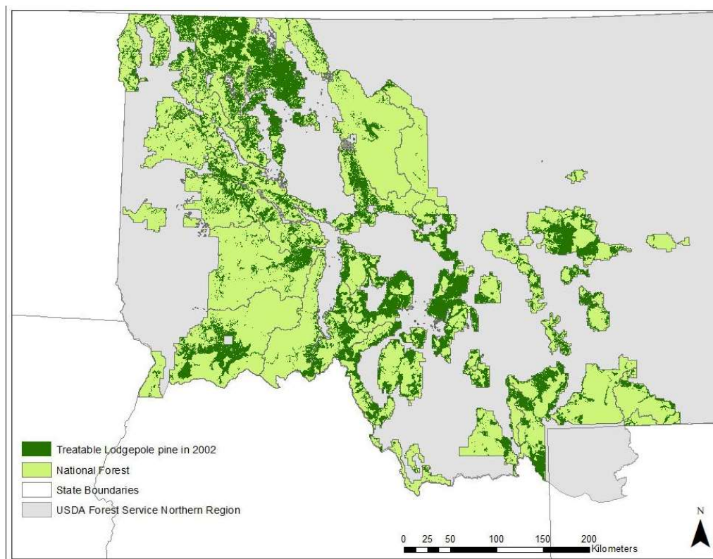
Figure 7. Spatial extent of land in the USDA Forest Service Northern Region in 2002 and the areas with a LPP probability of occurrence greater than or equal to 50% where tree removal is not prohibited by legal constraints.
