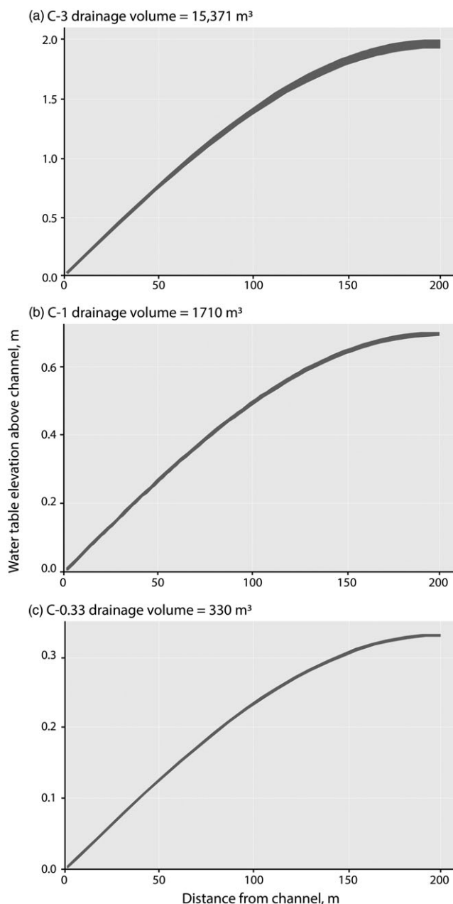
FIGURE 6 Drainage curves produced from Equation 12 for (a) 3-m incised scenario (C-3), (b) 1-m incised scenario (C-1), and (c) 0.33 m incised or “restored” scenario (C-0.33). Top of the curve shows position of water table at t_1 , bottom of curve shows position of water table at t_c . Note differences in scale of Y axis and considerable vertical exaggeration
