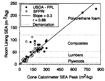
Figure 8 Prediction of lining SEA from SEA peak of cone calorimeter tests of horizontal specimen at 35 \text{ kW/m}^2
