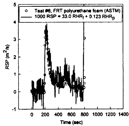
Figure 3 Correlation of RSP with RHR for Test #6
