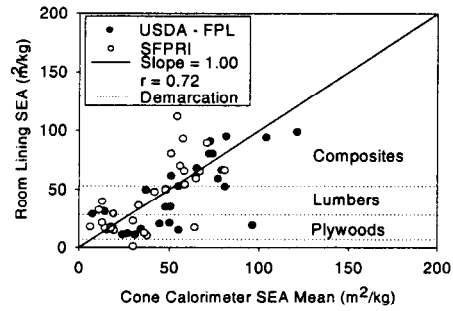
Figure 7 Correlation of lining SEA with SEA mean of cone calorimeter tests of horizontal specimen at 35 \text{ kW/m}^2
