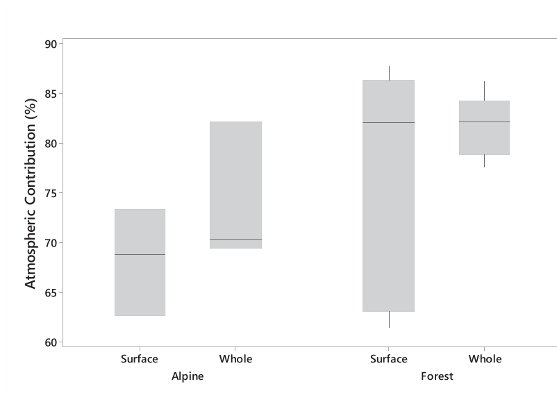
Fig. 6. Atmospheric deposition contribution to Fraser Experimental Forest summit soils associated with alpine ( n = 3 ) and forest vegetation ( n = 5 ). Box plots show depth-weighted median mass transfer function values (horizontal line), middle 50% (box), and upper and lower 25% (bars). There were no outliers to report. Surface = surface mineral horizon; Whole = whole soil profiles.
