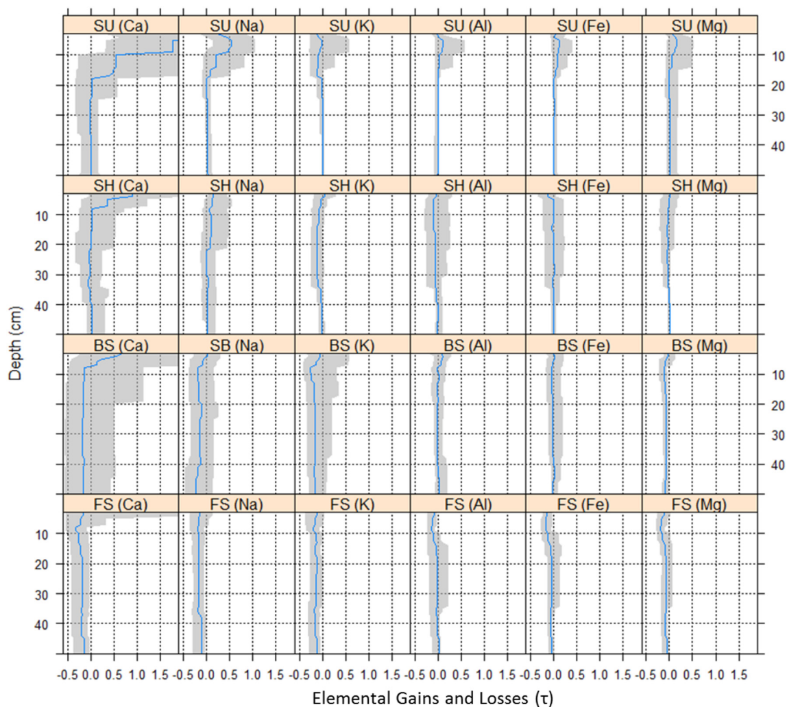
Fig. 3. Elemental gains and losses for soil profiles by landscape position the Fraser Experimental Forest, Colorado, by landscape position ( n = 8 ). Plots show the mean tau for each respective cation (blue line) bounded by the 25th and 75th percentiles of each value at depth. SU = summit; SH = shoulder; BS = backslope; FS = footslope. (For interpretation of the references to color in this figure legend, the reader is referred to the web version of this article.)
