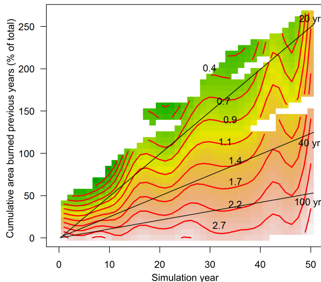
Fig. 7. Contour plot of expected area burned in the current year (% total) conditional on simulation year and cumulative area burned in all previous years. Black lines show reference fire rotation intervals, or number of years to burn an area equal to the entire study area. The average area burned per year for all simulations was 2.2% or a fire rotation of about 45 years. Contours show a 10-year periodicity that corresponds to the modeled vegetation regrowth after fires.
