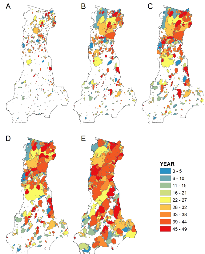
Fig. 3. Simulated fire perimeters in the study area from one 50-year Envision simulation for five wildfire scenarios: 1X (A), 2X (B), 3X (C), 4X (D), and 10X (E). Increased levels of wildfire activity in each scenario were achieved by multiplying the burn period of each ignition over contemporary levels by the multiplier indicated.
