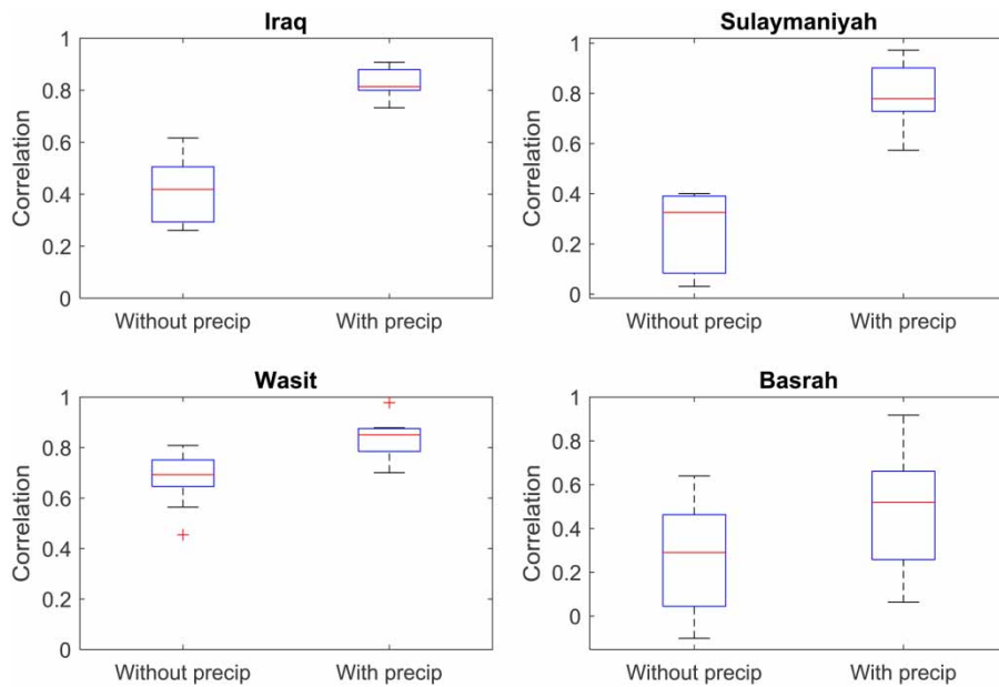
Figure 3 | Correlations between composite period NDVI values and modified modelled GSI values over ten years (2001-2010) for whole study area (Iraq) and for test sites (Sulaymaniyah, Wasit, and Basrah). All correlations were significant ( P value < 0.001 ).
