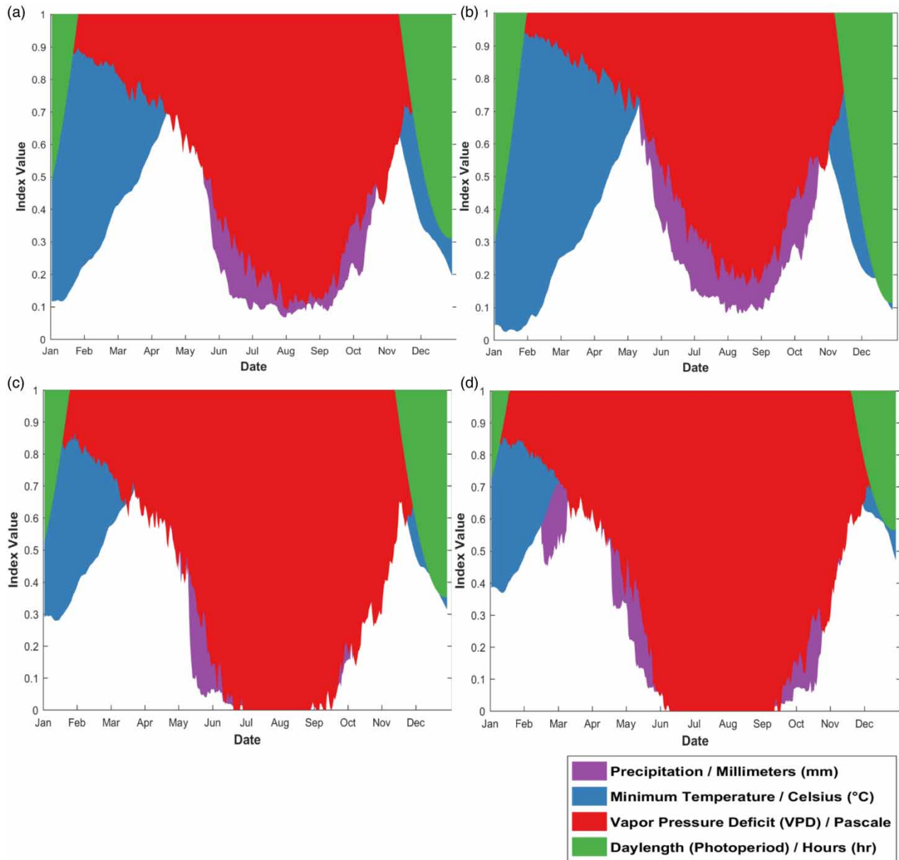
Figure 4 | The seasonal index values for minimum temperature, vapour pressure deficit, precipitation and photoperiod for whole study area for Iraq (a), Sulaymaniyah (b), Wasit (c), and Basrah (d), showing the seasonal limits of each variable for ten-year average. Indices are presented as a 21-day running average to better depict seasonal trends.
