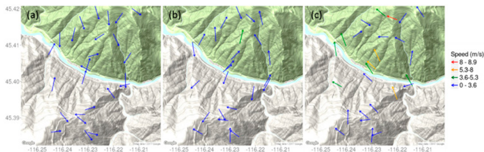
Figure 2. (a) Downslope winds at 0100 LT on 11 August 2011; (b) upslope winds at 1100 LT on 11 August 2011; and (c) gap winds at 1000 LT on 17 August 2011.
