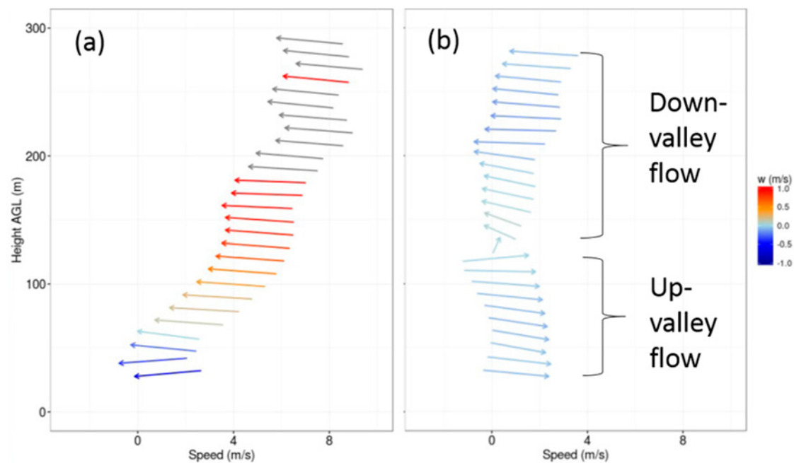
Figure 5. Vertical profiles of wind speed at 0900 LT measured by a sodar located at river level during: (a) a gap wind event on 17 August; and (b) a non-event day on 18 August. The arrows are centered on the average speed measured at each height AGL. The direction of the arrow indicates the direction of the horizontal wind; arrows pointing left indicate wind from the east (downvalley wind). The arrow color indicates the w-component of the wind.
