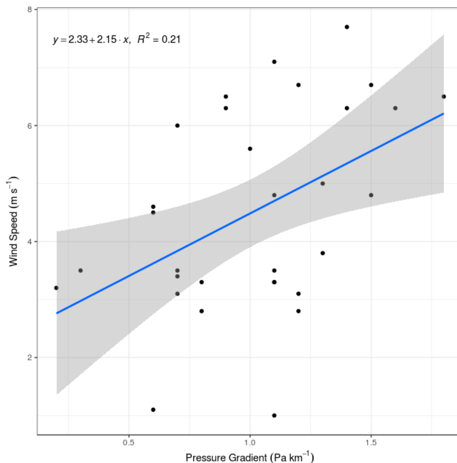
Figure 3. Relationship between the mean sea level pressure gradient at 0600 LT and wind speed at sensor NM3 at 0900 LT. Gray shading indicates the 95% confidence interval.
