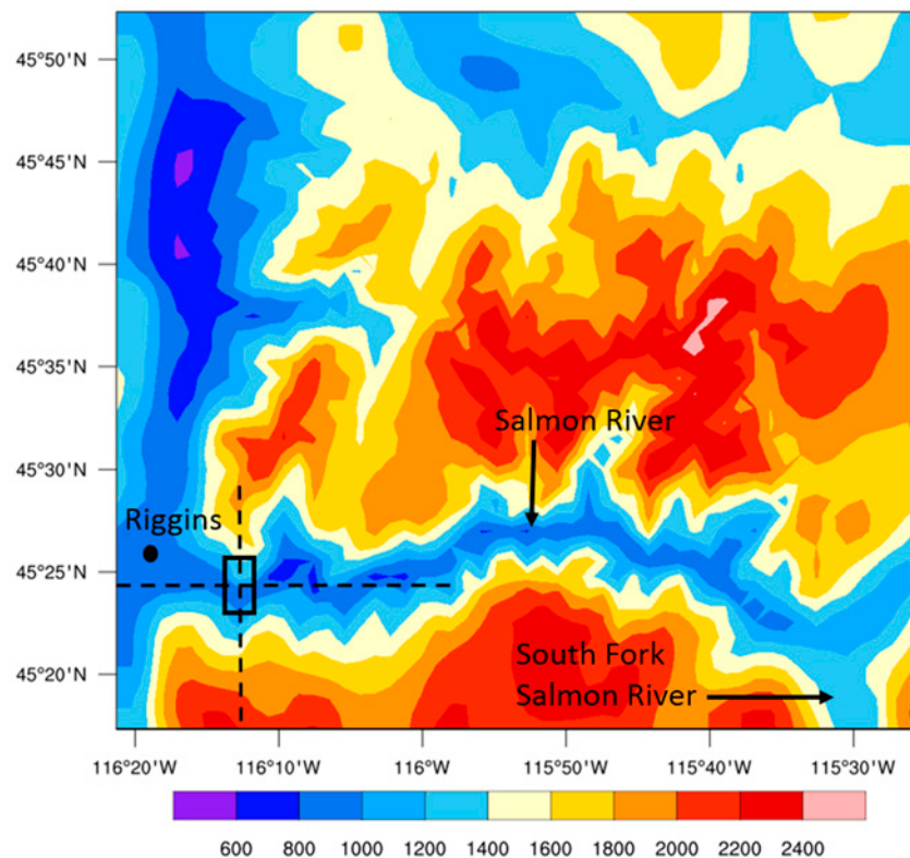
Figure 8. WRF 1.33 km domain with major geographical features and the study area labeled. Colors indicate terrain height in meters in the GMTED10 digital elevation model used for the simulations. The dashed black lines indicate transects along which vertical profiles are extracted for analysis.
