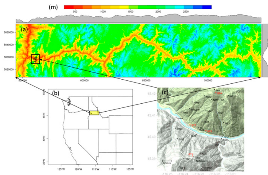
Figure 1. Study area and surrounding terrain. (a) Digital elevation model of the Salmon River Canyon and surrounding terrain; the small black crosses indicate wind sensor locations. (b) Geographic location of the Salmon River Canyon; the yellow box denotes the location Salmon River Canyon; the black circle indicates the study area. (c) Hillshade of the study area with wind sensor locations.
