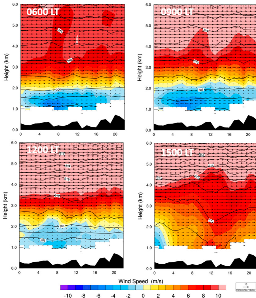
Figure 10. Along-valley vertical profiles of wind and potential temperature simulated in the 1.33 km domain for event day 17 August. Wind vectors indicate wind in the x - z plane. Wind speed is the u -component of the wind; negative values indicate easterly flow. The study area is located in cells 7–10 on the x -axis. Only the lowest 6 km are shown.
