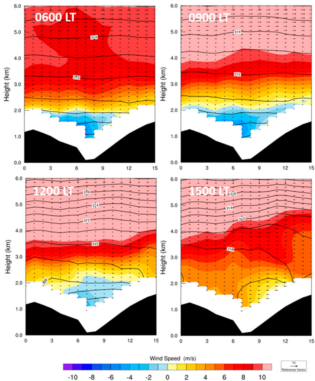
Figure 11. Cross-valley vertical profiles of wind and potential temperature simulated in the 1.33 km domain for event day 17 August. Wind vectors indicate wind in the y - z plane. Wind speed is the u -component of the wind; negative values indicate easterly flow. Into the page is west with the north canyon wall on the right. Only the lowest 6 km are shown.
