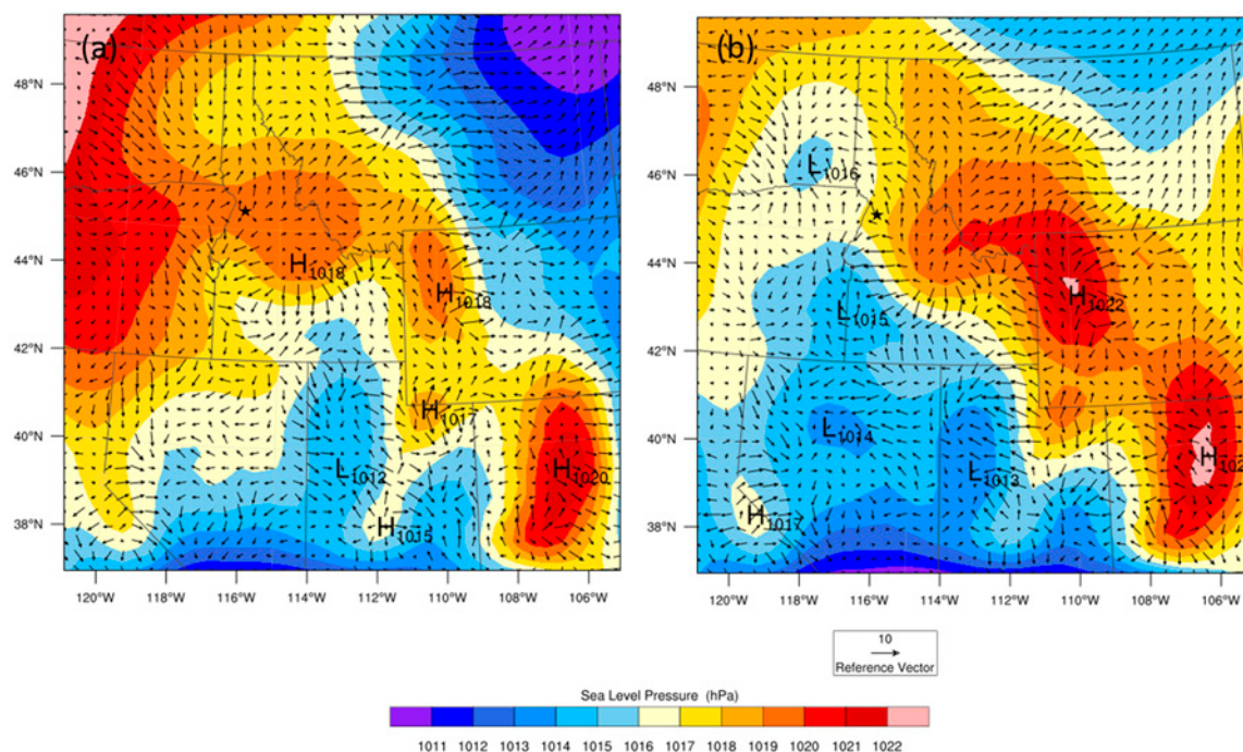
Figure 7. Mean sea level pressure and 10-m winds simulated in the 36 km domain at 0600 LT on: (a) non-event day 18 August; and (b) event day 17 August. The study area is indicated with a star.
