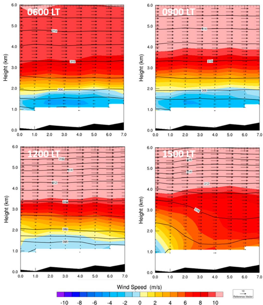
Figure 14. Along-valley vertical profiles of wind and potential temperature simulated in the 4 km domain for event day 17 August. Wind vectors indicate wind in the x - z plane. Wind speed is the u -component of the wind; negative values indicate easterly flow. Only the lowest 6 km are shown.
