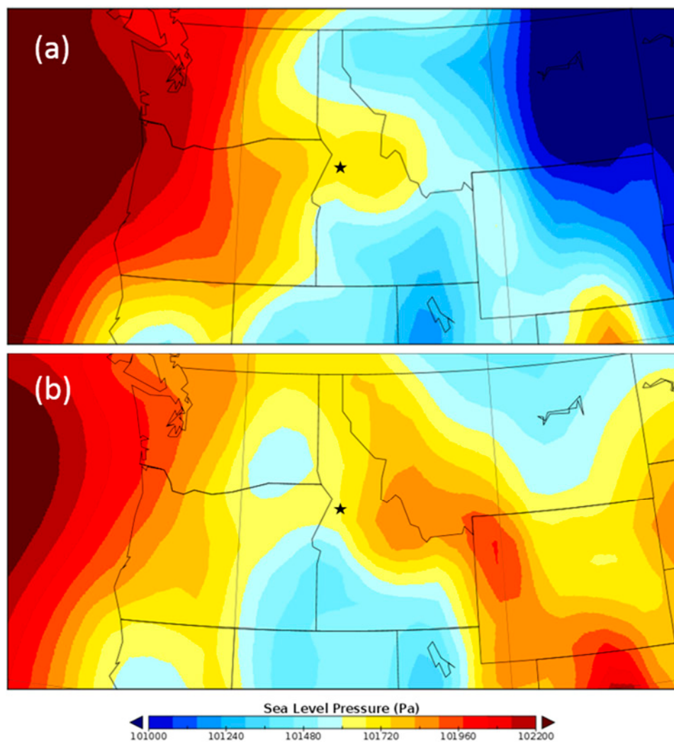
Figure 6. ERA-Interim sea level pressure analysis for 0600 LT on: (a) non-event day 18 August; and (b) event day 17 August. The study area is indicated with a star.
