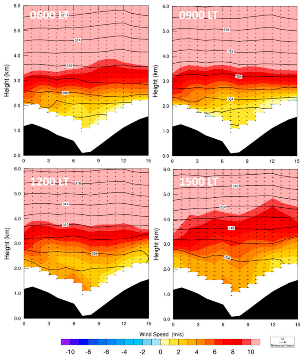
Figure 13. Cross-valley vertical profiles of wind and potential temperature simulated in the 1.33 km domain for non-event day 18 August. Wind vectors indicate wind in the y - z plane. Wind speed is the u -component of the wind; negative values indicate easterly flow. Into the page is west with the north canyon wall on the right. Only the lowest 6 km are shown.
