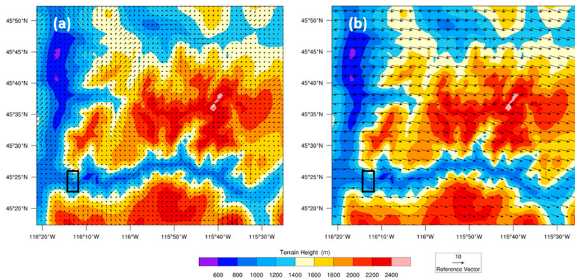
Figure 9. Simulated: (a) 10-m winds; and (b) 700-mb winds in the 1.33 km domain at 0900 LT on event day 17 August. The black box delineates the study area.
