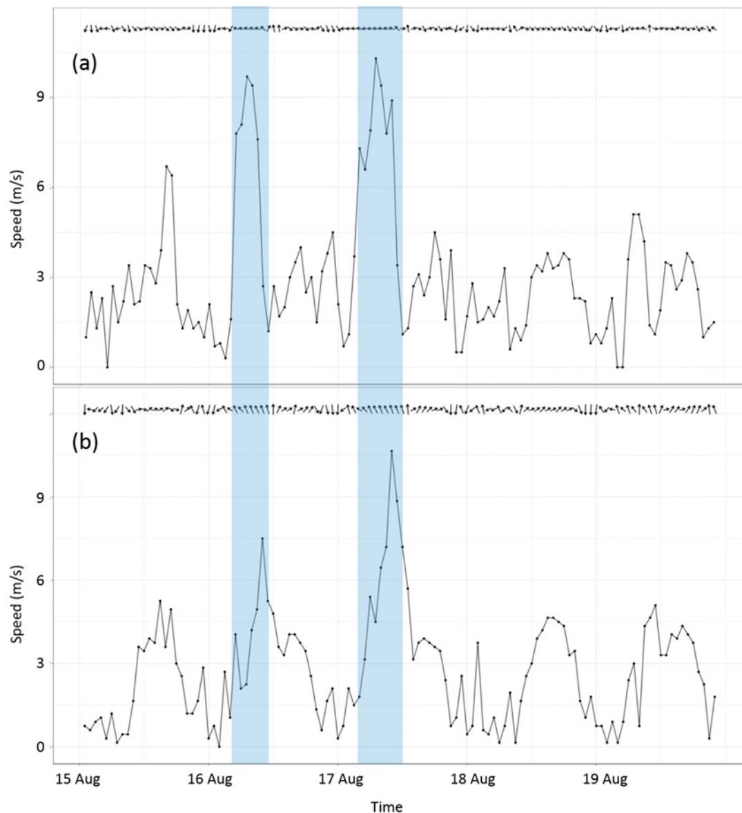
Figure 4. The 10-min average winds observed at the top of each hour at sensor: (a) NM1; and (b) NM3. The blue shading highlights two gap wind events.
