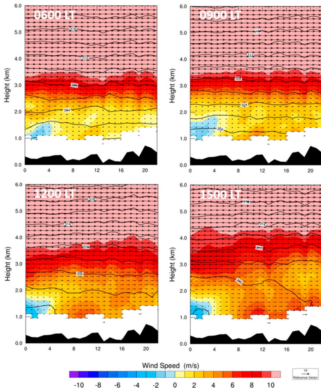
Figure 12. Along-valley vertical profiles of wind and potential temperature simulated in the 1.33 km domain for non-event day 18 August. Wind vectors indicate wind in the x - z plane. Wind speed is the u -component of the wind; negative values indicate easterly flow. The study area is located in cells 7–10 on the x -axis. Only the lowest 6 km are shown.
