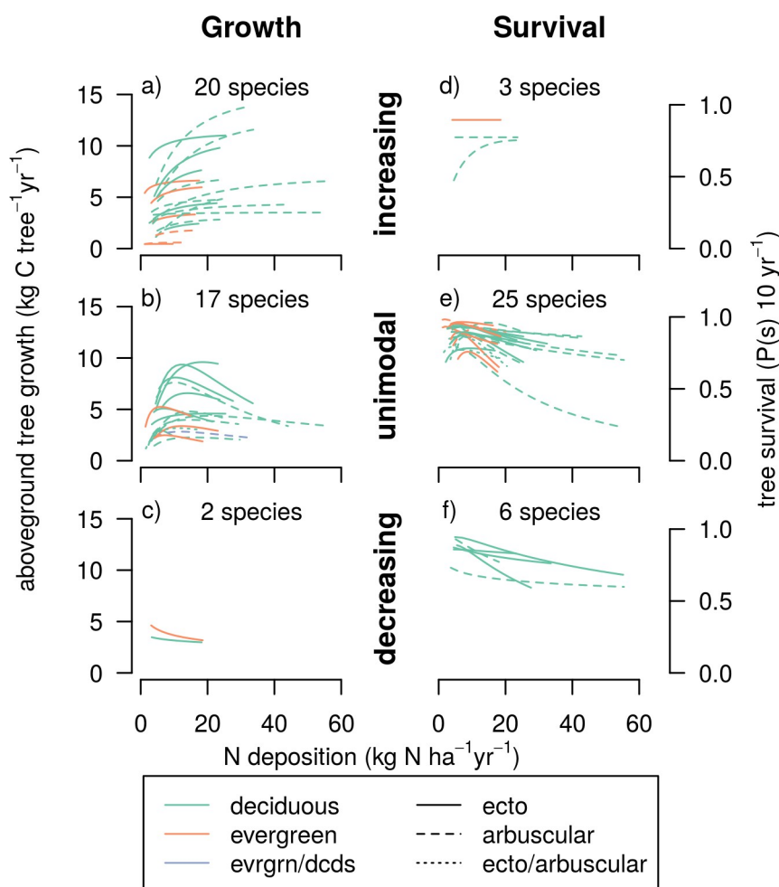
Fig 2. Tree growth and survival versus N deposition by species and colored by ecological attributes. Each curve represents the average tree growth (a-c) or survival (d-f) across the N deposition gradient for a single species. The relationships are separated by general curve shape; The (a,d) increasing, (b,e) unimodal, and (c,f) decreasing relationships with N deposition are shown. (For individual species and growth and survival curves by species and the curves associated with S deposition see S1 Fig). Note that two of the five species in panel d are functionally flat (< 0.01% change over deposition range) and are classified as flat in Table 1.
