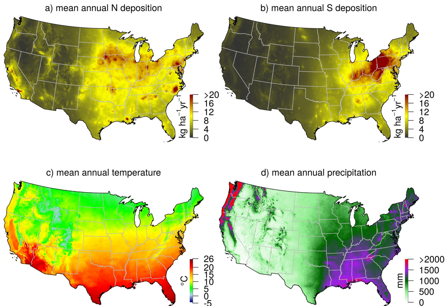
Fig 1. Gradients of N deposition, S deposition, mean annual temperature, and mean annual precipitation across the conterminous U.S. Panels are the a) mean total N deposition from 2000–2012, b) mean total S deposition from 2000–2012, c) mean annual temperature from 2000–2014, and d) mean annual precipitation from 2000–2014. Deposition data are from the TDEP product [23] and climate data are from PRISM ( http://prism.oregonstate.edu ). The averages for each tree in the analysis were a subset of these datasets that coincided with its measurement interval. The values used in the species-level empirical models correspond to the spatial distribution of the species.
