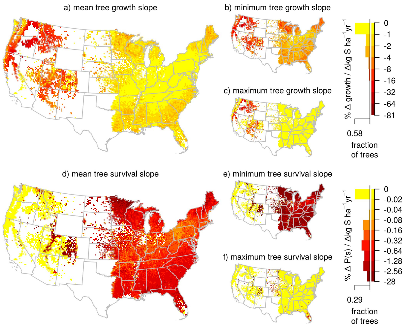
Fig 4. Relative change in growth and survival with S deposition of individual trees across the conterminous U.S. Maps show the relative mean, minimum, and maximum growth (a-c) and survival (d-f) responsiveness (percent change in growth or survival per change in annual S deposition rate) of trees within each 20 x 20 km pixel. Values were derived from the instantaneous rate of change in growth or survival with S deposition of the most parsimonious, species-specific models that allowed both N and S deposition (but did not necessarily contain N or S deposition). Red areas indicate where small increases in S deposition are associated with relatively large decreases in growth or survival. White areas are where no tree growth or survival data were available. Histograms indicate the fraction of individual trees by responsiveness to N deposition. Sample size for growth was 1,183,931 trees and for survival was 1,423,455 trees.
