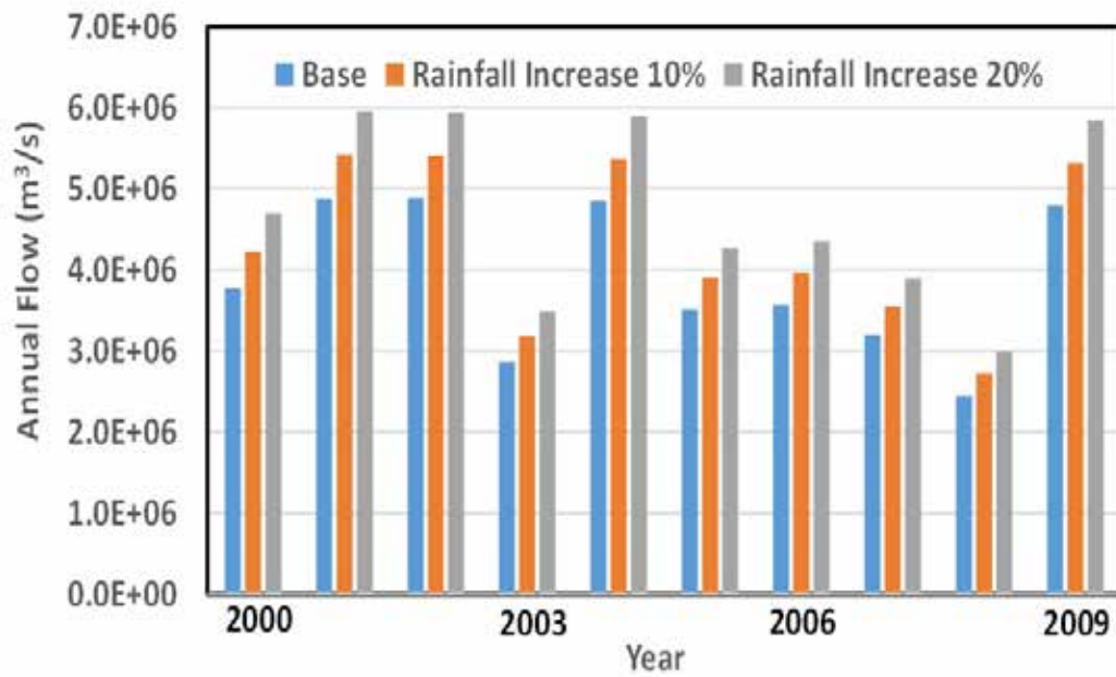
Figure 4. Annual stream discharge as rainfall rate increased.
