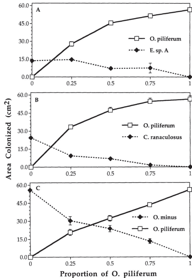
FIG. 1. De Wit replacement series. A. Mean area (with standard error bars) of malt extract agar colonized by O. piliferum and A. E. sp. A 2 wk after inoculation. B. C. ranaculosus 1 wk after inoculation. C. O. minus 1 wk after inoculation. In the absence of differential competition an “x” shaped pattern is seen, with the area colonized by both species directly proportional to the proportion of each species in the initial population.
