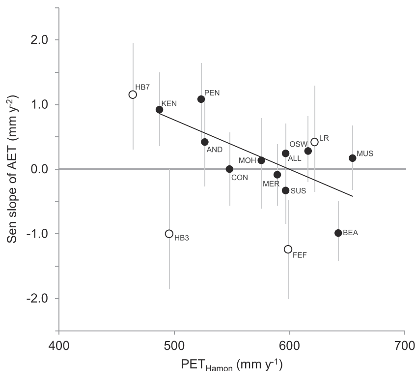
FIGURE 3 The observed trend in AET inferred from water balance is related to mean annual PET. Open circles represent the small watersheds; filled circles represent river basins. Watershed abbreviations follow Tables 1 and 2. Only small watersheds with >45 years of data are included here. Trends are expressed using Sen's monotonic slope estimate and shown with 95% confidence intervals; trends with confidence intervals not overlapping the zero line are significant at \alpha = 0.05 . The regression line shown, for the large watersheds only, has a slope of -0.0076 and an intercept of 4.6 \text{ mm year}^{-2} . AET: actual evapotranspiration; PET: potential evapotranspiration
