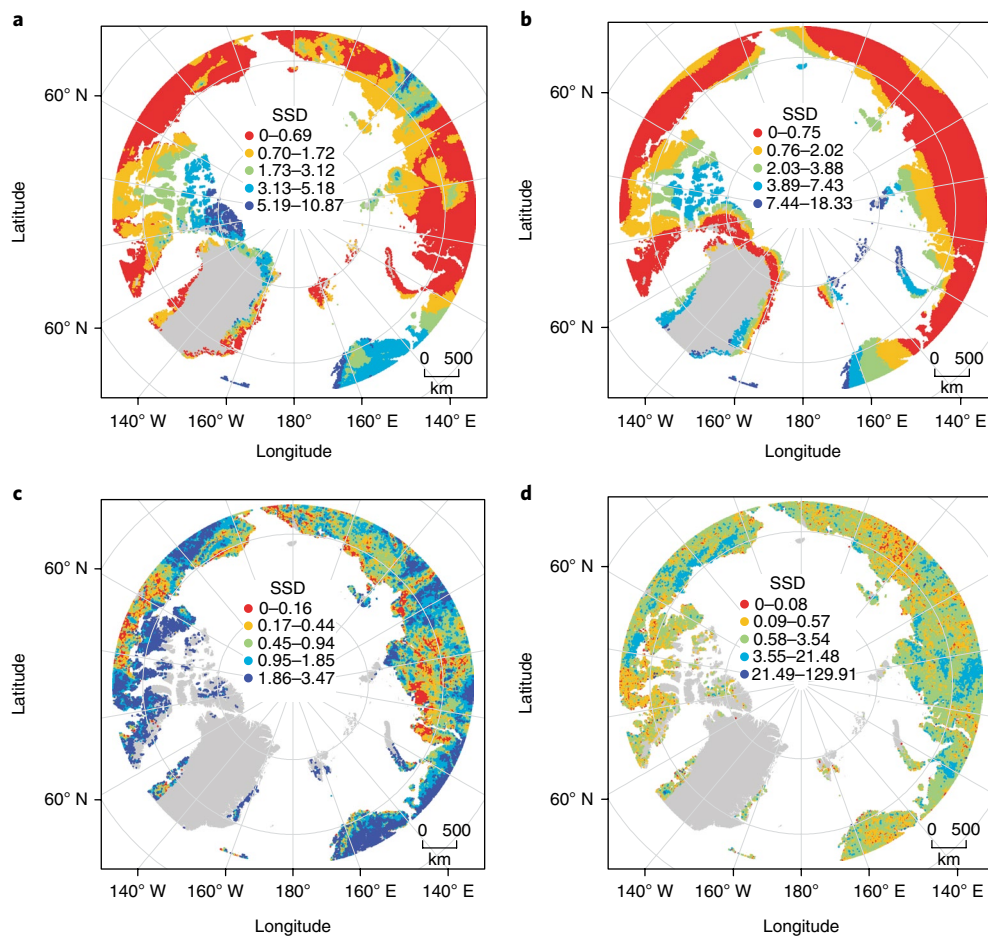
Fig. 3 | Differences between sampled conditions and actual conditions. a–d, Similarity between conditions at sampled locations and actual conditions of MAT ( a ), \Delta MAT ( b ), fAPAR ( c ) and \Delta fAPAR ( d ) within terrestrial ecosystems above the Arctic Circle. The smaller the sum of squared differences (SSD), the greater the similarity between conditions at sampled locations and actual conditions at every pixel. Areas with permanent ice cover (for example, the interior of Greenland and portions of the Canadian archipelago) are shaded grey and were not included in the analysis.
