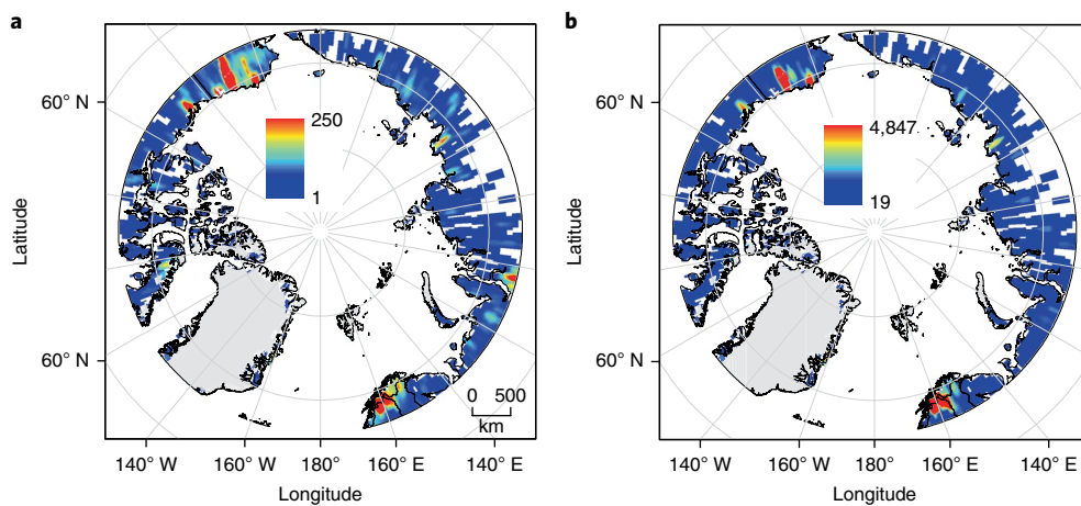
Fig. 1 | Sampling location and citation density. a,b , Density of field sampling locations ( a ) and citations ( b ) per unit land area (km 2 ) from environmental research above the Arctic Circle. The spatial resolution is 1°. Areas with permanent ice cover (for example, the interior of Greenland and portions of the Canadian archipelago) are shaded grey and were not included in the analysis. Areas in white have no locations or citations.
