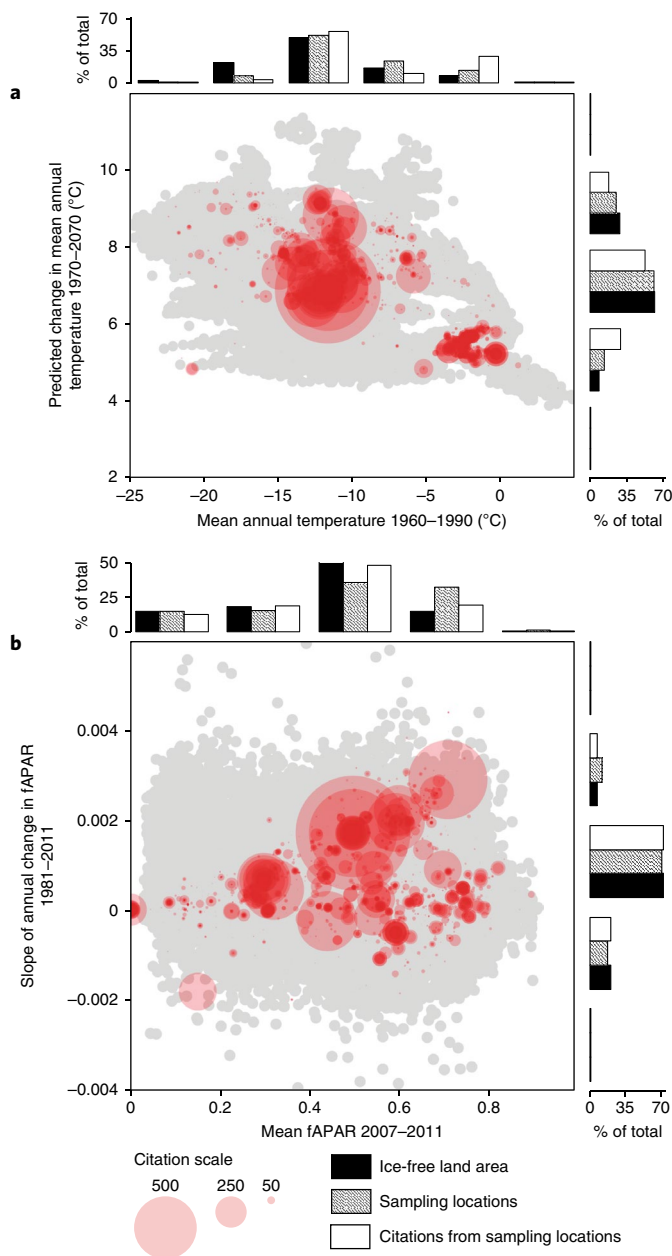
Fig. 2 | Distribution of research citations for MAT versus \Delta MAT and fAPAR versus \Delta fAPAR. a,b , Distribution of research citations with natural variation in MAT versus \Delta MAT ( a ) and fAPAR versus \Delta fAPAR ( b ) within terrestrial ecosystems above the Arctic Circle. Each red circle denotes a study sampling location (6,246 in total). The circle diameter indicates the number of corrected citations for each sampling location (the number of corrected citations is the study citation number divided by the number of locations within the study). Grey circles denote conditions extracted from every pixel above the Arctic Circle. The bar graphs denote the portion of ice-free land area (black bars), number of research sampling locations (hatched bars) and number of citations from locations (white bars) covered by each bioclimatic zone above the Arctic Circle.
