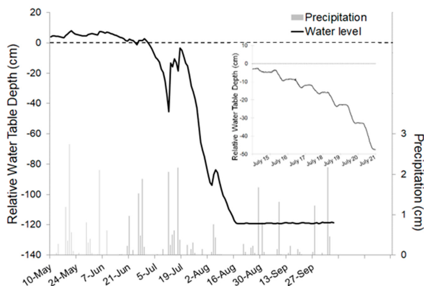
Figure 3. Water table hydrograph for a black ash wetland in northern Minnesota (classified as WFn64 based on Aaseng et al. [25]). Water tables are above the soil surface following spring snowmelt, and then rapidly drawdown once black ash leaf expansion occurs (usually in mid-June). The influence of black ash transpiration on this pattern is readily apparent in the diurnal water table pattern once water tables are below the soil surface (inset).
