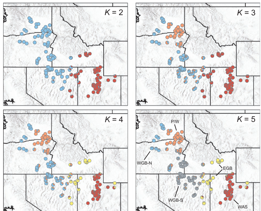
FIGURE 4 Results of STRUCTURE analyses for K = 2 to K = 5 . The posterior probabilities of individual assignments are averaged within sampling localities and represented by pie charts. Populations discussed in the text are noted for K = 5 and include Palouse/Wallowa (P/W); Western Great Basin (WGB-North and WGB-South); Eastern Great Basin (EGB); and Wasatch (WAS)
