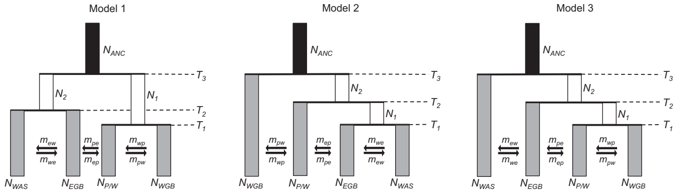
FIGURE 2 Schematics of FASTSIMCOAL2 modeling scenarios. All italicized labels represent estimated parameters, except for the ancestral effective population size ( N_{ANC} ), which was set to 60,000 (see Methods). The rate of migration ( m ) is assumed to be directionally the same between population pairs. Each model has the same parameter values, though they vary in their order and/or representation. To crosswalk to K = 4 in Figure 4: N_{WAS} = Wasatch sampling localities (red); N_{EGB} = Eastern Great Basin (yellow); N_{P/W} = Palouse/Wallowa (orange); and N_{WGB} = Western Great Basin (blue)
