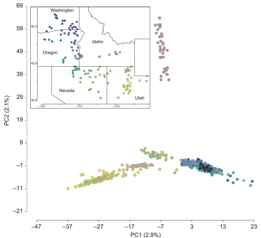
FIGURE 3 Distribution of diploid Pseudoroegneria spicata individuals along principal component 1 and principal component 2 axes of genetic variation. Variation explained by the axes is given in parentheses. Individuals in PC space are colored by their sampling locations, which are displayed in the inset (see also Figure 1). Individuals colored black represent the commercial germplasm sources. Colors in this figure do not correlate to colors that describe populations (i.e., Figures 4 and 5)
