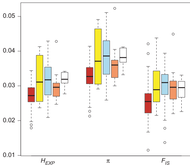
FIGURE 5 Comparison of genetic diversity statistics across populations identified in the K = 4 STRUCTURE analysis (red—WAS, yellow—EGB, blue—WGB, and orange—P/W; see Figures 1 and 4 for population definitions). The white box-and-whisker plots represent the commercial germplasm sources. For each summary statistic ( H_{EXP} , expected heterozygosity; \pi , nucleotide diversity; F_{IS} , inbreeding coefficient), the median, first and third quantiles, standard deviation, and range across populations are shown
