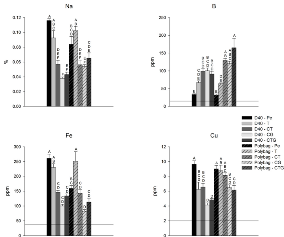
Figure 3. Foliar nutrient concentrations of Hispaniolan pine seedlings across interacting container and growing media treatment levels where significant ( \alpha = 0.05 ). Horizontal lines indicate normal nutrient levels reported for Pinus strobus from http://agsci.psu.edu/aasl/plant-analysis/plant-tissue-total-analysis/interpretive-nutrient-levels-for-plant-analysis/pine-white (accessed 2 February 2018).
