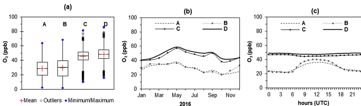
Fig. 3. Variability of hourly O 3 concentrations (ppb): (a) mean annual data, (b) mean monthly data, and (c) diurnal variation at different altitudes (A, B, C, D) over 2016.
