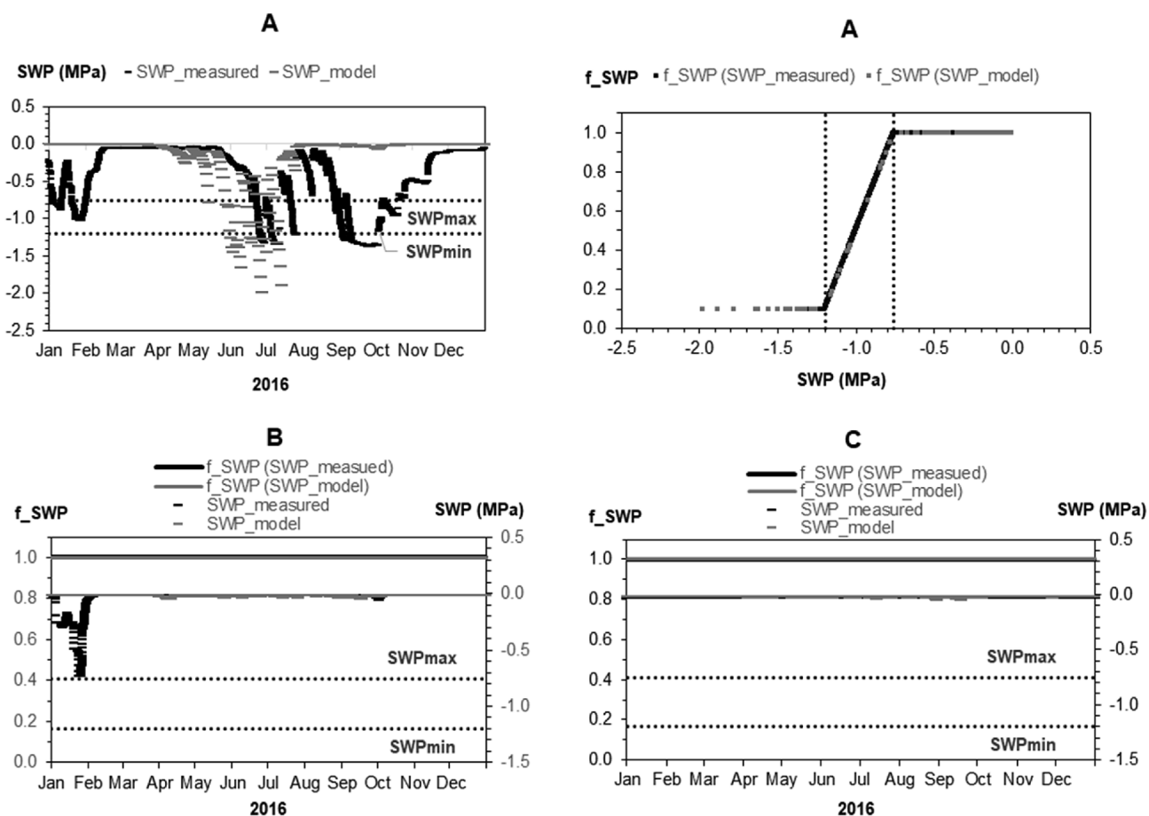
Fig. 5. Soil water potential (SWP, MPa) and factor f_{SWP} (Eq. (7)): comparison between measured and modelled values for different altitudes (A, B, and C) in 2016; dotted lines illustrate SWP ranges for effective stomatal O_3 conductance (Table S1). Stomatal conductance calculated by the DO_3SE (Eq. (1)) and site-specific model (Eq. (8)) were compared at three study sites (A, B, and C).
