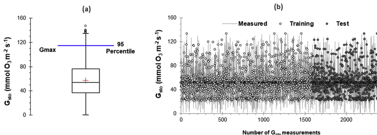
Fig. 2. Stomatal conductance ( G_{\text{sto}} ) for dwarf mountain pine in SK-HT: (a) box plot of measured data and the derived parameter G_{\max} ; (b) comparison of G_{\text{sto}} measured by Licor6400XT and tested by a site-specific regression function (Eq. (8)).
