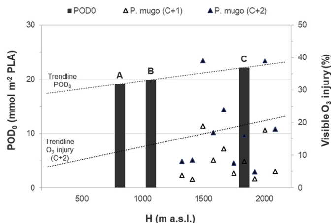
Fig. 7. POD 0 at different altitudes (A, B, C) and percentage of visible O 3 symptoms on needles of different age (C+1, C+2) for dwarf mountain pine in the SK–HT.
