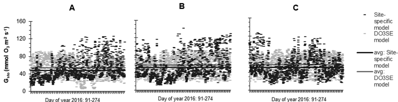
Fig. 6. Stomatal conductance ( G_{sto} ; mmol O_3 m^{-2} s^{-1} ) according to the DO_3SE (Eq. (1)) and site-specific model (Eq. (8)) estimated for selected meteorological conditions (AT above 9^\circ C and PAR above 150 \mu mol m^{-2} s^{-1} from April 1st to September 30th (DOY 91–274) for dwarf mountain pine at three study sites (A, B, and C) in SK-HT.
