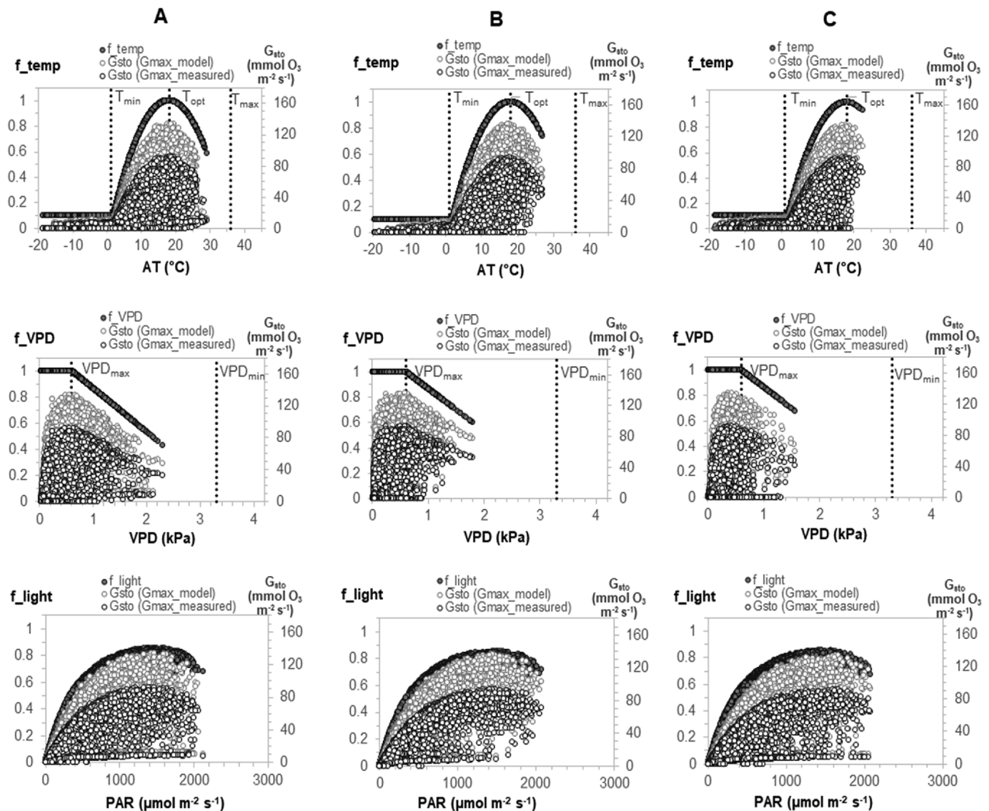
Fig. 4. Air temperature (AT, deg. C), vapour pressure deficit (VPD, kPa), and photosynthetically-active radiation (PAR, \mu\text{mol m}^{-2} \text{s}^{-1} ) in relation to environmental factors ( f_{\text{temp}} , f_{\text{VPD}} , and f_{\text{light}} ) and model results for G_{\text{sto}} ( \text{mmol O}_3 \text{m}^{-2} \text{s}^{-1} ) according to the G_{\text{max}} parameter as a pre-set value in model ( G_{\text{sto}}:G_{\text{max\_model}} ) and field measurement in local conditions ( G_{\text{sto}}:G_{\text{max\_measured}} ) for different altitudes (A, B, and C); dotted vertical lines depict the variable ranges (AT, VPD) for effective stomatal \text{O}_3 conductance (Table S1).
