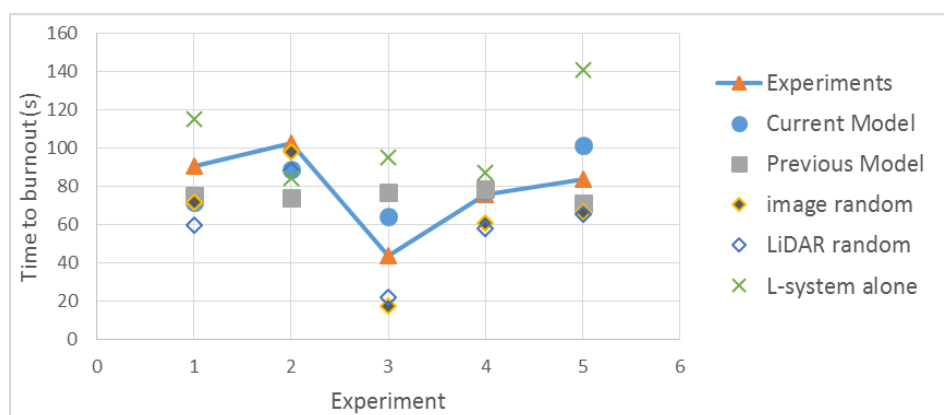
Figure 3 - Time to burnout comparison of model simulations for chamise.
