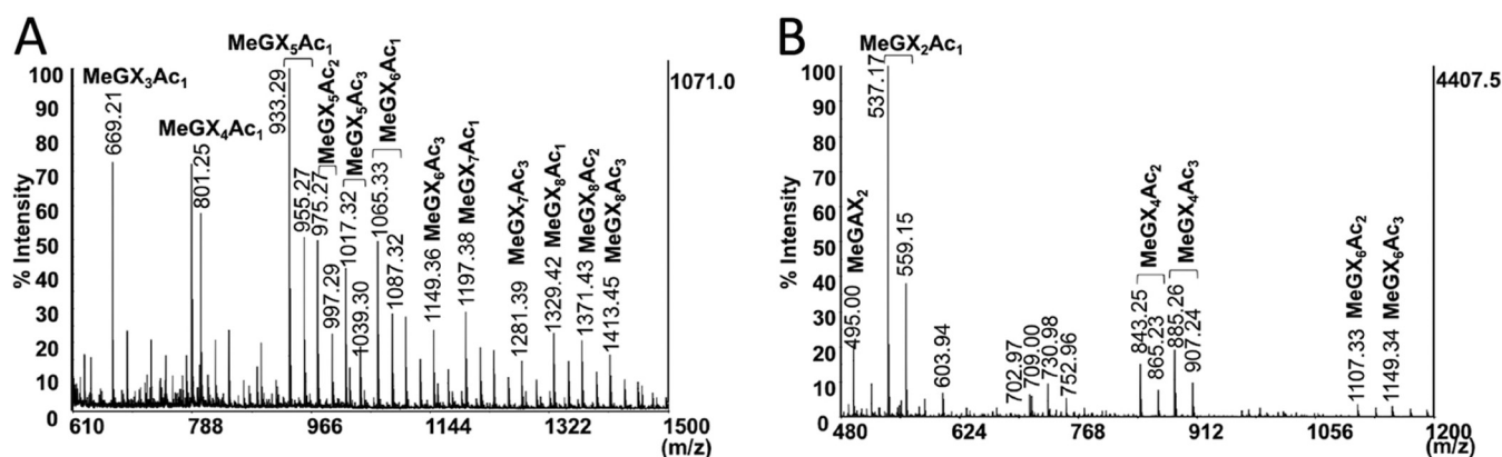
FIG 4 MALDI-TOF mass spectra of hydrolysis products of acetylated xylan. (A) Acetylated glucuronoxylan hydrolysate of StXyn30A. (B) Acetylated glucuronoxylan hydrolysate of StXyn30A and GH3 \beta -xylosidase. Acetylxylan (0.5% [wt/vol]) was incubated with StXyn30A in 50 mM acetate buffer (pH 6.0) containing 0.1% (wt/vol) BSA at 37°C for 20 h. GH3 \beta -xylosidase was then added to the reaction mixture, and the mixture was incubated at 37°C for 2 days.
