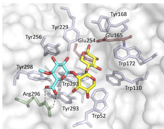
FIG 5 Model of the active site of StXyn30A with MeGX 2 . Blue, 4-O-methyl-glucuronic acid; yellow, xylose; transparent red, Glu165 and Glu254, catalytic residues. Trp52, Trp110, Tyr168, Trp172, Tyr229, Tyr256, Trp292, Tyr293, Arg296, and Tyr298 are conserved in bacterial GH30 enzymes. Two dashed lines indicate the salt bridge between the Arg296 side chain and 4-O-methyl-glucuronic acid of MeGX 2 . The homology model structure of StXyn30A with the substrate was modeled on the basis of the crystal structure of XynC from B. subtilis (9) (PDB accession number 3KL5) using the software Modeller ( https://salilab.org/modeller/ ) (36).
