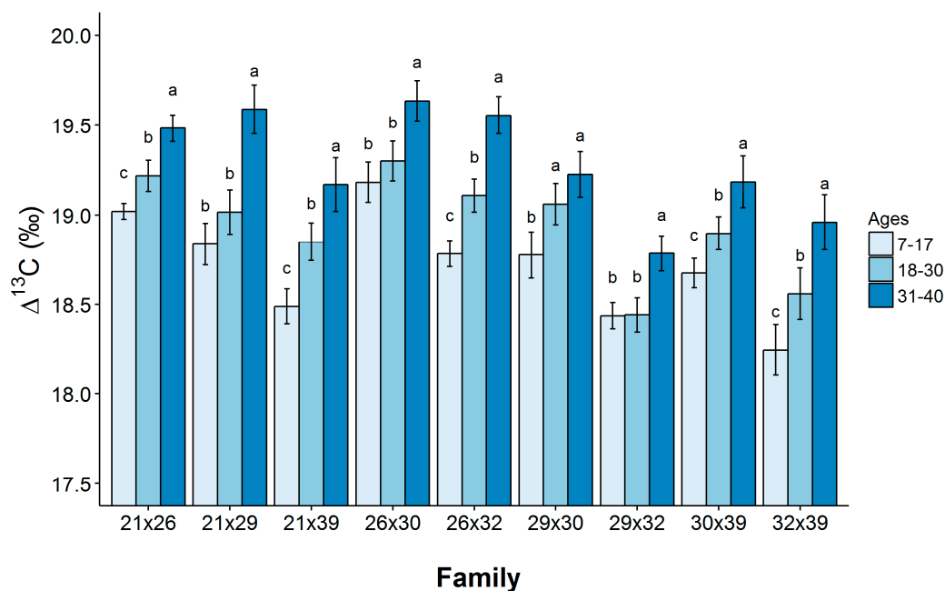
Figure 5. Mean \Delta^{13}\text{C} (‰) values tend to increase from early to late growth stages within families. Means with the same letter within each family are not significantly different from each other as indicated by Tukey HSD post-hoc test ( \alpha = 0.05 ).
