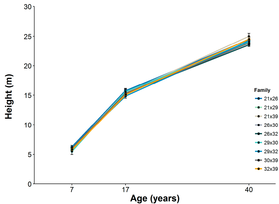
Figure 2. Family mean height at ages 7, 17 and 40. Vertical lines for each data point represent the standard error of the mean.
