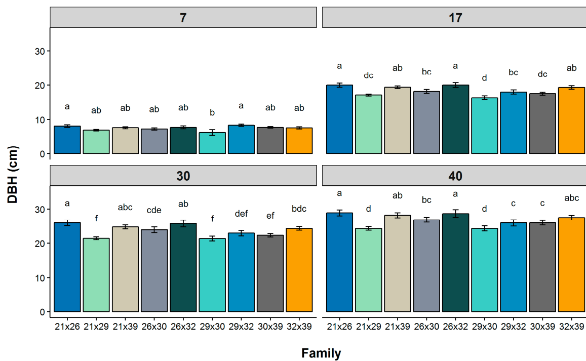
Figure 3. Family mean DBH values for all families at ages 7, 17, 30 and 40. Lines on each bar represent the standard error of the mean. Families with the same letter within a time period are not significantly different from each other as indicated by Tukey HSD post-hoc test ( \alpha = 0.05 ).
