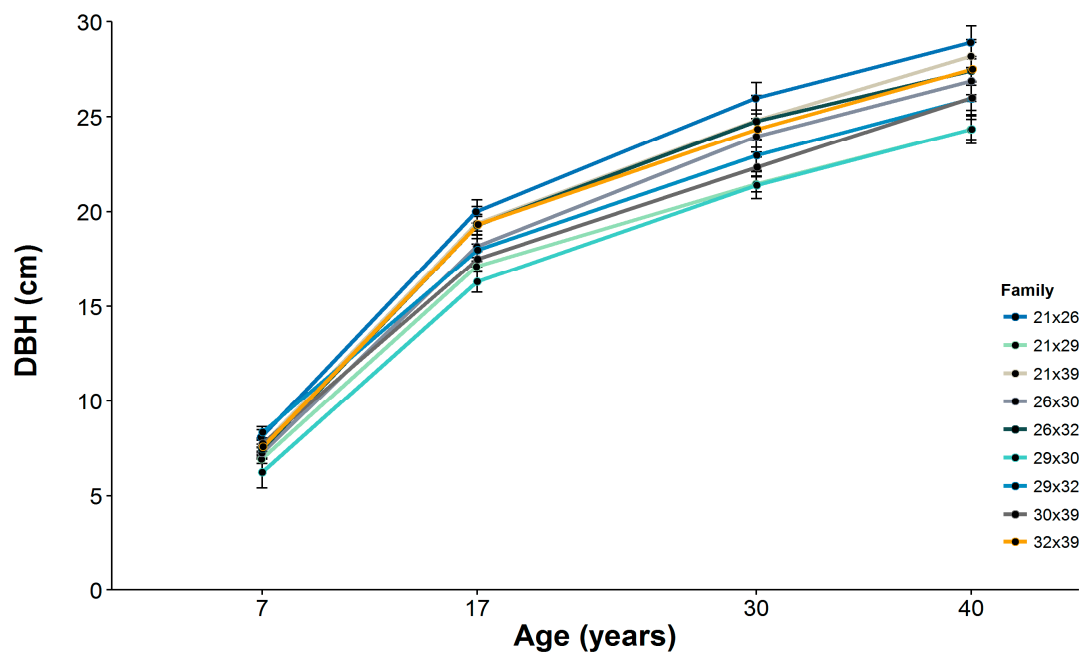
Figure 1. Family mean diameter at breast height (DBH) at ages 7, 17, 30 and 40. Vertical lines for each data point represent the standard error of the mean.
