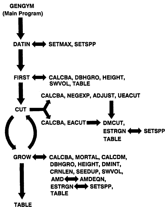
Figure 7.—Flow diagram of GENGYM execution.
