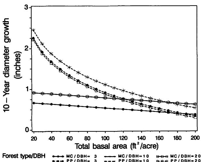
Figure 3.—Comparison of predictions of 10-year periodic d.b.h. growth for ponderosa pine in the mixed conifer (MC) and ponderosa pine (PP) types at site index 70, assuming the diameter class is at the midpoint of the basal area distribution.
