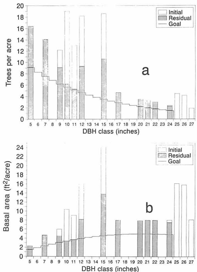
Figure 8.—Example of uneven-aged cutting in an irregular stand to a residual basal area of 80 square feet per acre, a q-ratio of 1.1, and a regulated diameter range of 5 to 24 inches, demonstrating how subroutines UEACUT, NEGEXP, and ADJUST balance deficits in stocking below the goal line by retaining surplus trees in adjacent diameter classes: a, in terms of trees per acre; b, in terms of basal area per acre.
