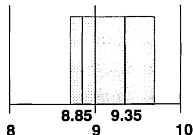
Figure 9.—Diagram of movement of a diameter class after growth projection and subsequent partitioning into two classes at the diameter class break in subroutine GROW.
