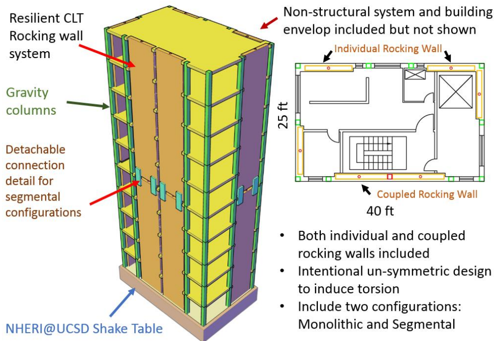
Figure 4. Concept of the 10-story full scale test at NHERI@UCSD facility
