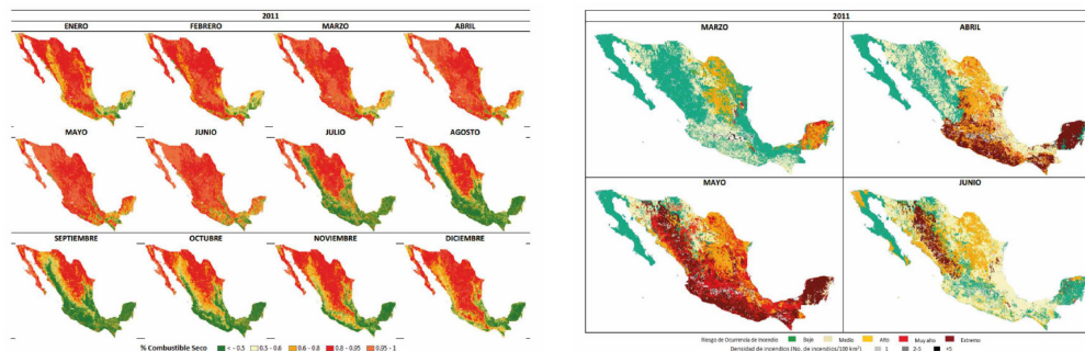
Figure 3. Examples of Fuel Dryness Index (left figure, monthly fuel dryness for 2011) and Fire Occurrence Risk maps (right figure, march to june 2011). Animations of fuel dryness and fire risk for historic years in Mexico can be consulted at the link:
