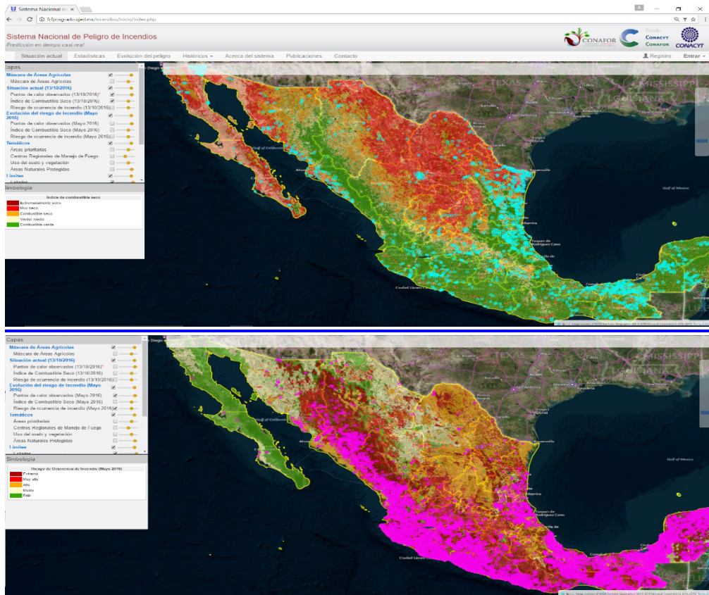
Figure 2. Online interface of the Mexican Forest Fire Danger System: current situation. Top figure shows current fuel dryness index and observed fire hotspots (in blue) in October 2016. Colors represent fuel dryness, with green being very wet fuel and red and light pink being dry and very dry fuel conditions. Bottom figure shows the predicted fire occurrence risk map and observed fire hotspots (in bright pink) in May 2016. Colors represent risk of fire occurrence, with green meaning low probability of fire occurrence and red and dark red representing high and very high fire occurrence risk. http://fcfposgrado.ujed.mx/incendios/inicio/index.php
