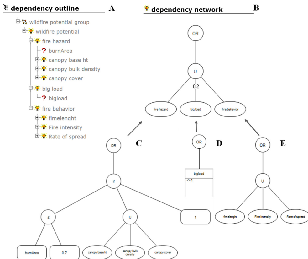
Fig. 3. NetWeaver logic model for fire potential. A, simple outline view of model structure; and the logic specifications for B, fire potential; C, fire hazard; D, big load; and E, fire behavior. Complete documentation for the fire potential model (Fig. 3) is provided in HTML in the supplementary material accompanying this paper.
