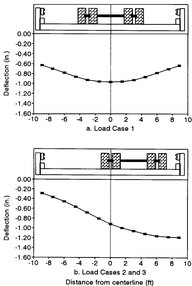
Figure 17—Theoretical maximum deflection under HS 20-44 load.
