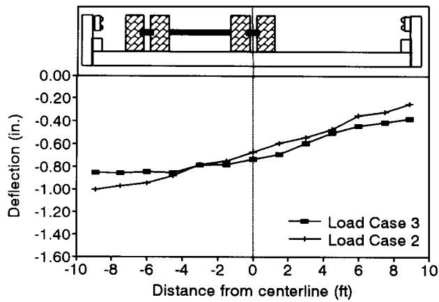
Figure 15—Comparison of load cases 2 and 3.
