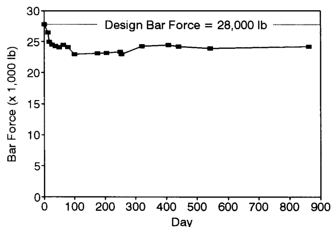
Figure 13—Average bar tension force obtained from load cells installed on two stressing bars.
