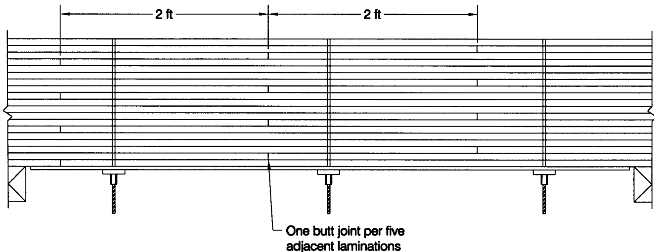
Figure 3—Butt-joint configuration used for the Connell Lake bridge. A butt joint was placed transverse to the bridge span in every fifth lamination. Longitudinally, butt joints in adjacent laminations were separated by 2 ft.
