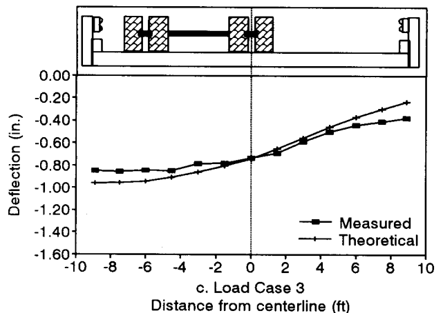
Figure 16—Theoretical deflection compared with measured deflection under the actual applied load using an orthotropic plate analysis.
