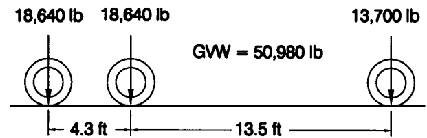
Figure 10—Load test vehicle configuration and axle loads.
