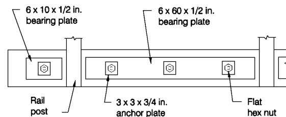
Figure 4—Details of the continuous bearing plate bar anchorage system.
