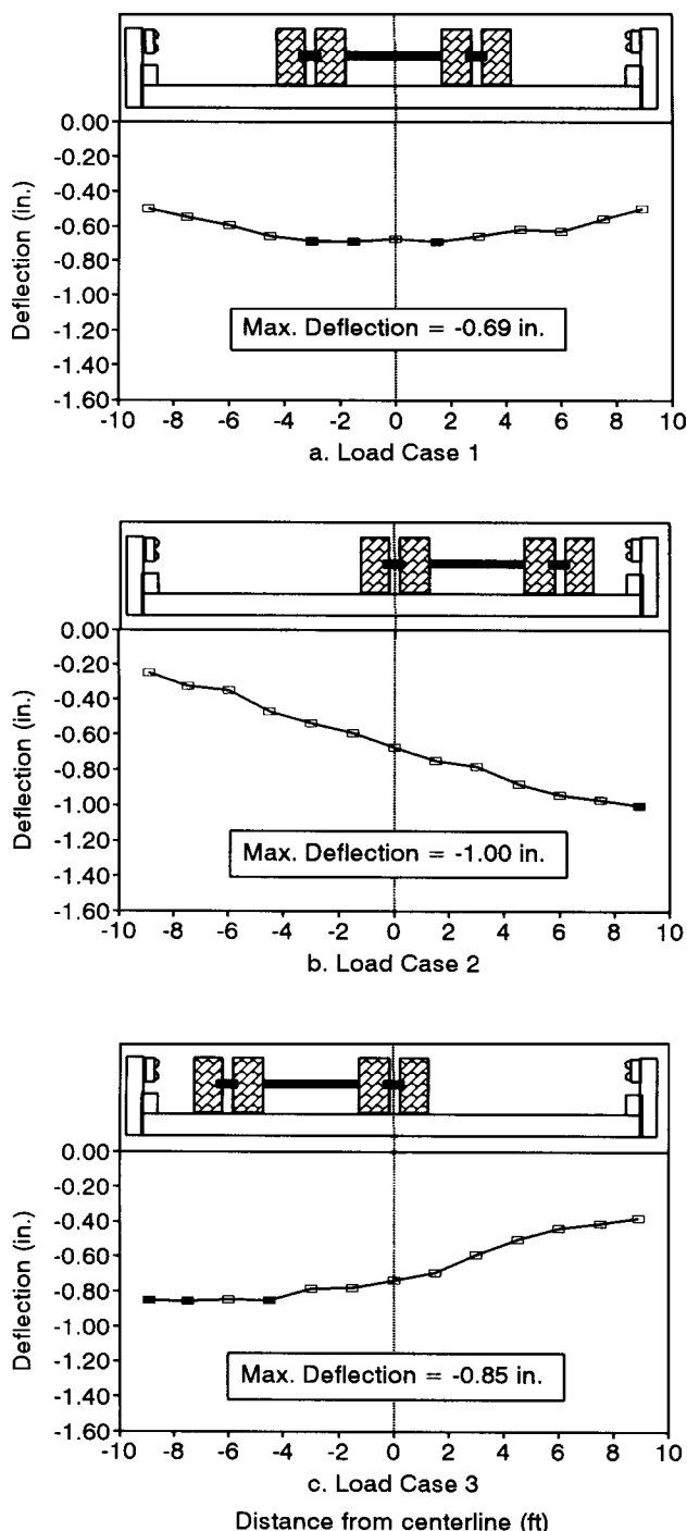
Figure 14—Transverse deflection for load test, measured at midspan. Bridge cross sections and vehicle positions are shown to aid interpretation and are not to scale.
