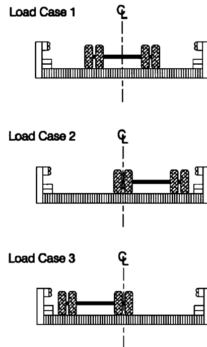
Figure 11—Transverse vehicle load cases as viewed from the east, looking west. For all load cases, the vehicle was facing east with the longitudinal vehicle centroid placed over the bridge midspan. The transverse vehicle track width was 6 ft, measured center-center of the rear tires.
