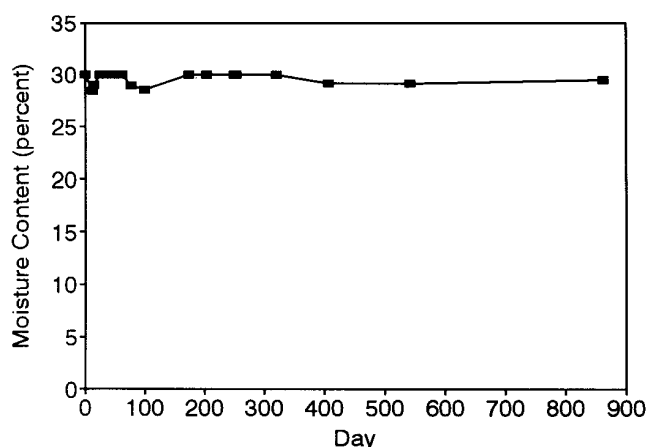
Figure 12—Average moisture content changes in the deck of the bridge.
