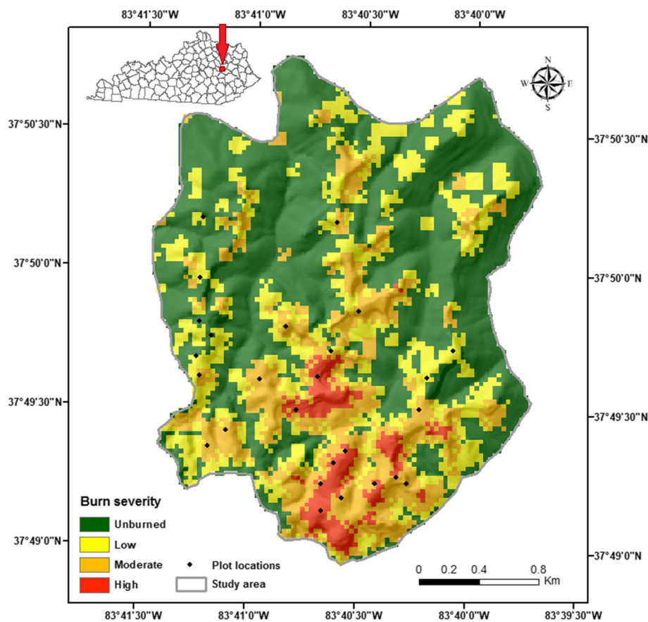
Fig. 1 Map of 26 study plots arrayed across the Fish Trap Fire site, which is characterized by fire severity, in the Daniel Boone National Forest, Kentucky, USA. dNBR, based on NDVI values, was used to create this map in Arc GIS (Upadhyaya 2015). Categories correspond to CBI as follows: unburned: 0, low: 0.1 to 1, moderate: 1 to 2, high: 2 to 3.
