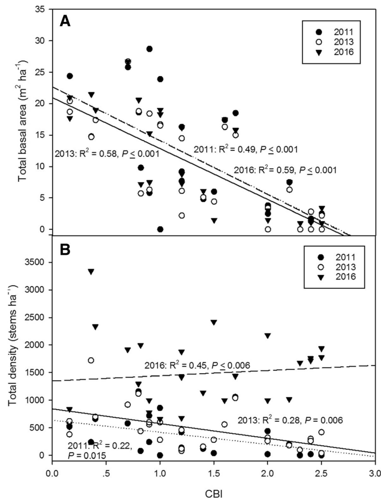
Fig. 2 Relationship between CBI, as a proxy for fire severity, and (a) total basal area (all stems \geq 2 cm DBH, \text{m}^2 \text{ha}^{-1} ), and (b) stem density (all stems \geq 2 cm DBH, stems \text{ha}^{-1} ) in years one (2011), three (2013), and six (2016), following a 2010 wildfire on the Cumberland Plateau, Kentucky, USA.
