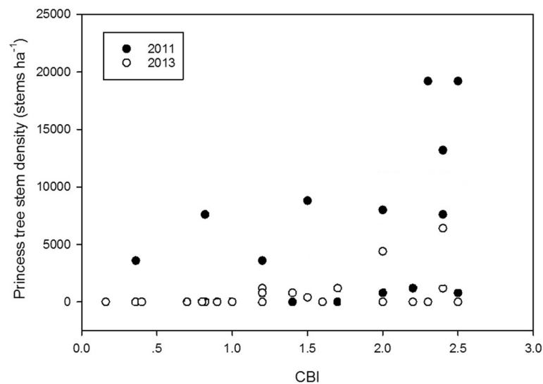
Fig. 6 Density of princess tree <2 cm DBH (stems \text{ha}^{-1} ) across a gradient of fire severity in years one and three (2011 and 2013) after a 2010 wildfire on the Cumberland Plateau, Kentucky, USA.
