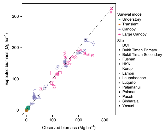
Fig. 6 | Observed versus predicted biomass. Observed biomass by survival mode versus predicted biomass from an individual based model at each site (marginal R^2 = 0.9735 ). The line between points traces census interval typically diverging from the broken line, which represents the 1:1 line, with time.
