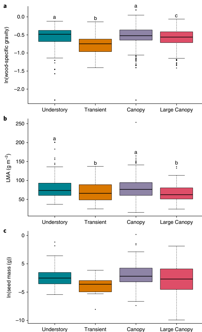
Fig. 4 | In general, traits do not map strongly onto the four survival modes. a , Natural log-transformed wood-specific gravity at all sites. b , LMA at six sites (Lambir, BCI, Luquillo, Laupahoe, Palamanui and Fushan). c , Natural log-transformed seed mass and survival modes at Luquillo, Laupahoe, Palamanui and BCI where there were no significant differences between survival modes. Whiskers on boxes indicate the range of the data out to 1.5 times the length of the box. Letters represent significant differences among survival modes in traits at \alpha = 0.05 by Tukey HSD test.
