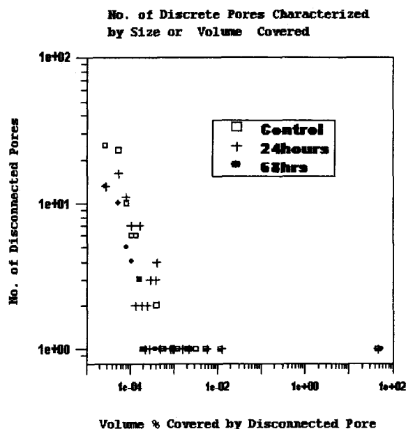
Figure 5. Disconnectivity Curves
