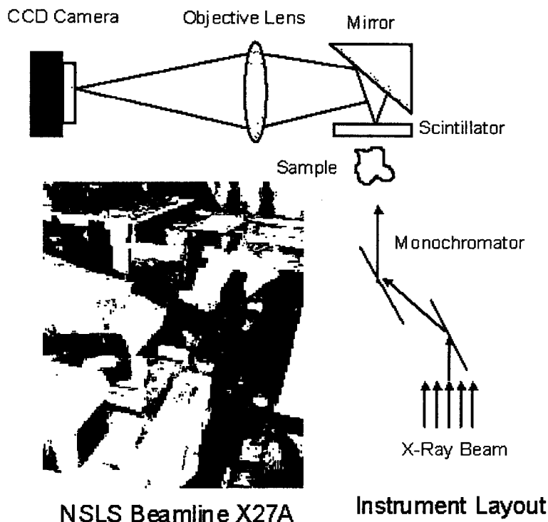
Figure 1. XCMT apparatus
