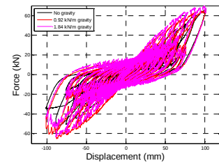
Fig. 7- 1.22mx2.44mx168.9mm specimen tested under different vertical loading
