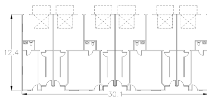
Fig. 13- Index building 1st floor plan for a 3-story multi-family residential building ( dimensions in meters)
