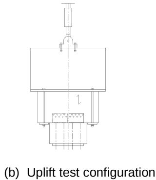
Fig. 1- Test configuration for connector tests
