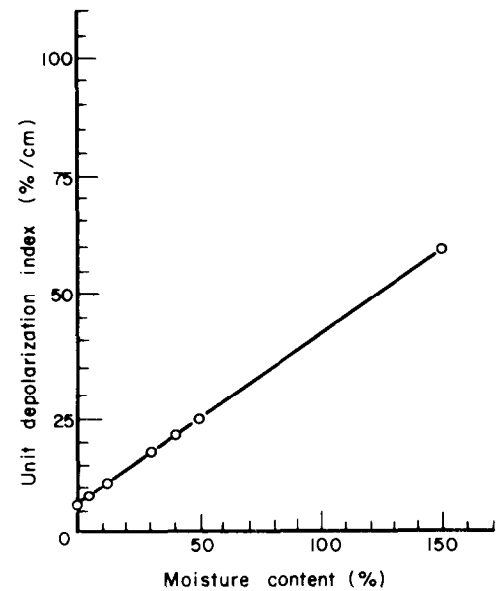
Figure 5.—Depolarization index per centimeter thickness of Douglas-fir as a function of moisture content. (ML84 5832)
