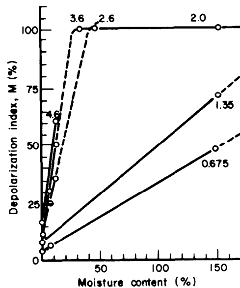
Figure 4.—Depolarization index of Douglas-fir as a function of specimen thickness and moisture content. The numbers at each curly are the corresponding specimen thicknesses in centimeters. (ML84 5829)
