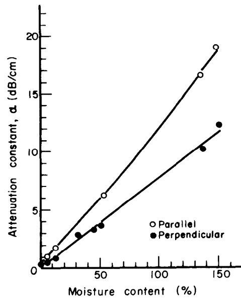
Figure 2.—Attenuation constant of Douglas-fir parallel and perpendicular to the grain as a function of moisture content. (ML84 5827)
