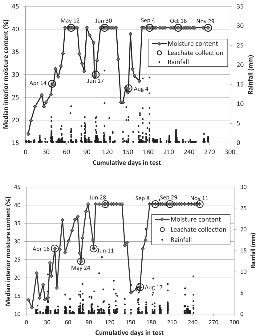
Figure 2. Rainfall and median interior MC for specimens exposed outdoors for year 1 (top) or year 2 (bottom). MC is capped at 40% because of method limitations. Individual markers show rainfall amounts in 15-min intervals.
